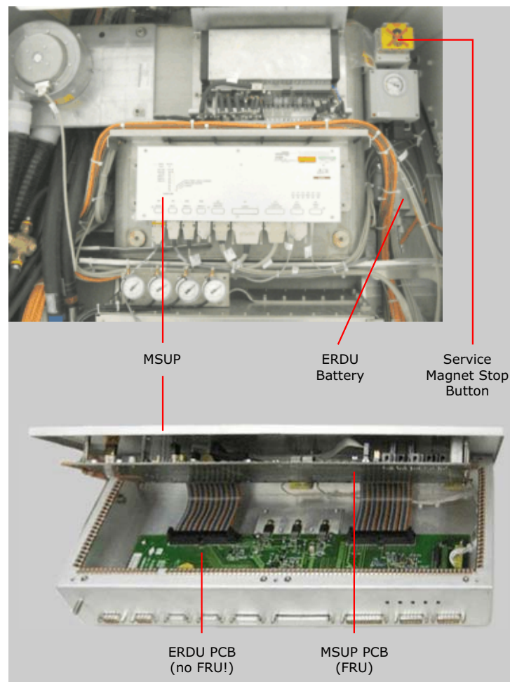
Figure 196 MSUP 2306 Layout
