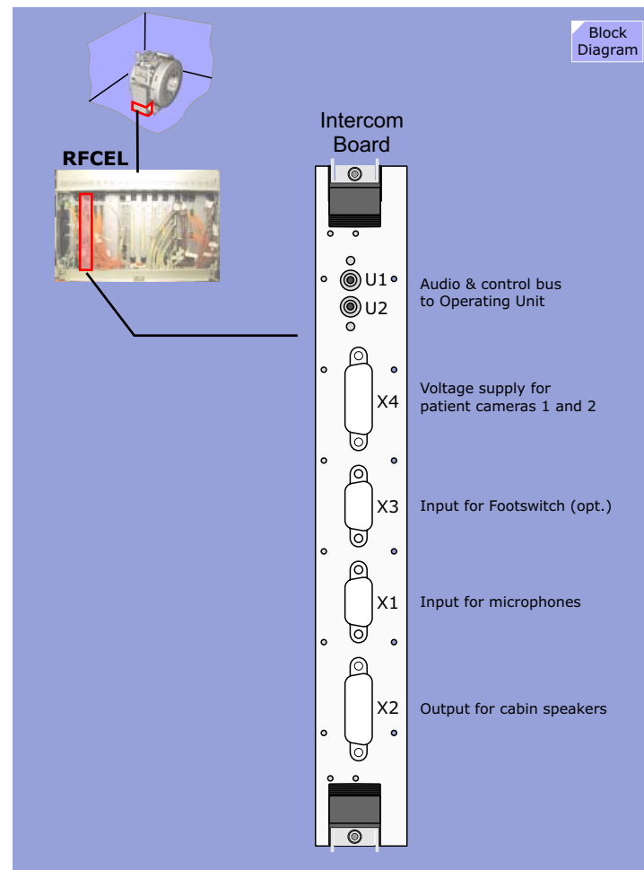
Figure 137 Intercom Board Front View
