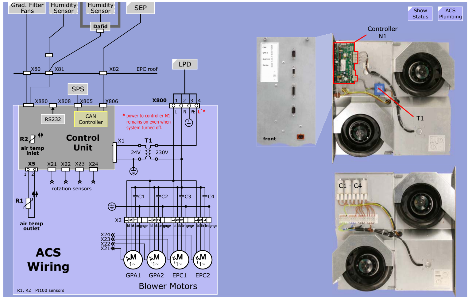
Figure 215 ACS Wiring Diagram
