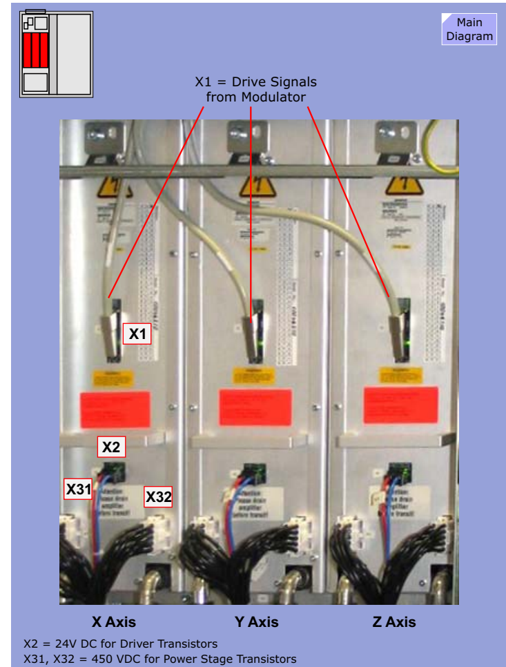
Figure 172 90/22/F Power Stage Layout
