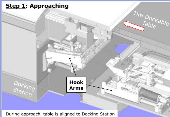
Figure 117 Docking Process
