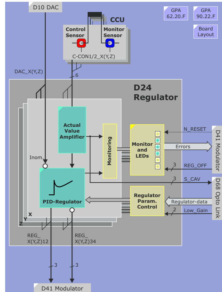
Figure 150 D24 Regulator Block Diagram
