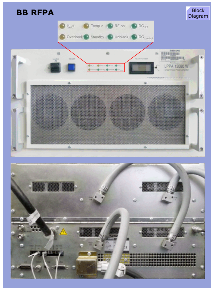
Figure 89 BB RFPA Layout
