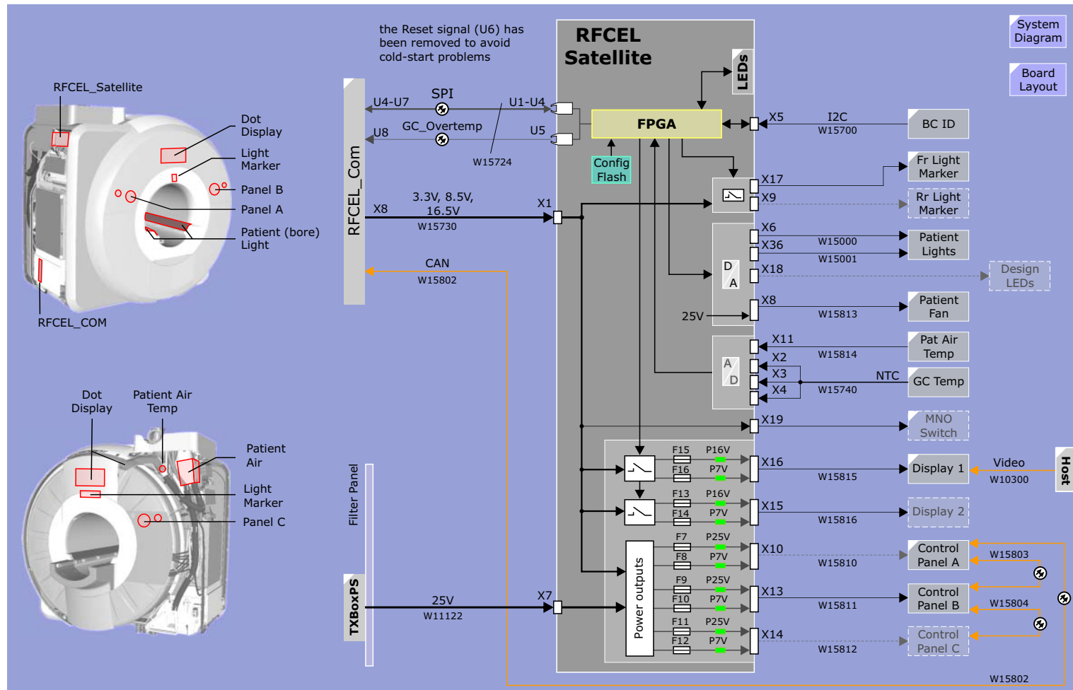
Figure 128 Cabin User Interface Block Diagram
