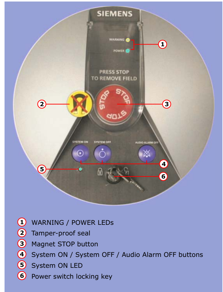
Figure 203 Alarm Box Layout
