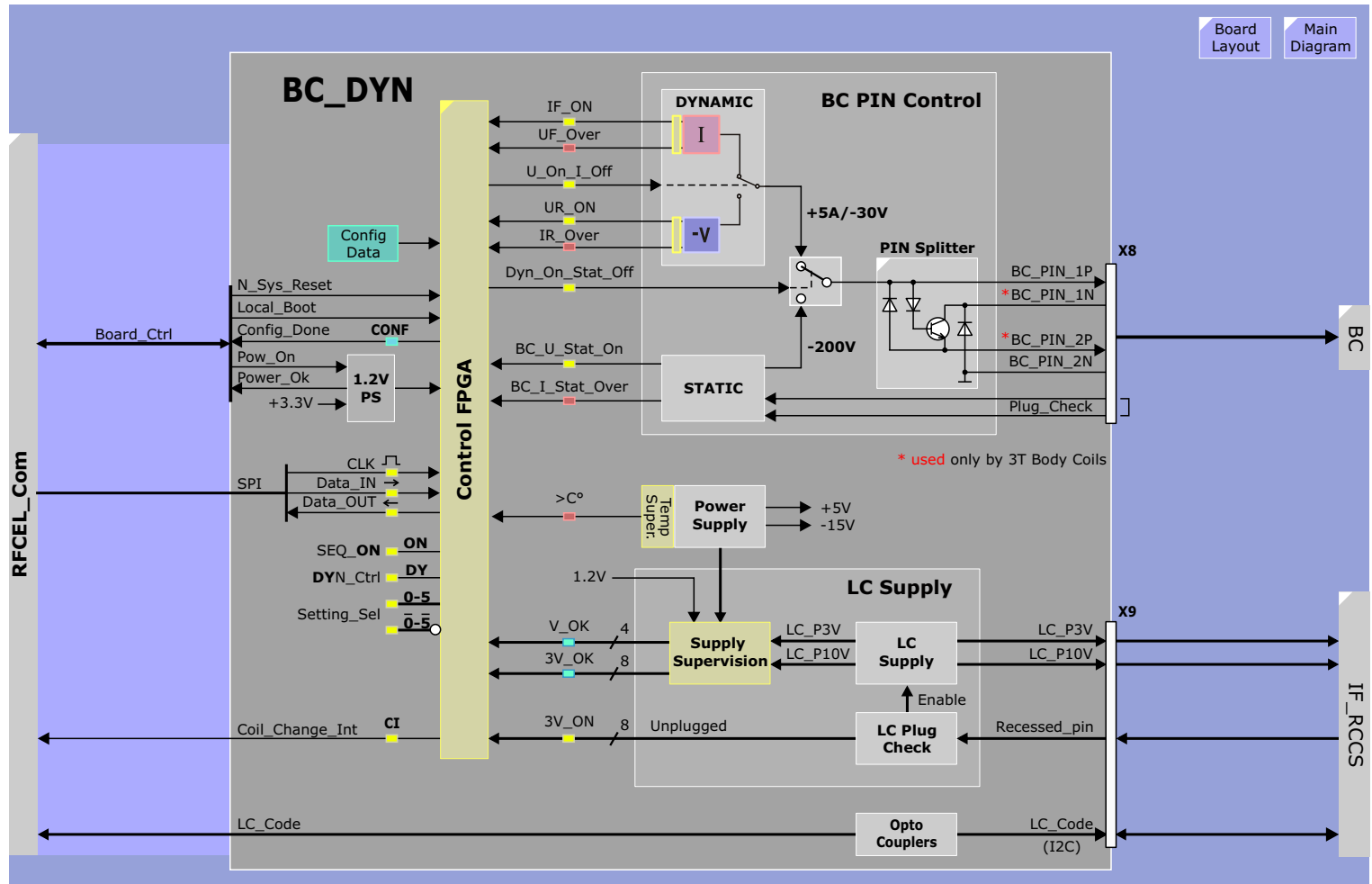
Figure 63 BC_DYN Block Diagram
