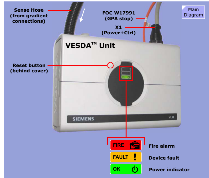
Figure 183 Gradient Supervision SIEMENS_VLM
