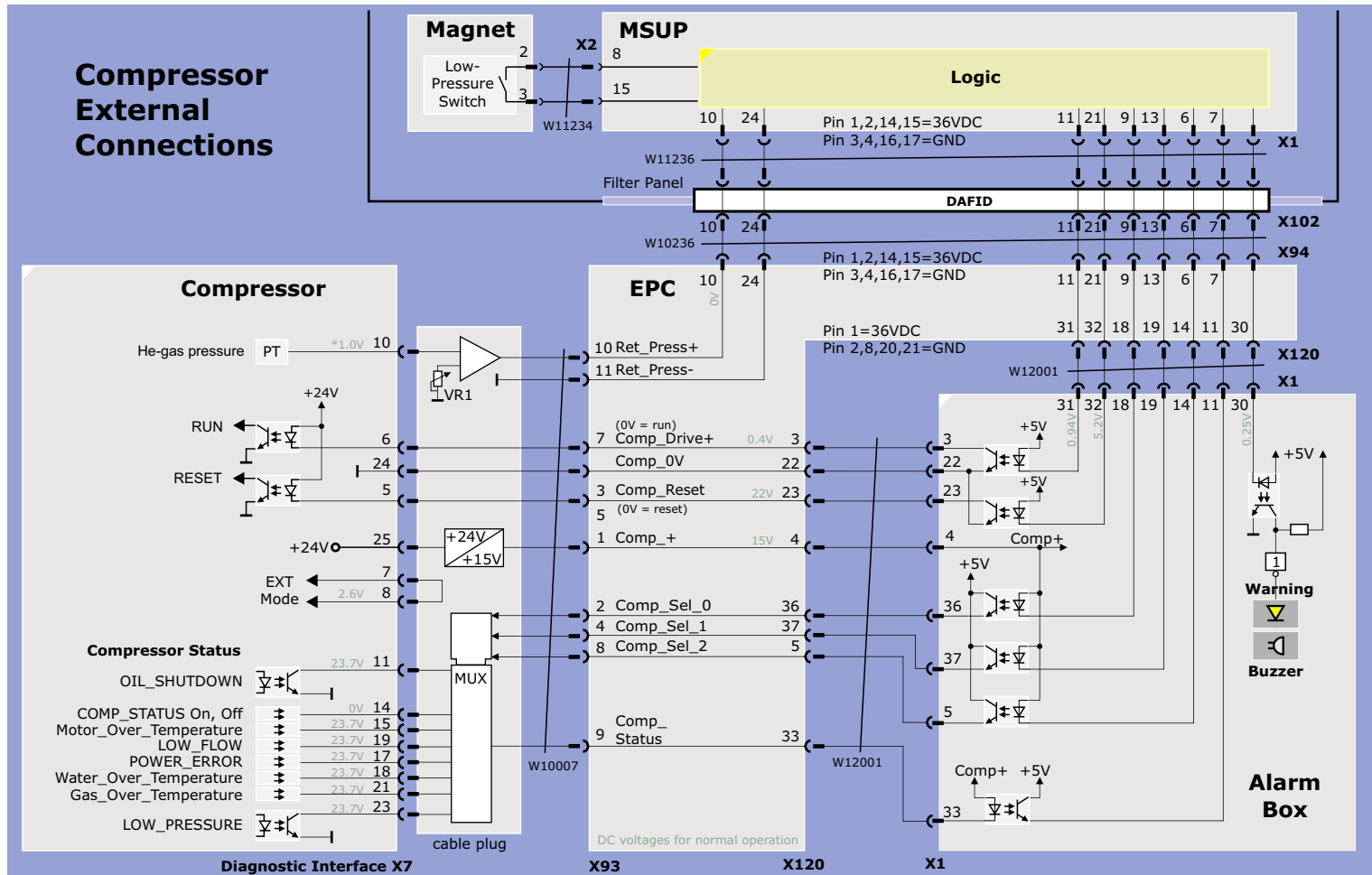
Figure 209 F70 Compressor Control Diagram
