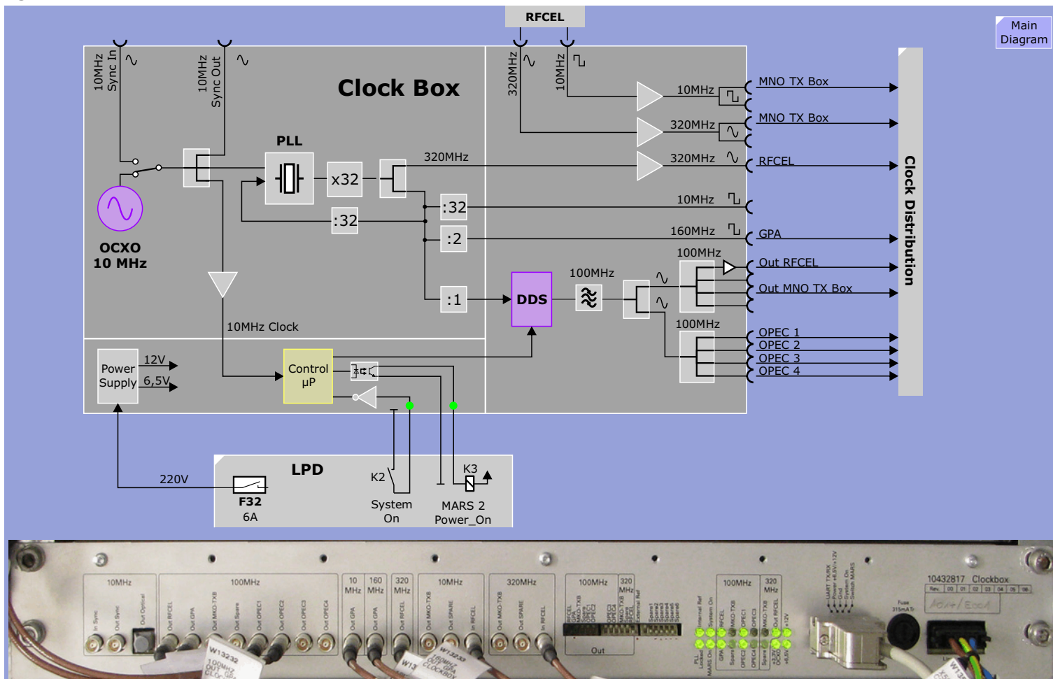
Figure 41 Clock Box
