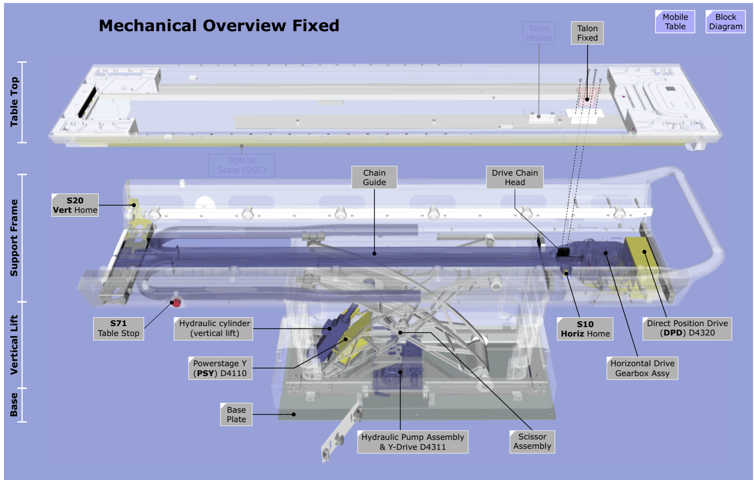
Figure 94 Tim Table Parts Location
