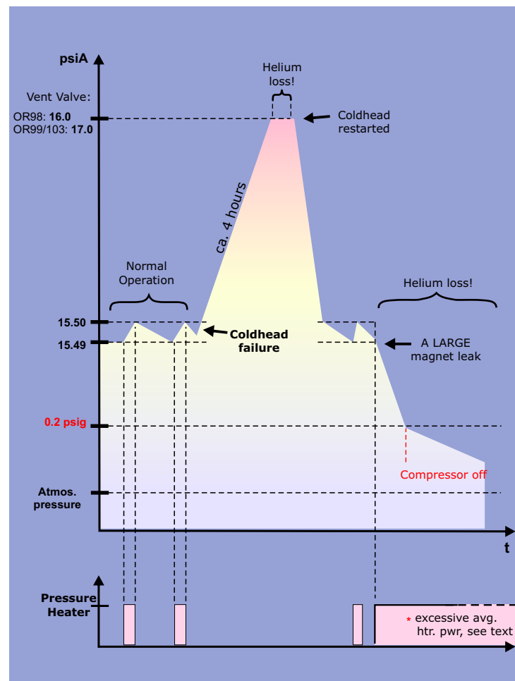
Figure 200 Magnet Pressure Regulation
