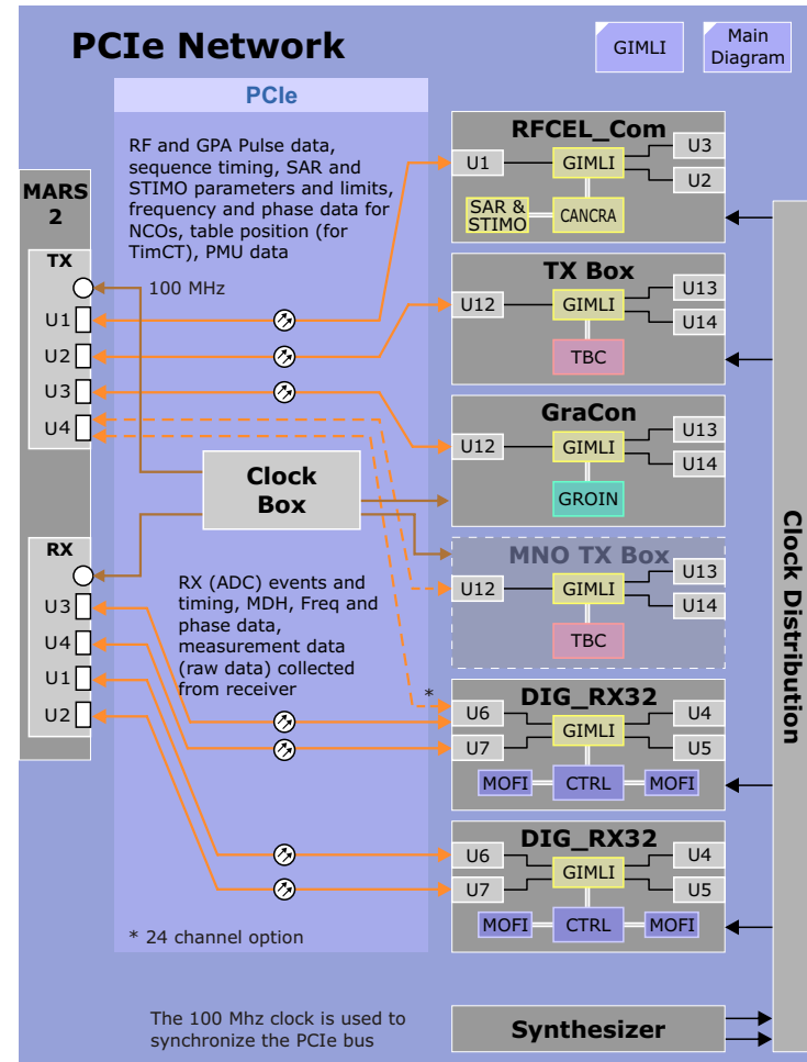
Figure 32 PCIe Network
