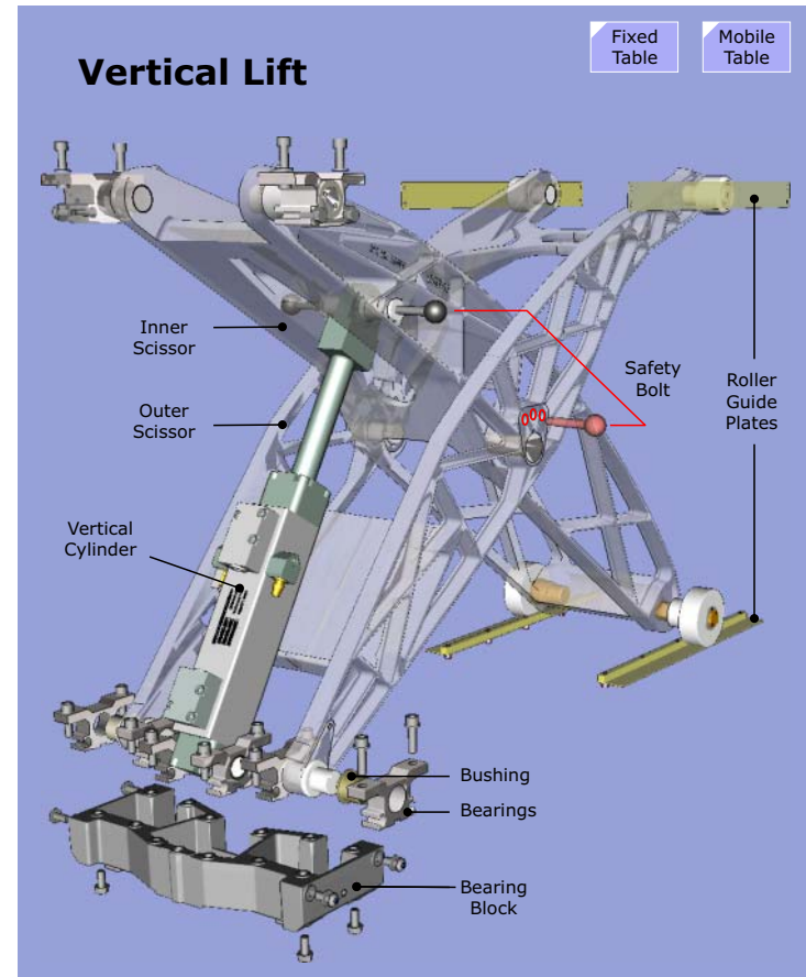
Figure 95 Vertical Lift Mechanics
