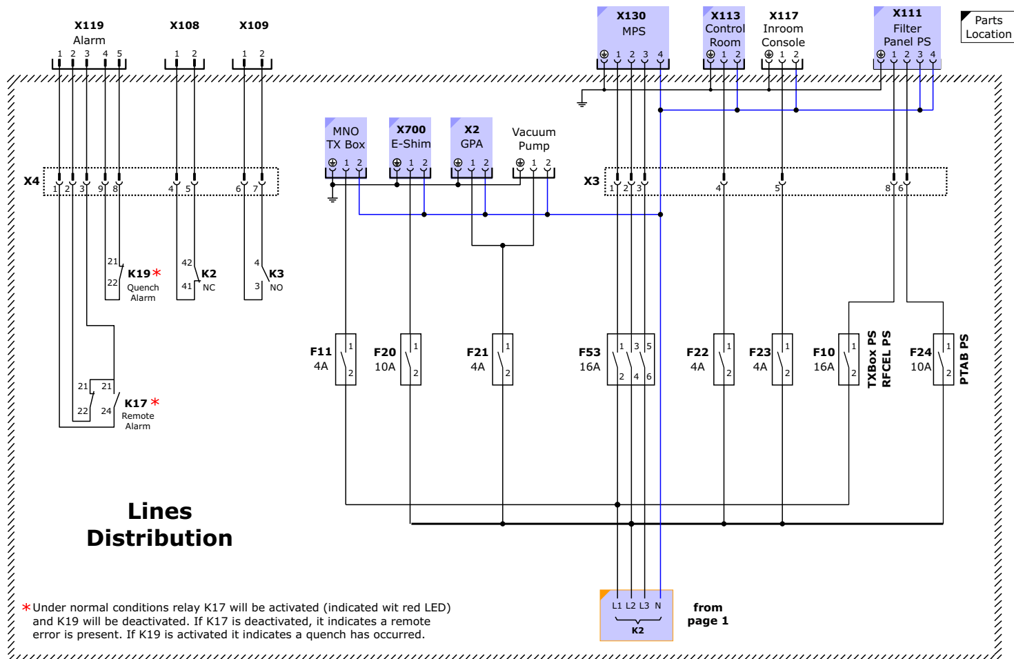
Figure 224 Line Power Distributor Diagram, page 2
