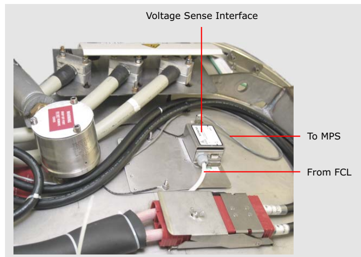
Figure 193 Voltage Sense Interface
