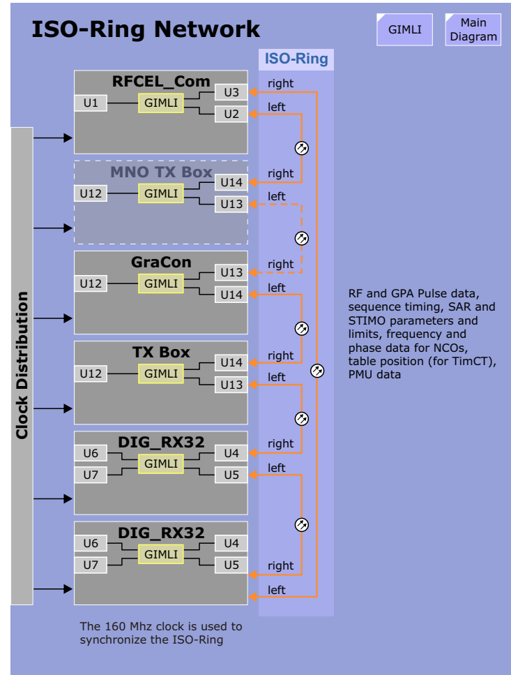
Figure 33 ISO-Ring Network
