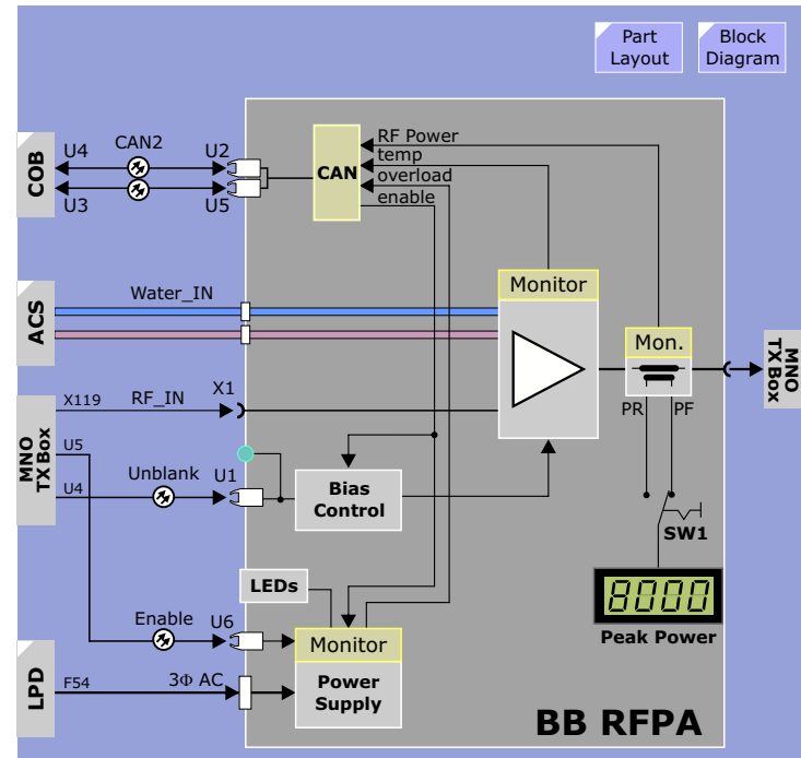
Figure 88 BB RFPA
