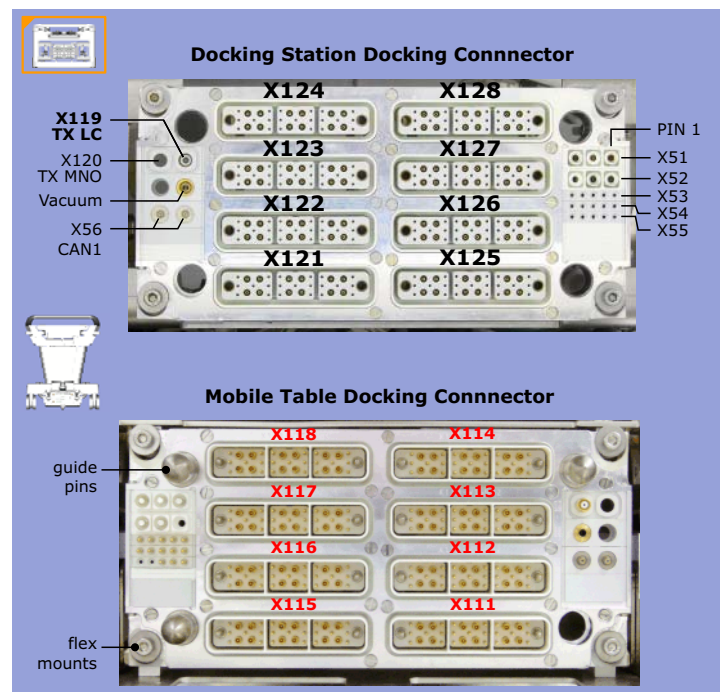
Figure 119 Connector Assemblies
