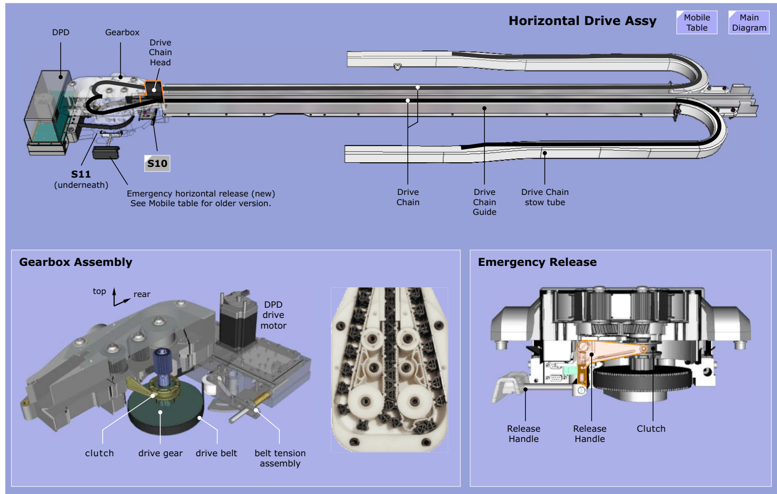
Figure 103 Horizontal Drive System - Fixed Table
