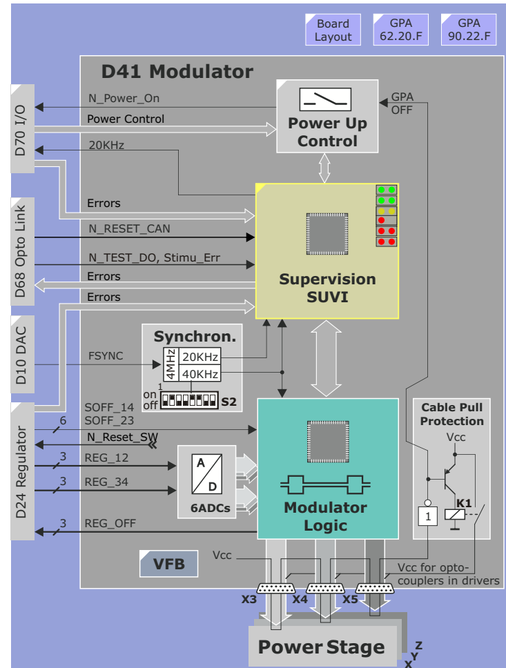
Figure 156 D41 Modulator Block Diagram
