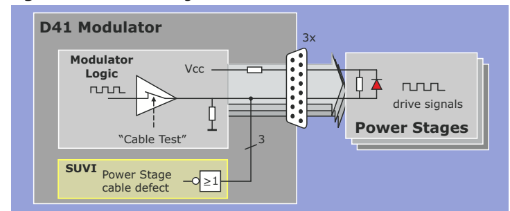
Figure 158 Power Stage Cable Test
