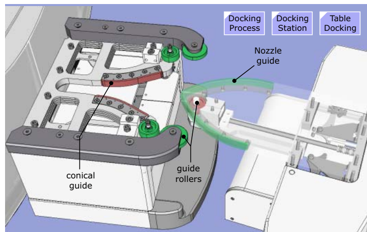
Figure 116 Dock Guidance
