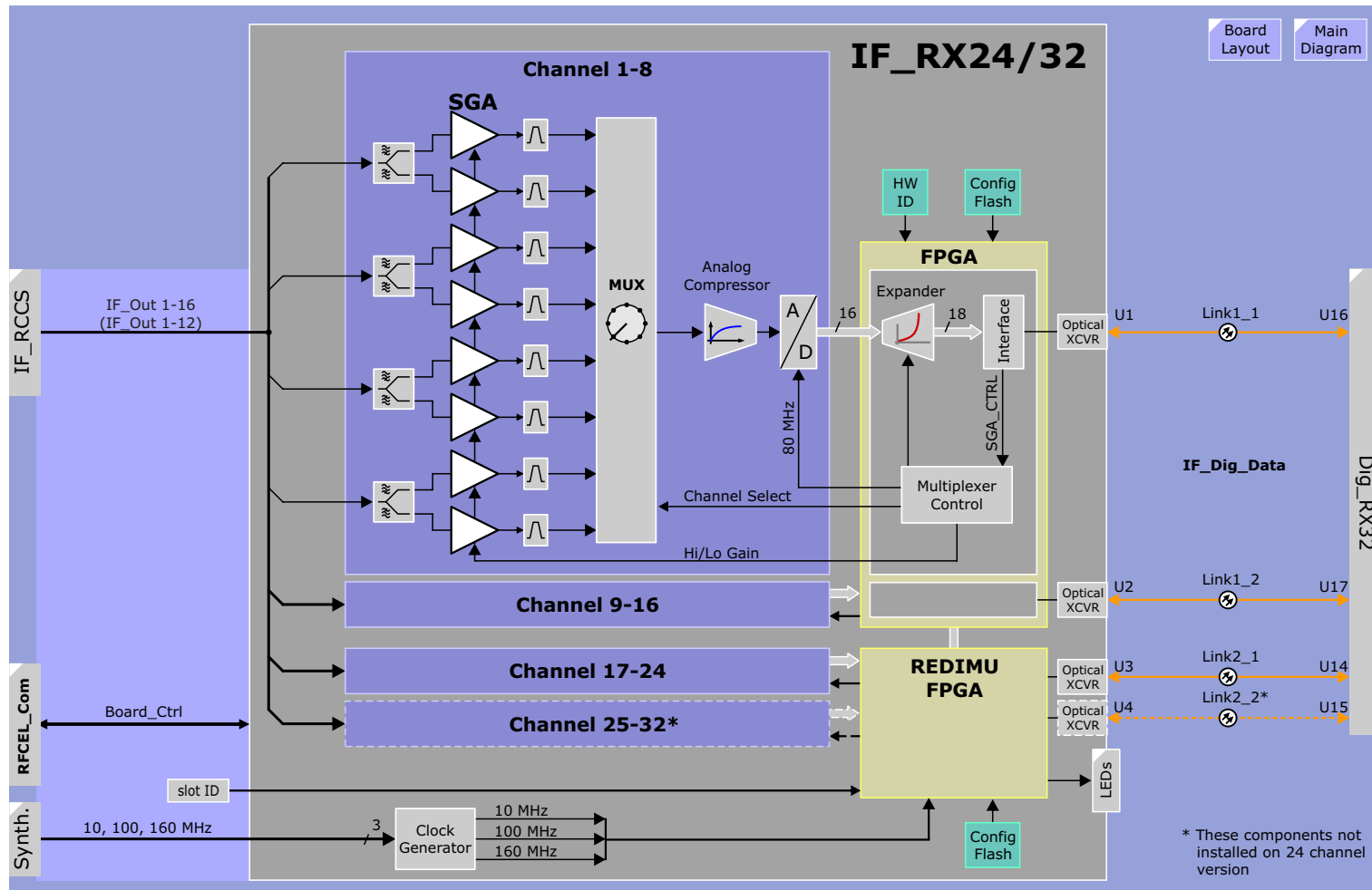
Figure 61 IF_RX32 Block Diagram
