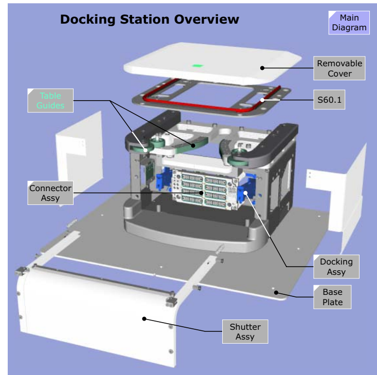
Figure 121 Dock Station
