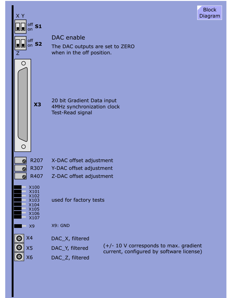
Figure 149 D10 Board Layout
