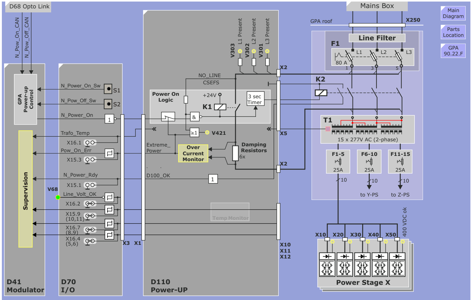
Figure 175 62/20/F Power Stage Supply Block Diagram
