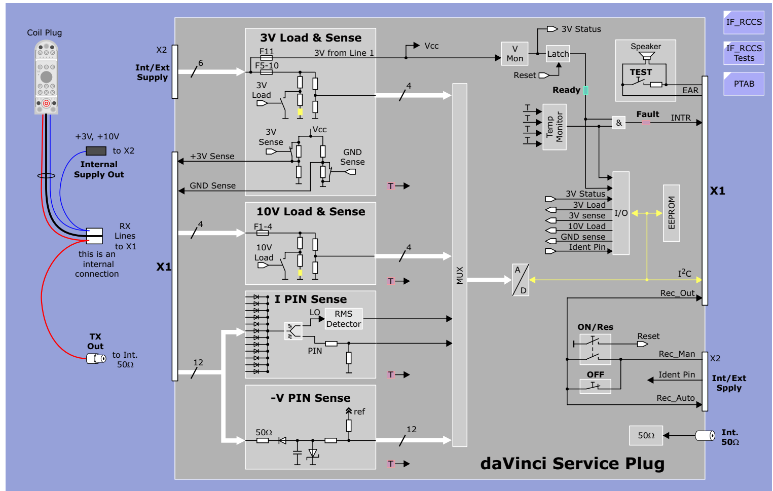
Figure 254 Service Plug Block Diagram
