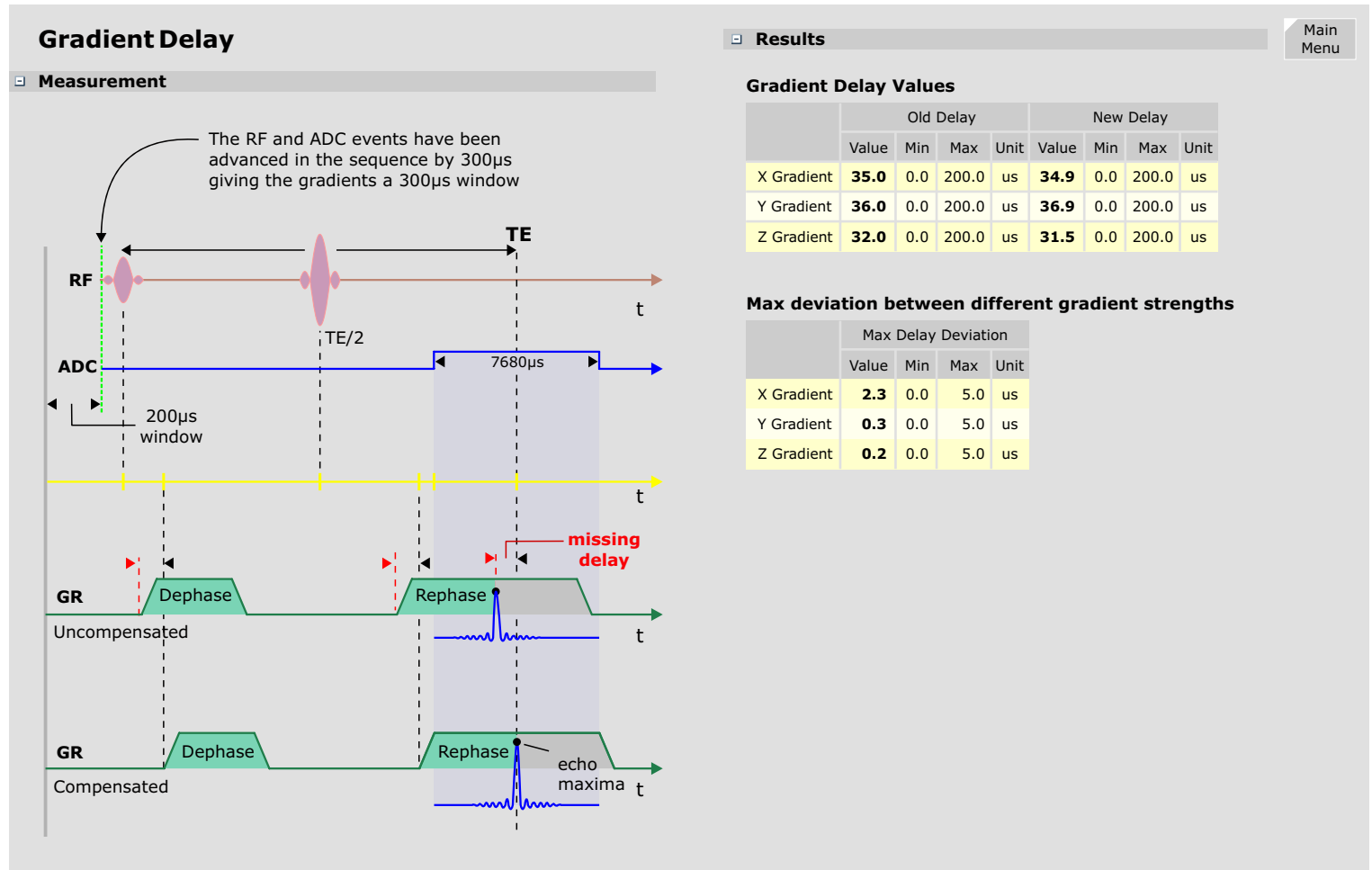
Figure 239 Gradient Delay Measurement and Results
