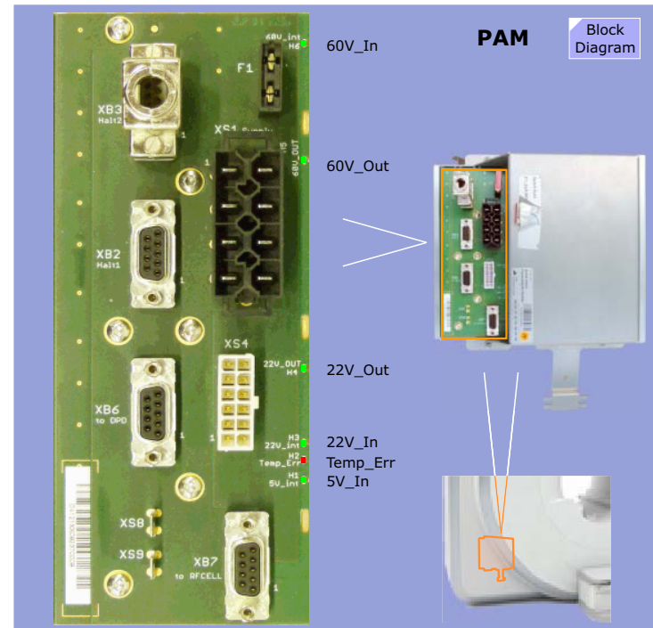
Figure 102 Power Adaptor Module - PAM D4120
