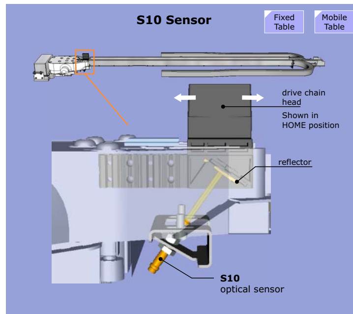
Figure 105 Horizontal HOME Detector S10
