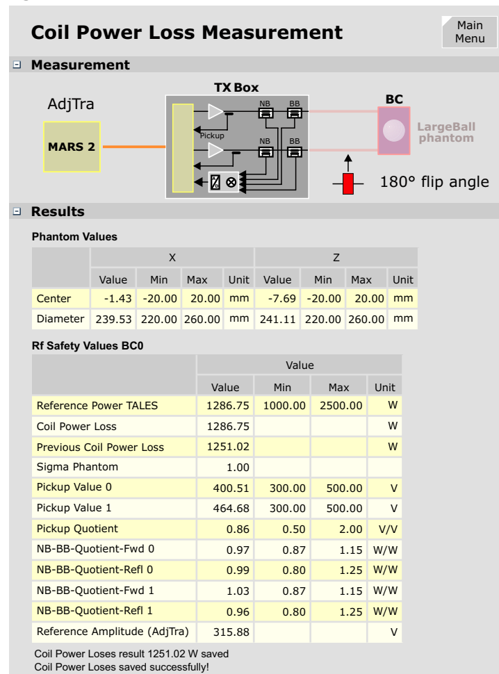
Figure 241 Coil Power Loss Measurement
