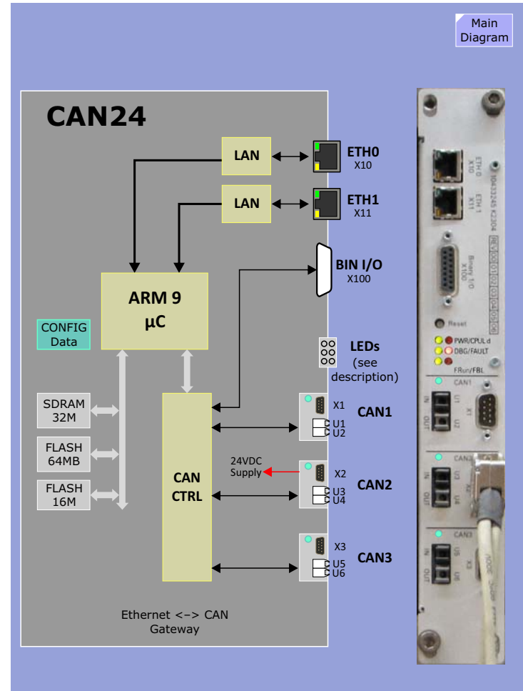
Figure 39 CAN24 Block Diagram
