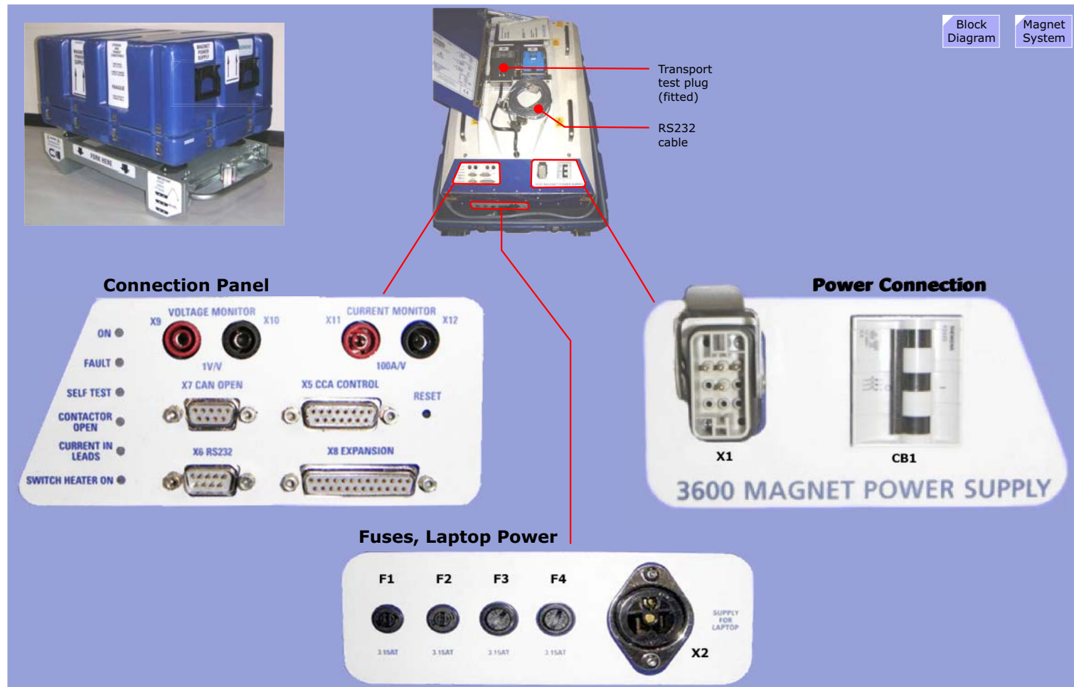
Figure 256 Magnet Power Supply Connections
