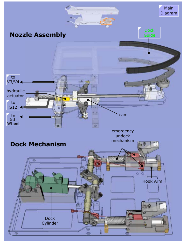
Figure 120 Table Docking Assembly
