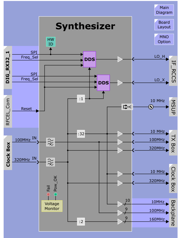
Figure 74 Synthesizer Block Diagram
