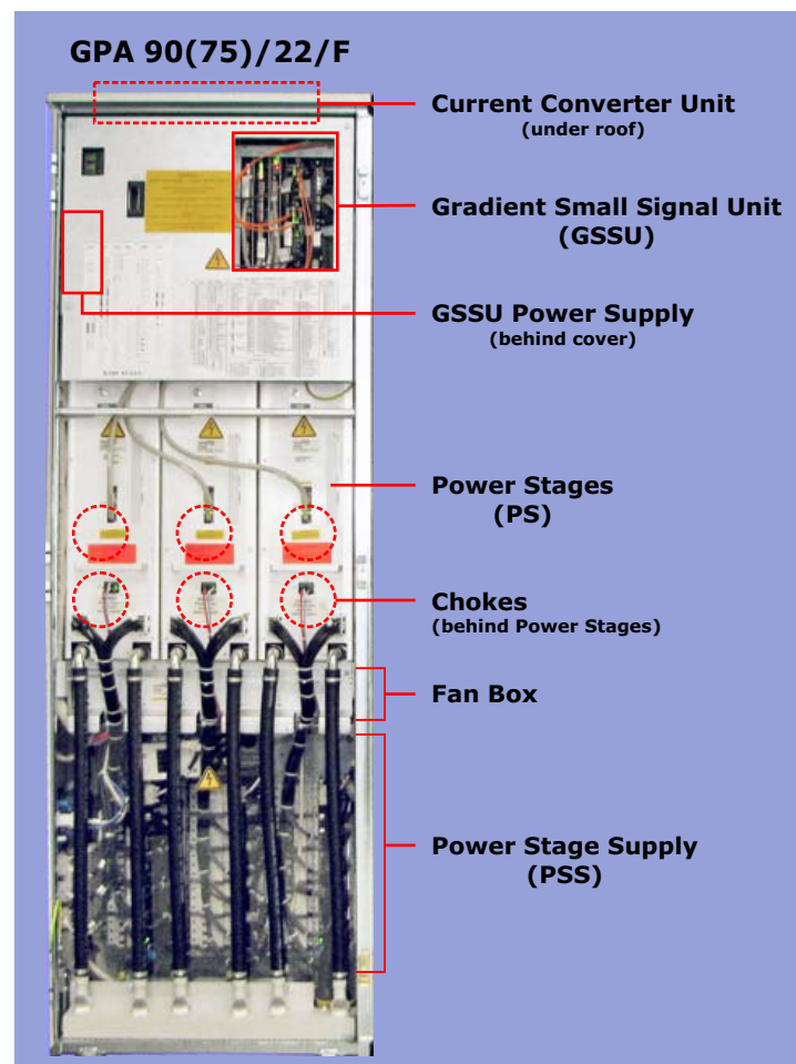
Figure 145 GPA 90(75)/22/F Layout
