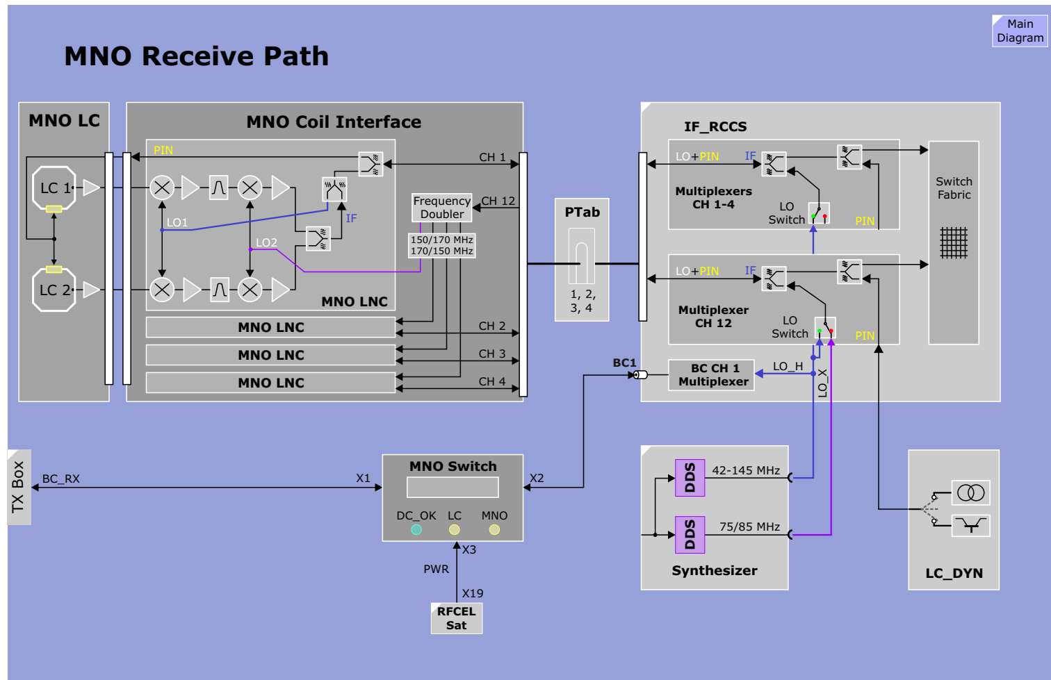
Figure 90 MNO Receive Path
