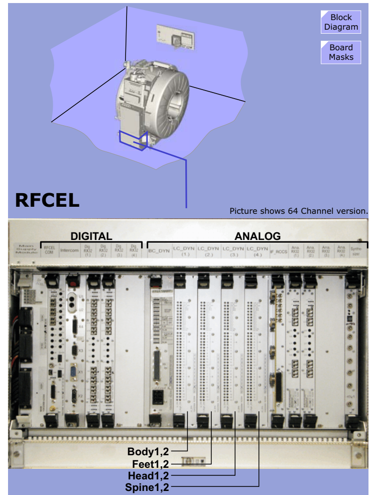
Figure 51 RFCEL Rack Location
