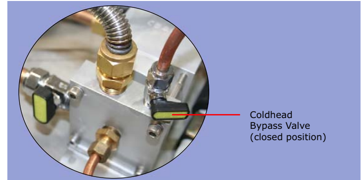
Figure 211 Cold Head bypass valve CLOSED
