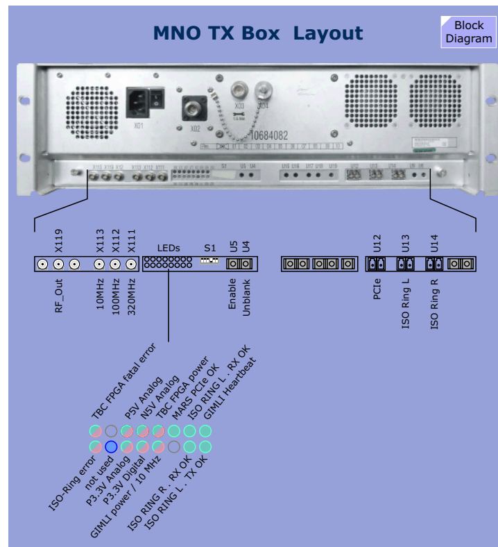
Figure 87 MNO TX Box Layout
