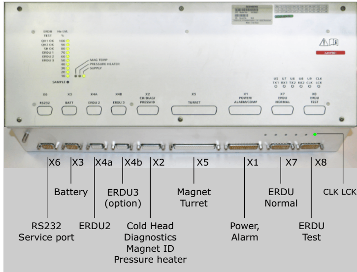
Figure 201 MSUP Connectors
