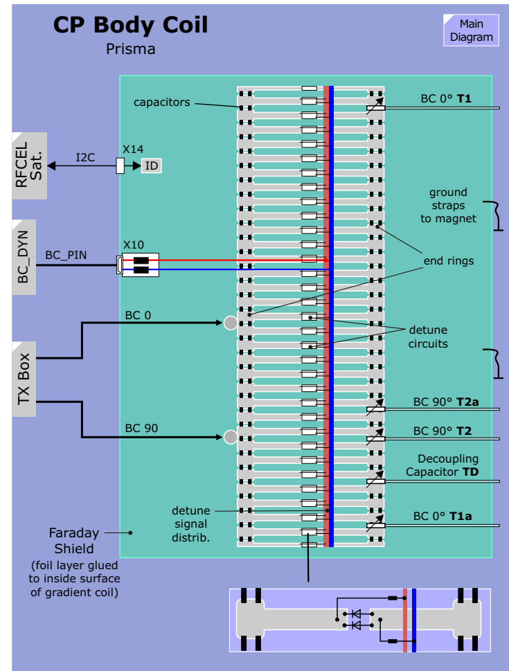
Figure 267 Prisma Body Coil Block Diagram
