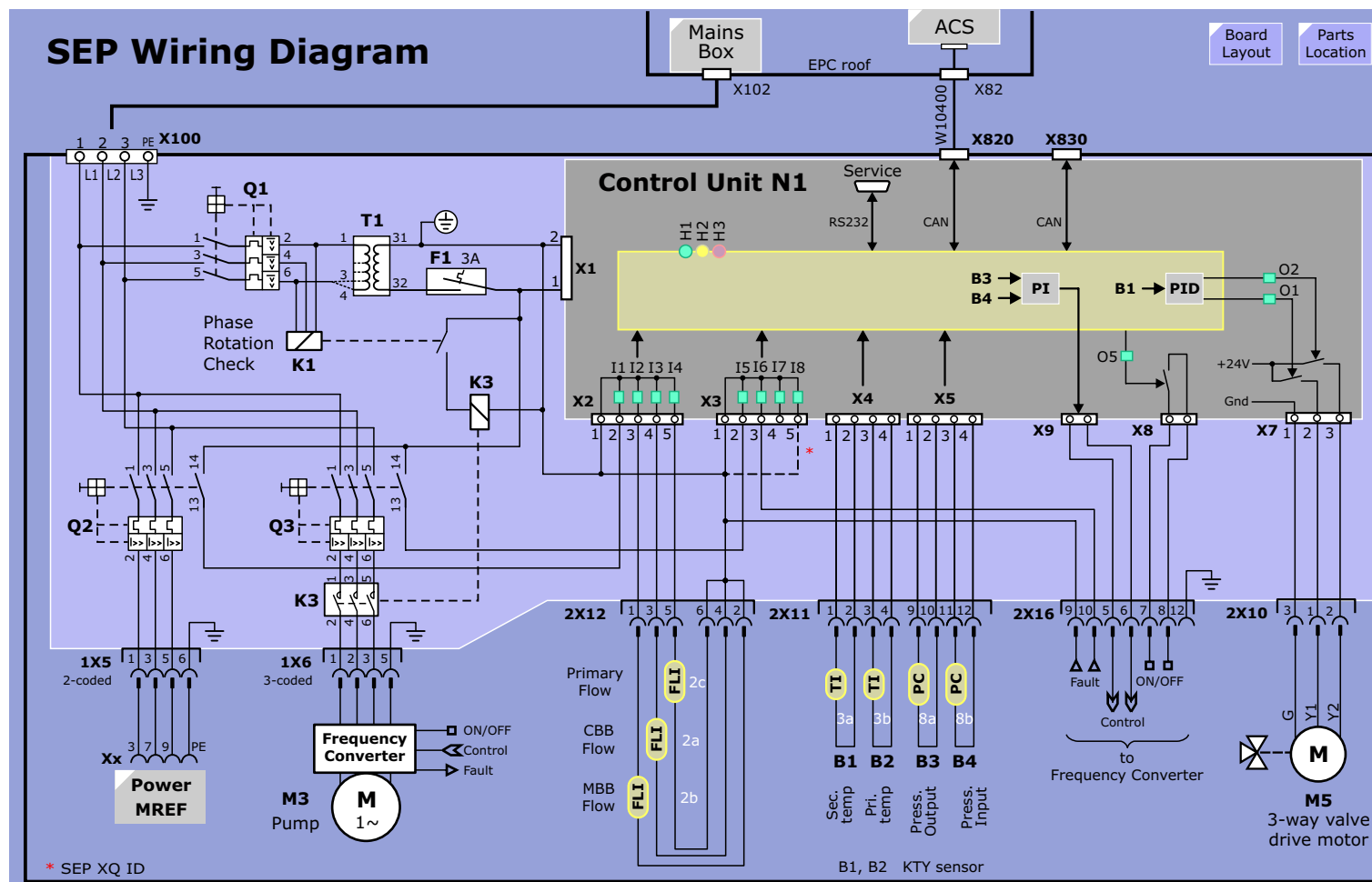
Figure 217 Separator Wiring Diagram
