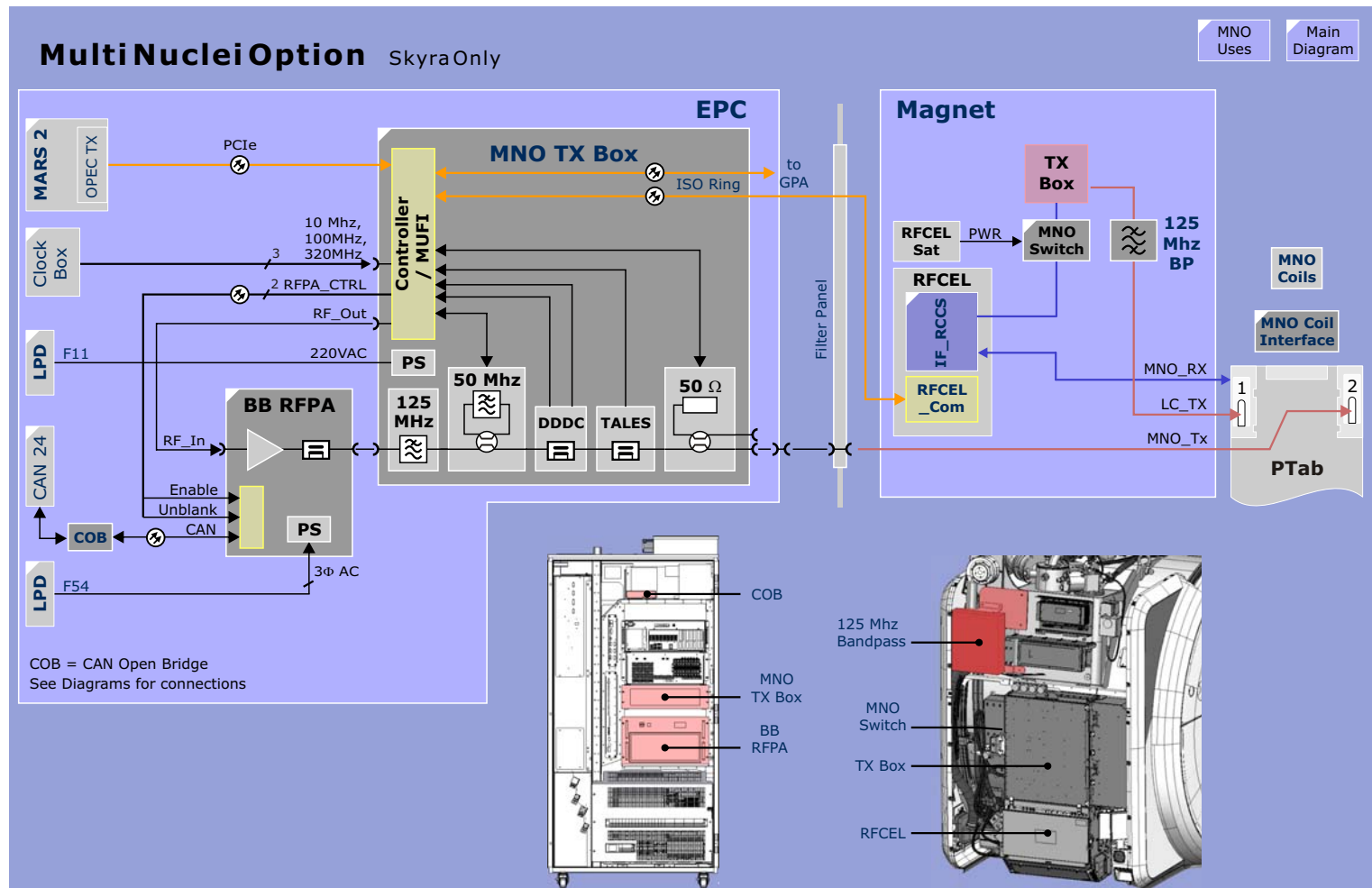
Figure 86 Multi Nuclear Spectroscopy Option (MNO)
