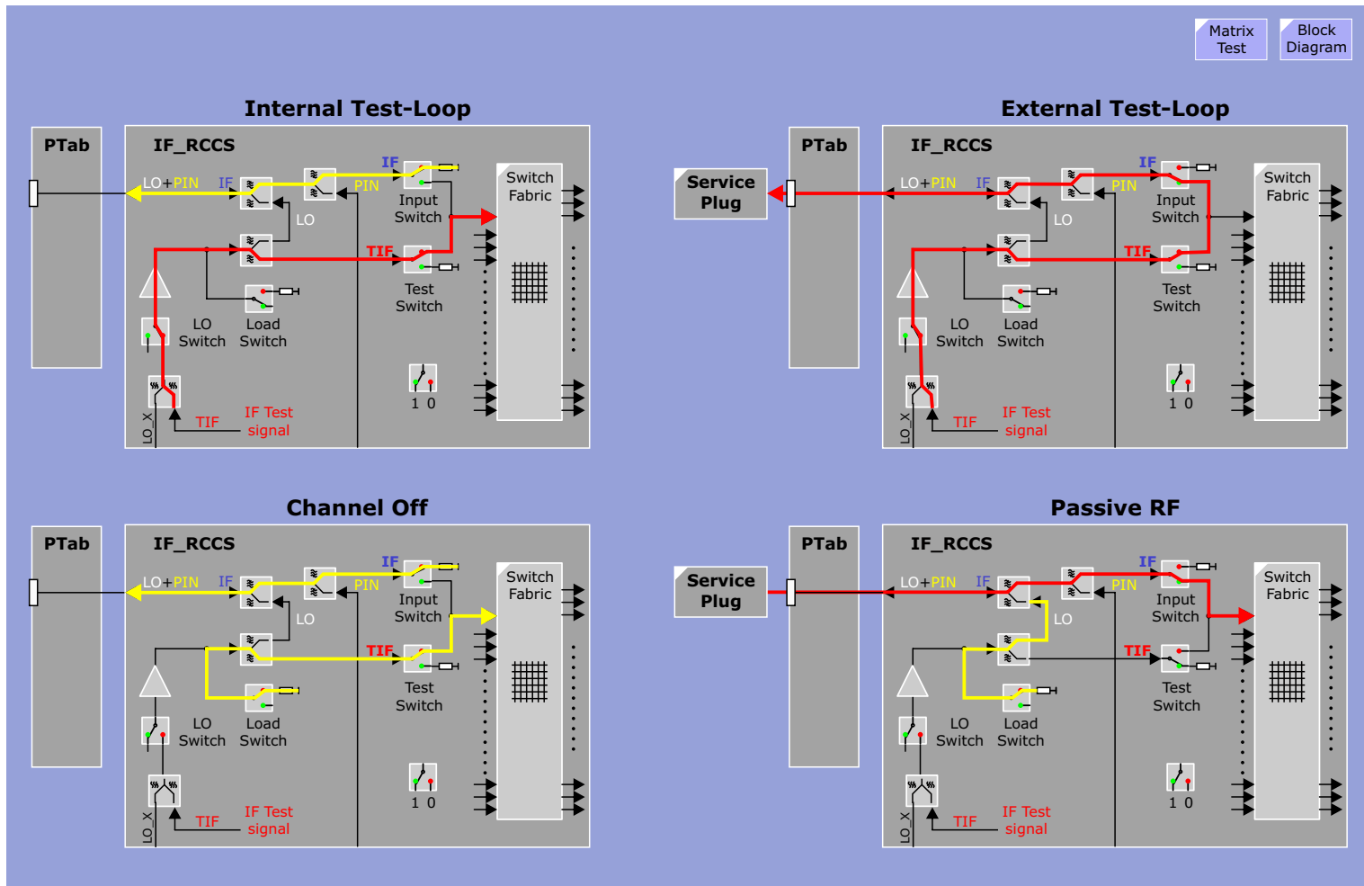
Figure 59 LC Input Multiplexer Settings
