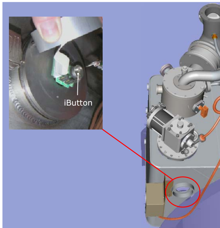
Figure 198 i Button Location
