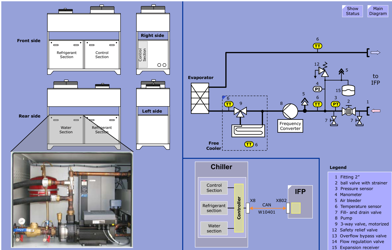
Figure 221 Chiller - Water Circuit Diagram
