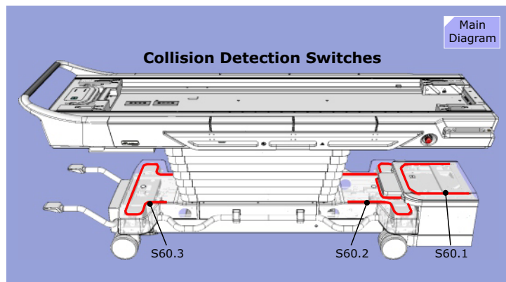
Figure 115 S60 Collision Detection
