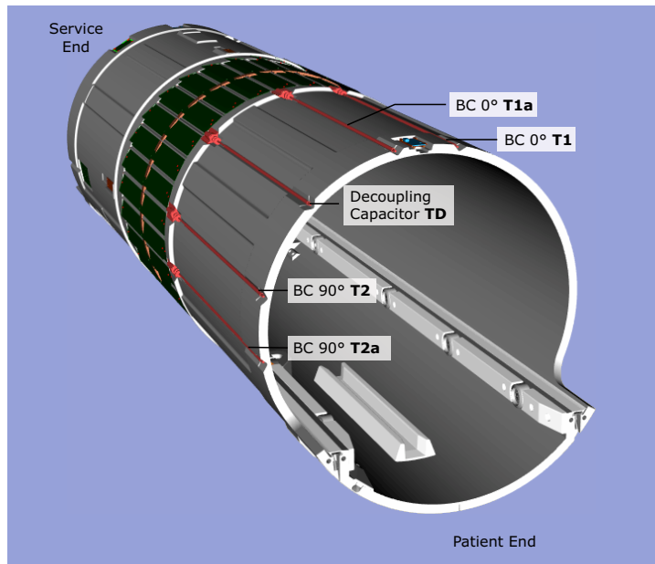
Figure 266 Prisma BC Parts Location
