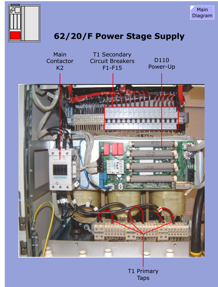
Figure 174 62/20/F Power Stage Supply Layout
