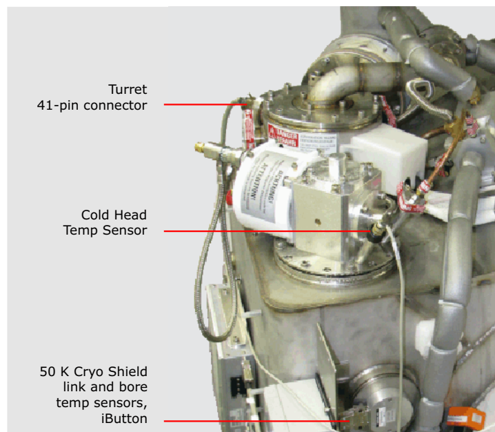
Figure 194 Electrical Connectors
