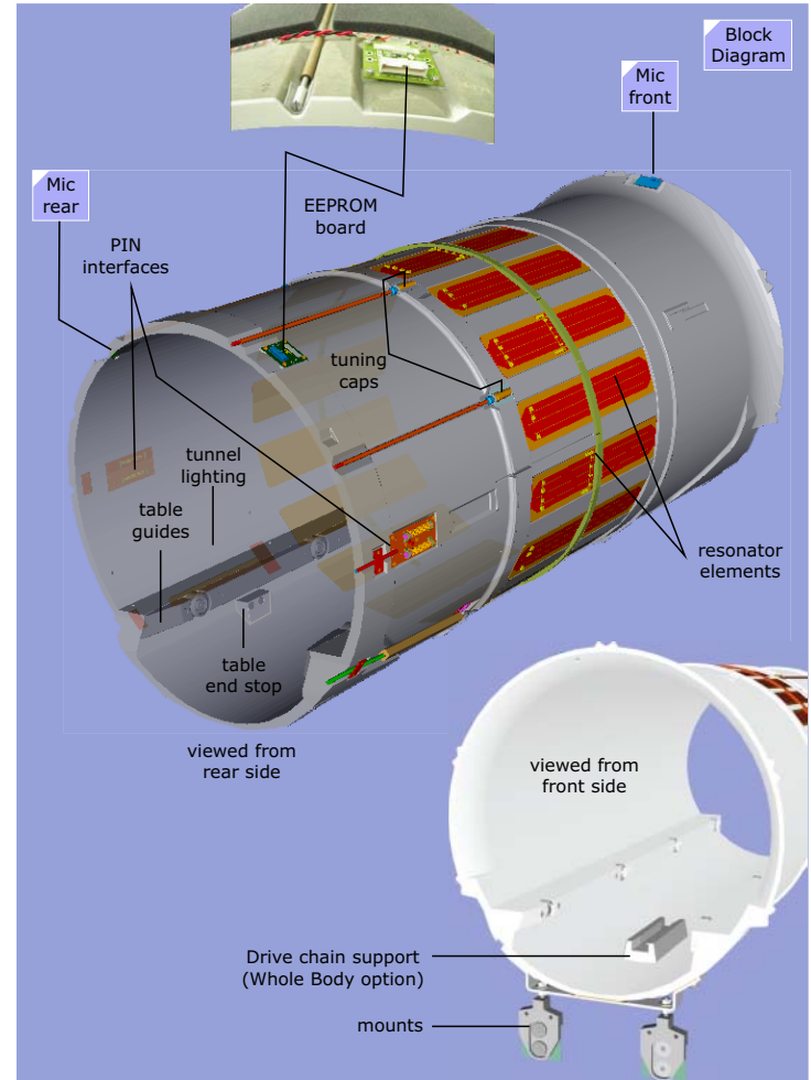
Figure 50 Body Coil Parts Location
