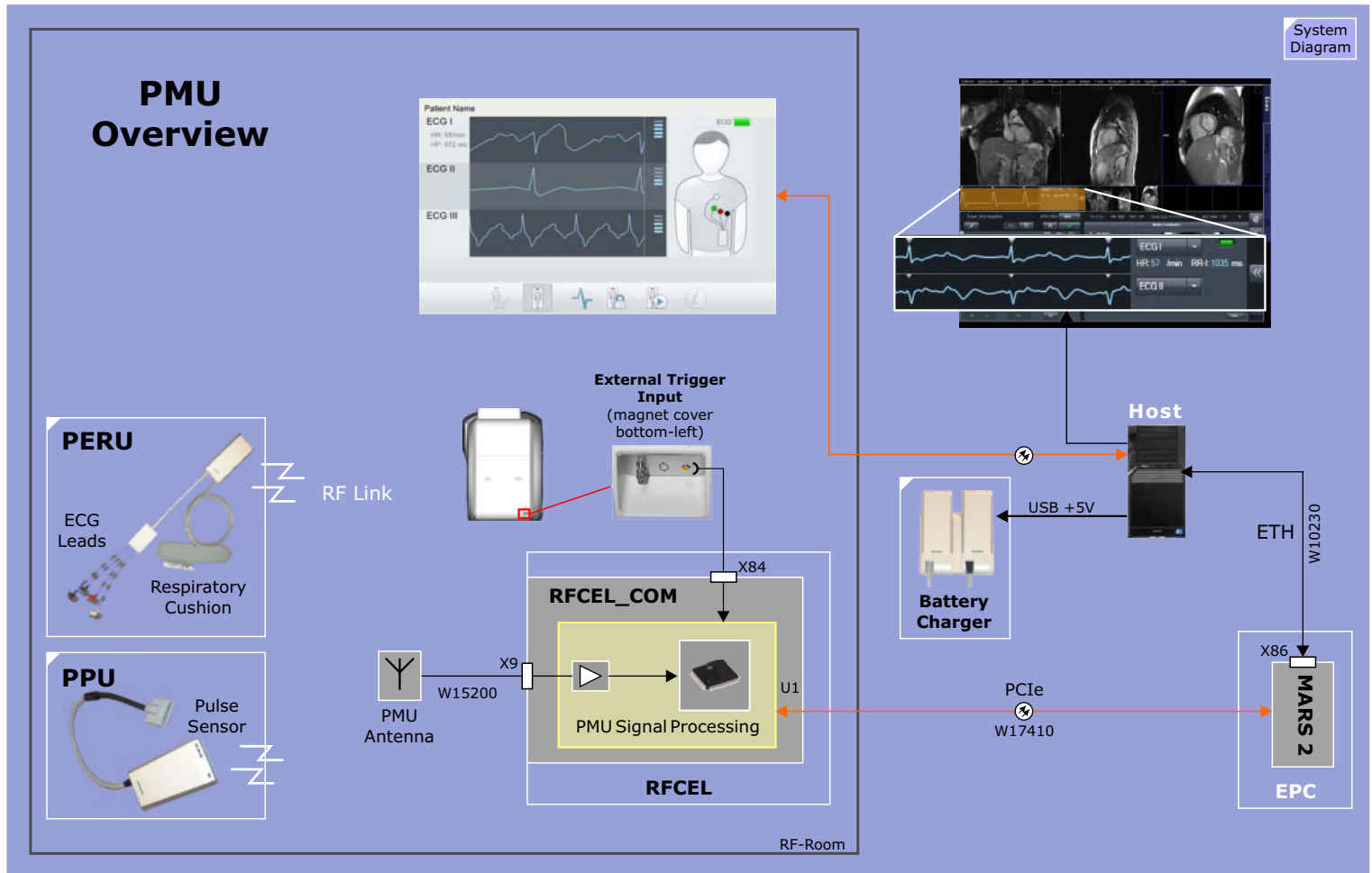
Figure 139 Physiological Measurement Unit (PMU) Block Diagram
