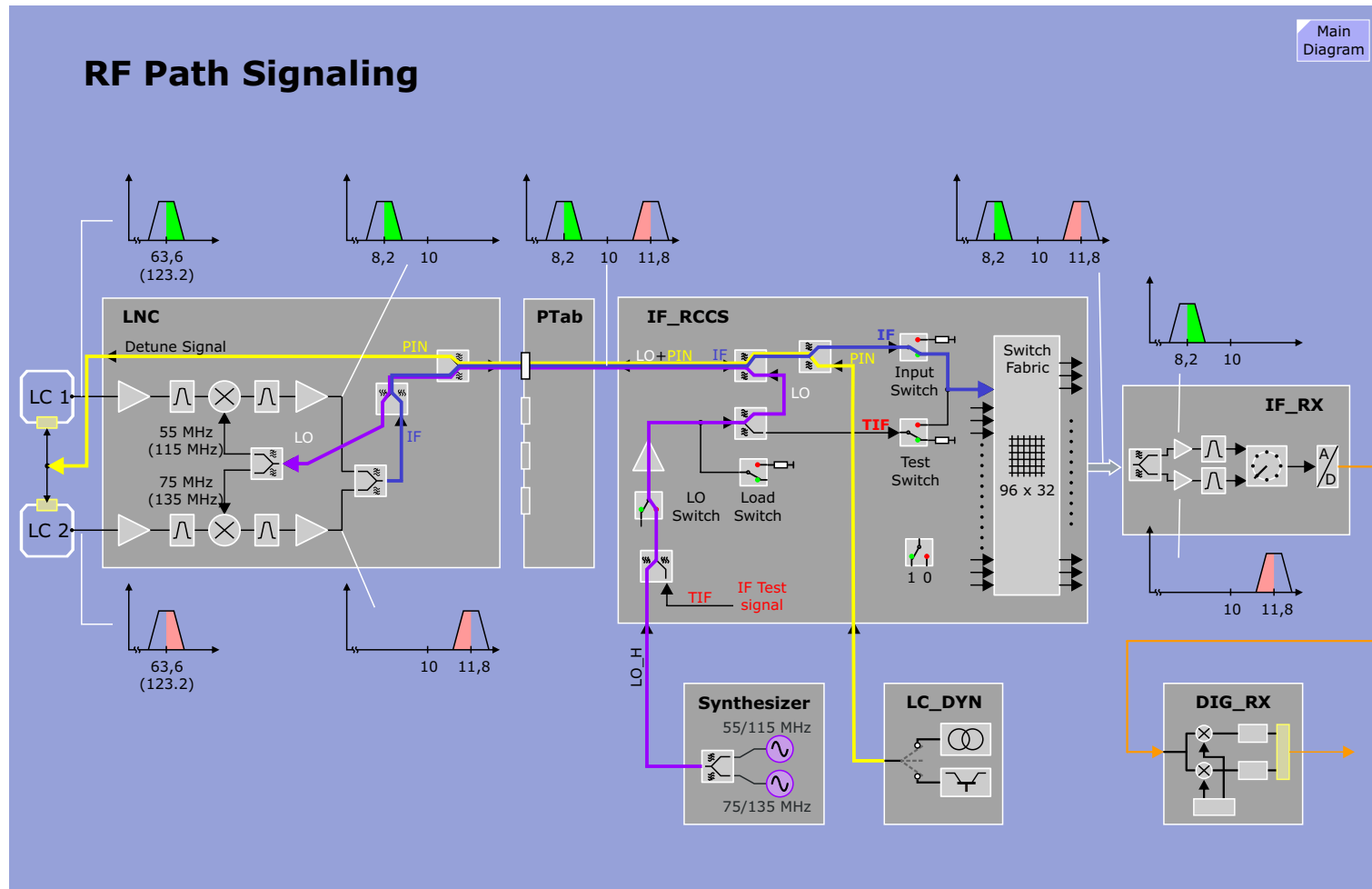
Figure 55 Receive Path Overview
