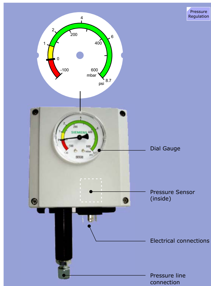
Figure 195 Pressure Display & Control Switch
