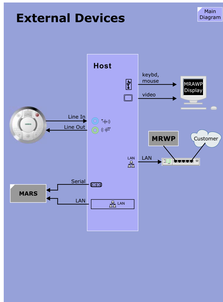
Figure 23 External Devices
