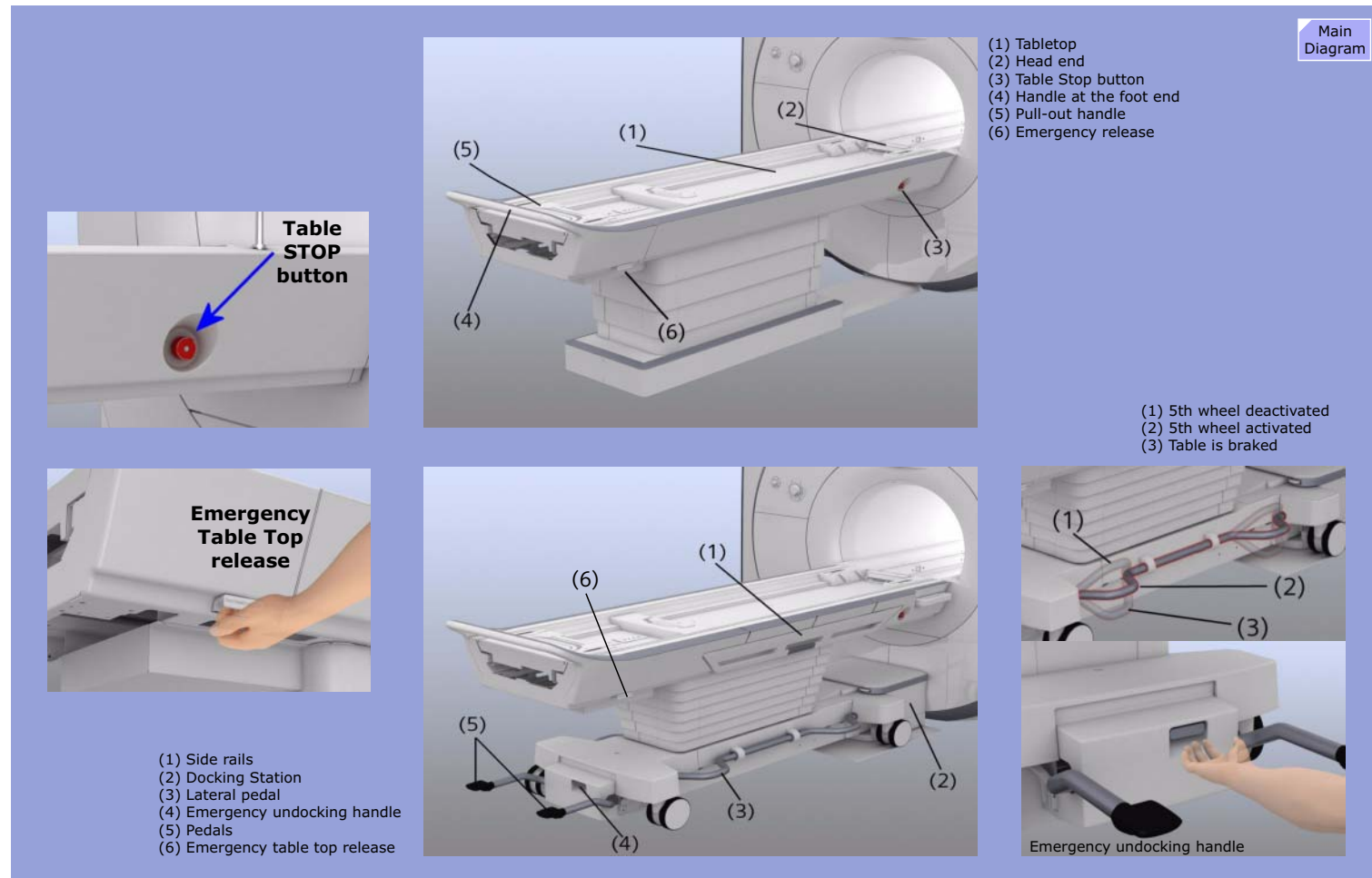
Figure 91 Table Features
