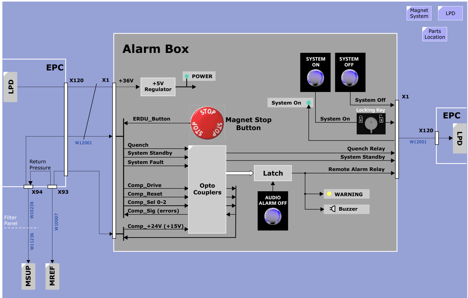
Figure 204 Alarm Box Block Diagram
