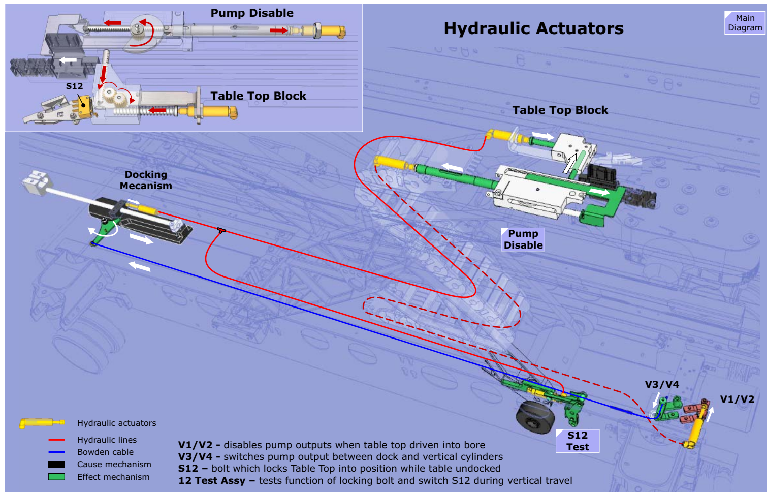
Figure 124 Tim Dockable Table - Mechanical Safety Interlocks
