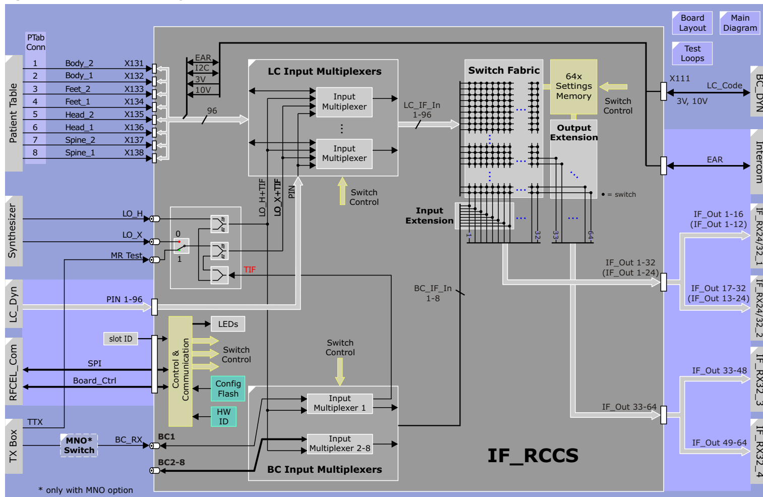
Figure 56 IF_RCCS Block Diagram
