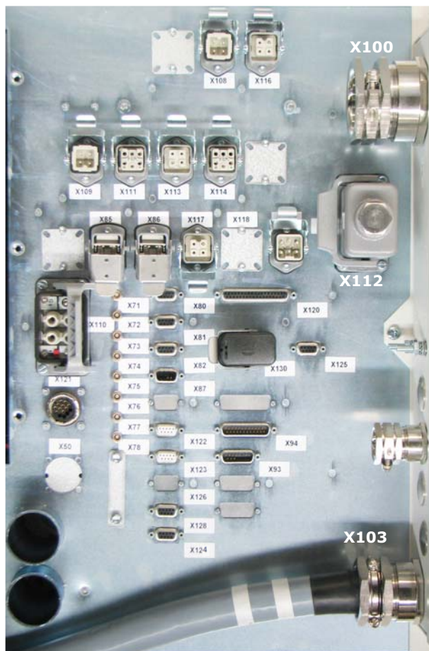
Figure 228 Mains Box and EPC Roof Connections
