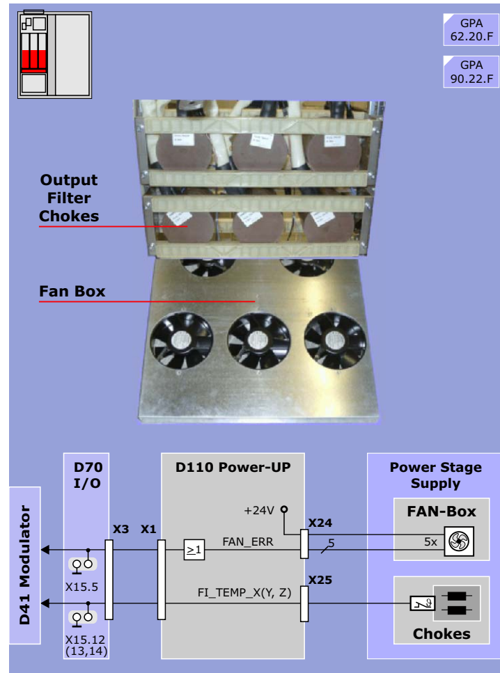
Figure 181 Output Filter-Chokes and Fan Box
