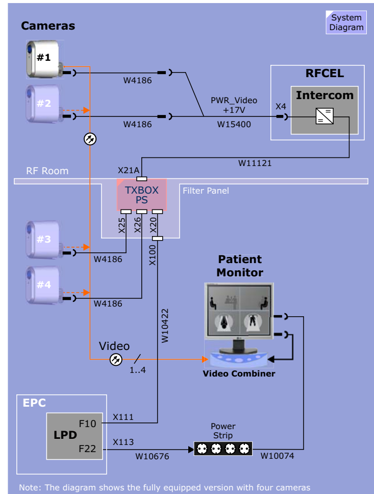
Figure 138 Patient Video Block Diagram
