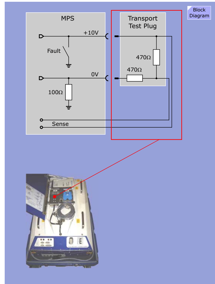
Figure 258 Transport Test Plug
