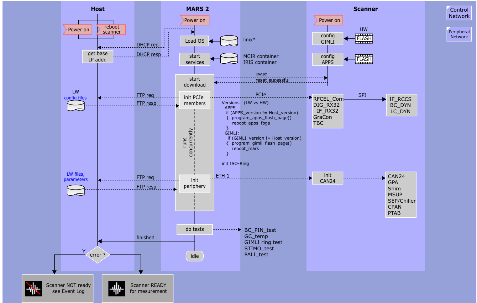
Figure 36 Scanner Boot Process Diagram
