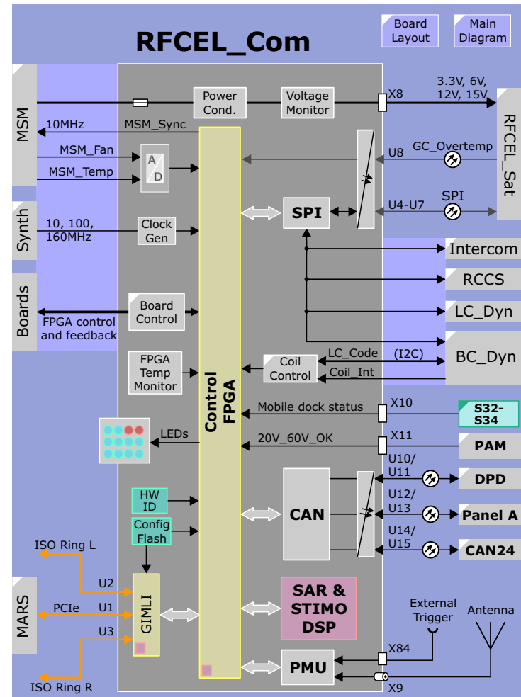
Figure 70 RFCEL_Com Block Diagram
