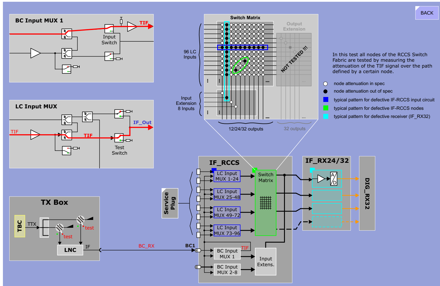
Figure 60 IF_RCCS / IF_RX32 Functional Test
