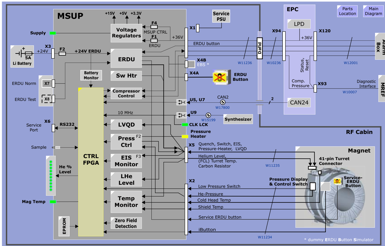
Figure 197 MSUP 2306 Block Diagram
