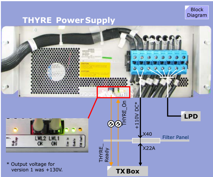
Figure 48 THYRE Power Supply
