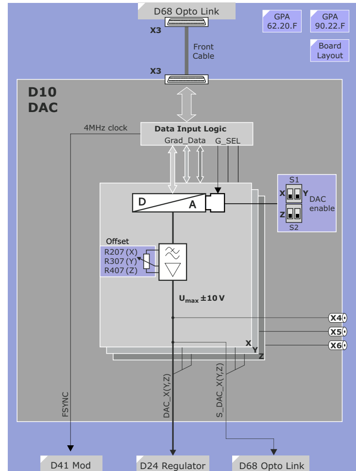
Figure 148 D10 DAC Block Diagram
