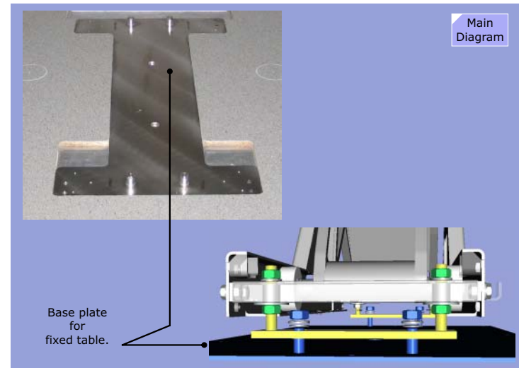
Figure 92 Base Mount Plate
