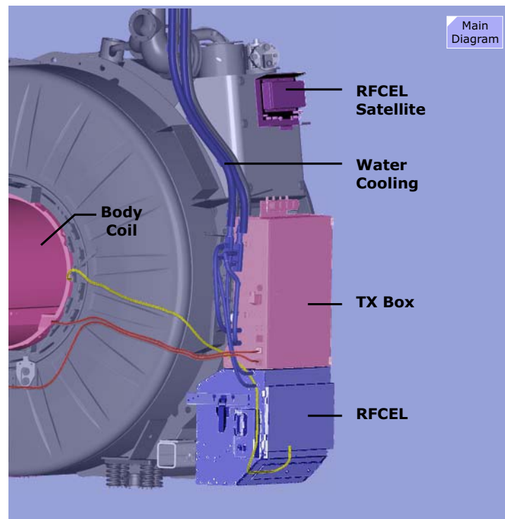
Figure 43 Aera/Skyra RF System
