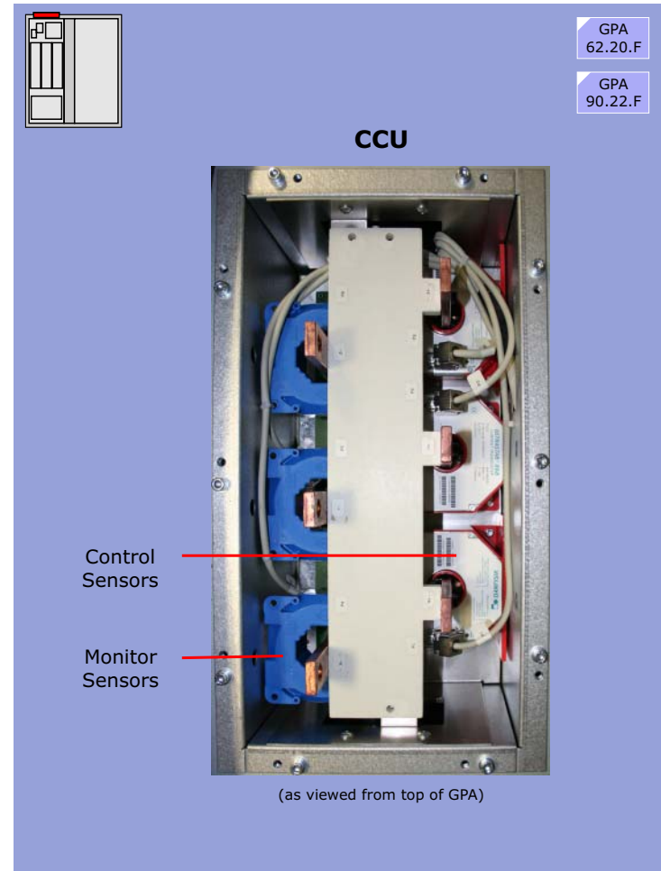
Figure 180 Current Converter Unit (CCU)
