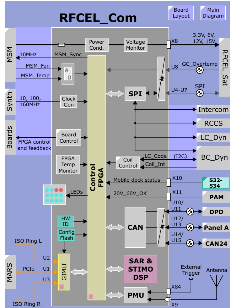
Figure 67 RFCEL_Com Block Diagram
