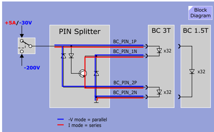
Figure 65 PIN Splitter
