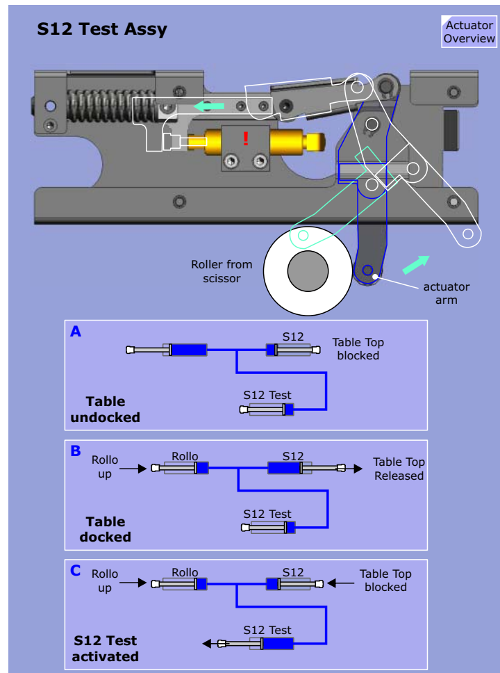
Figure 114 S12 Test Assembly
