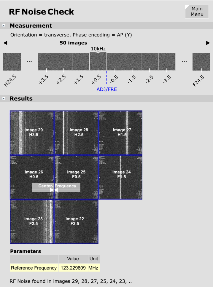
Figure 252 RF Noise Check
