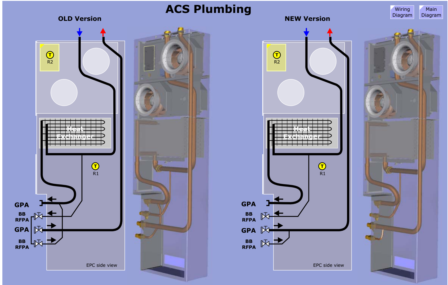
Figure 214 ACS Plumbing Diagram
