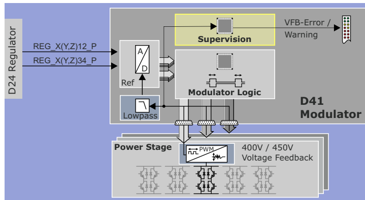
Figure 157 D41 Modulator VFB
