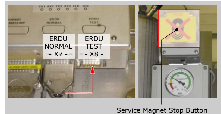
Figure 199 ERDU Test Connector
