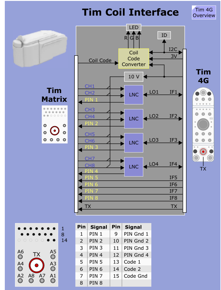
Figure 82 Tim Coil Interface Block Diagram
