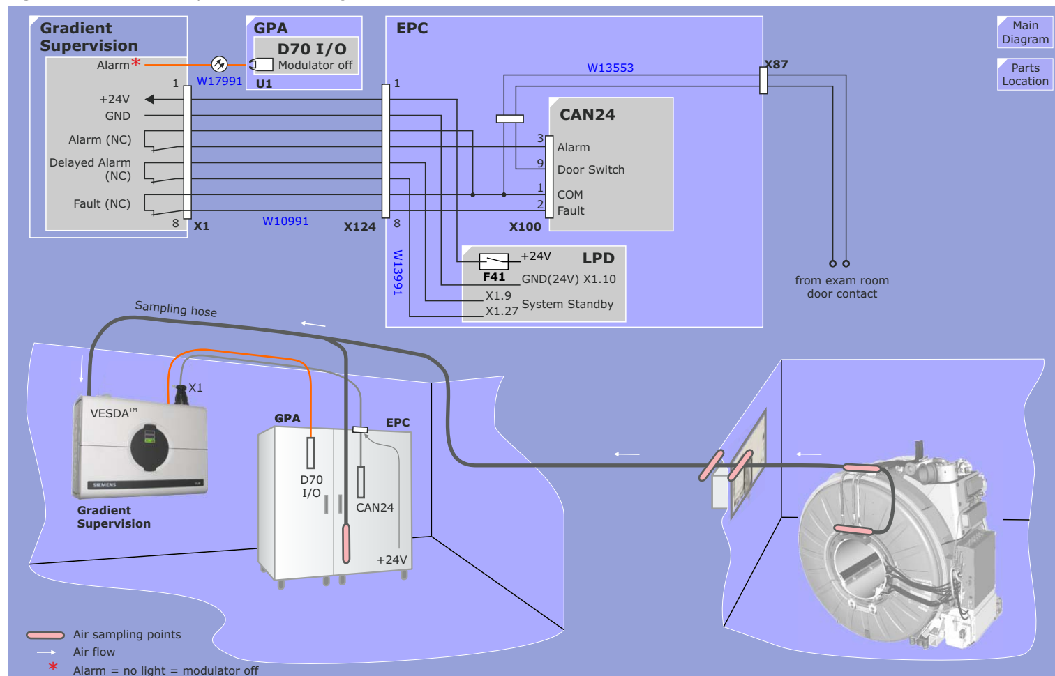
Figure 184 Gradient Supervision Block Diagram
