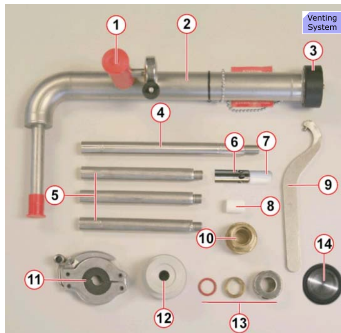
Figure 255 Helium Service Syphon Kit
