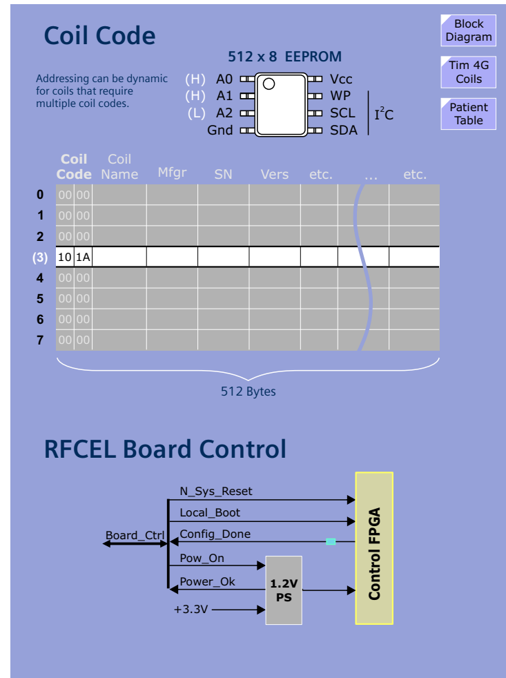
Figure 69 Coil Code and Board Control
