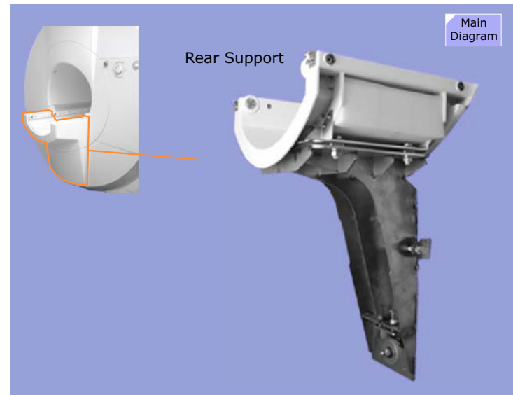
Figure 127 Whole Body Option - Rear Support
