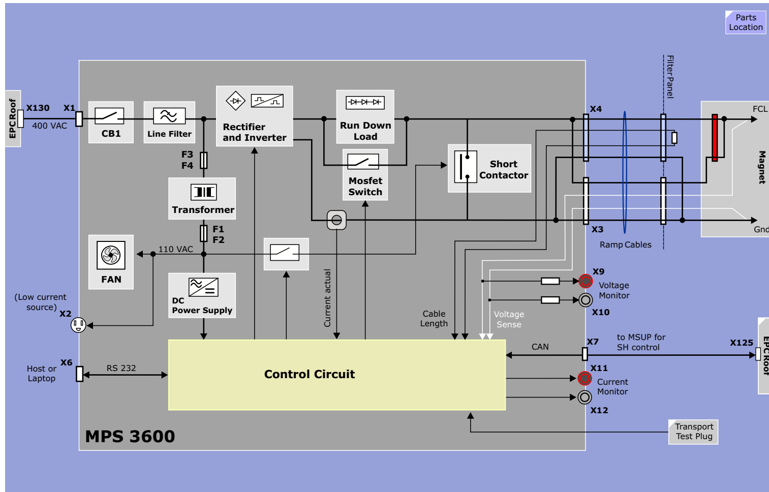
Figure 257 Magnet Power Supply 3600 Block Diagram
