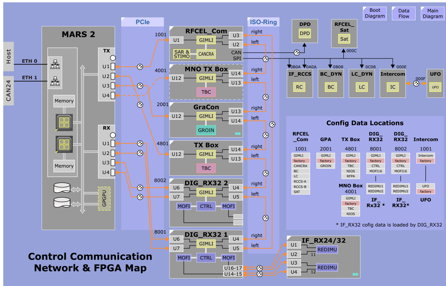
Figure 35 FPGA Topology
