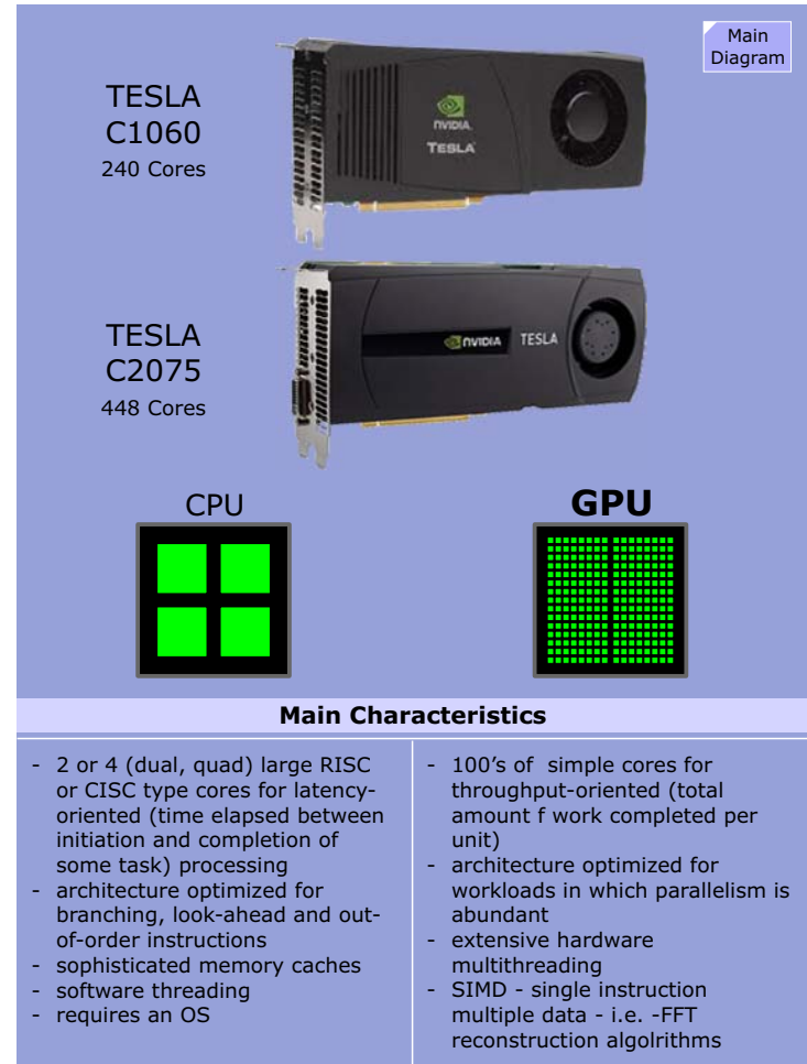
Figure 31 NVIDIA Tesla GPGPU
