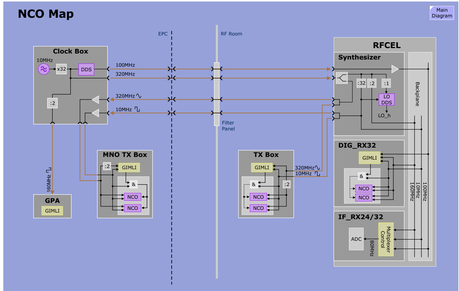
Figure 42 Map of all DDS and NCO Blocks
