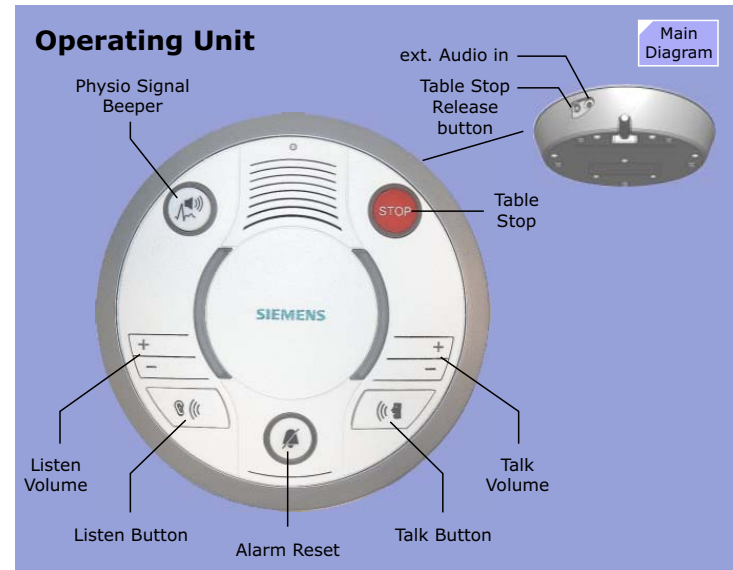
Figure 136 Intercom Operating Unit
