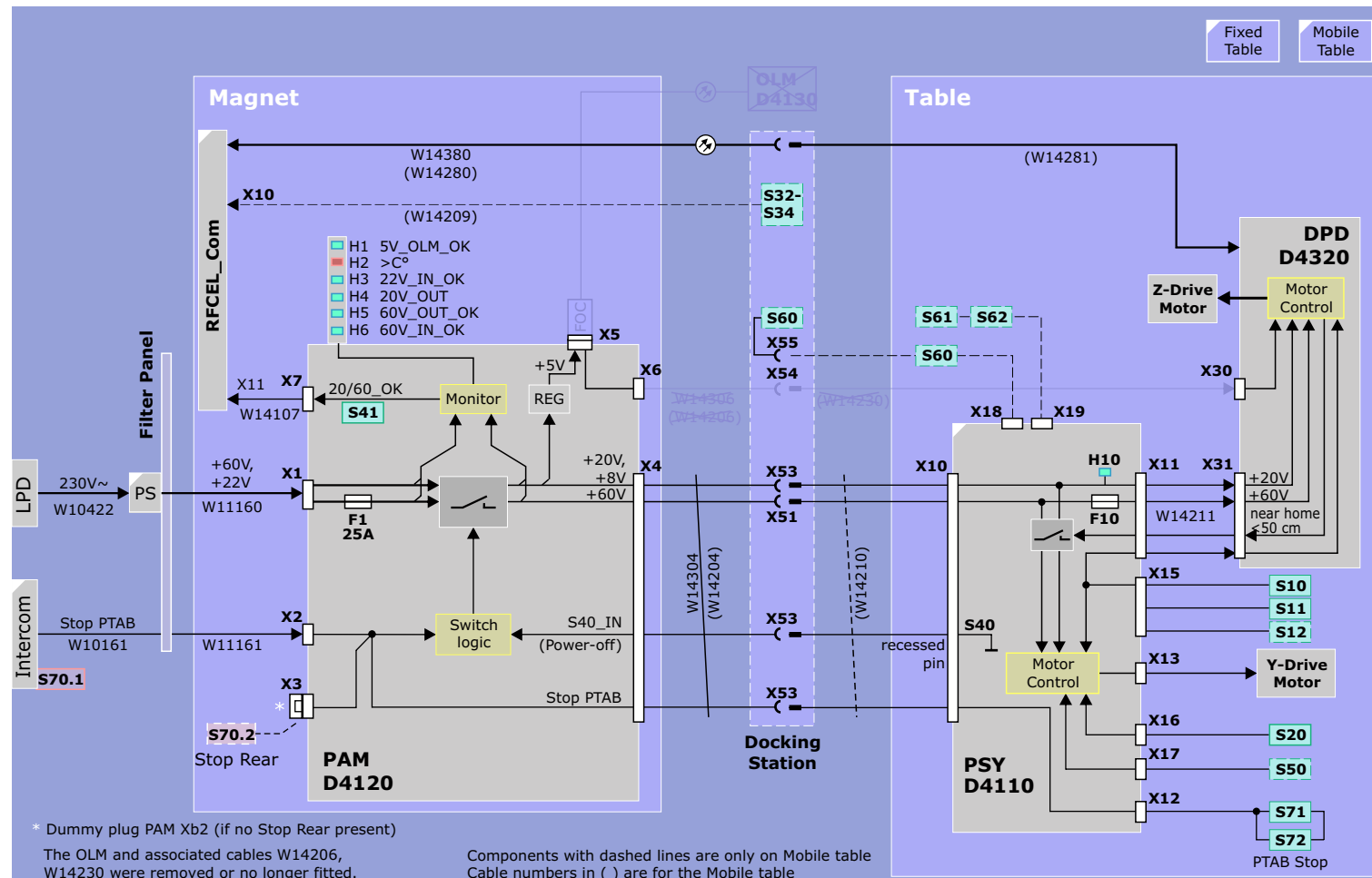
Figure 101 Electrical Components Block Diagram
