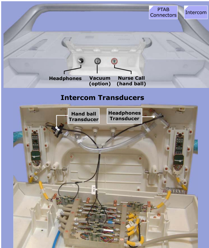
Figure 126 Coil and Auxiliary Connections
