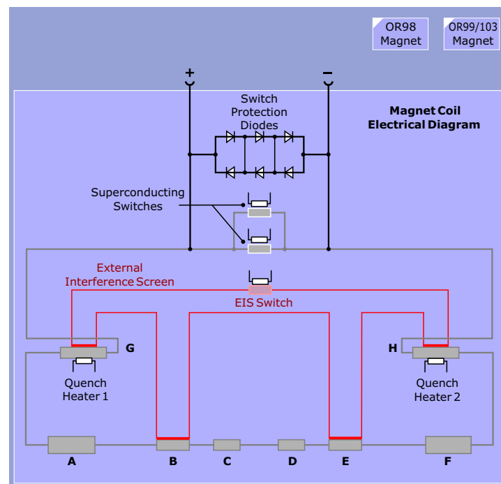
Figure 189 Magnet Electrical Diagram
