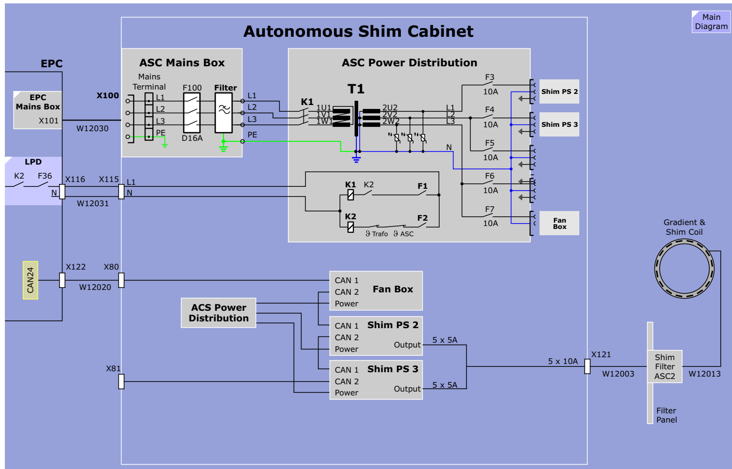
Figure 265 Autonomous Shim Cabinet Block Diagram
