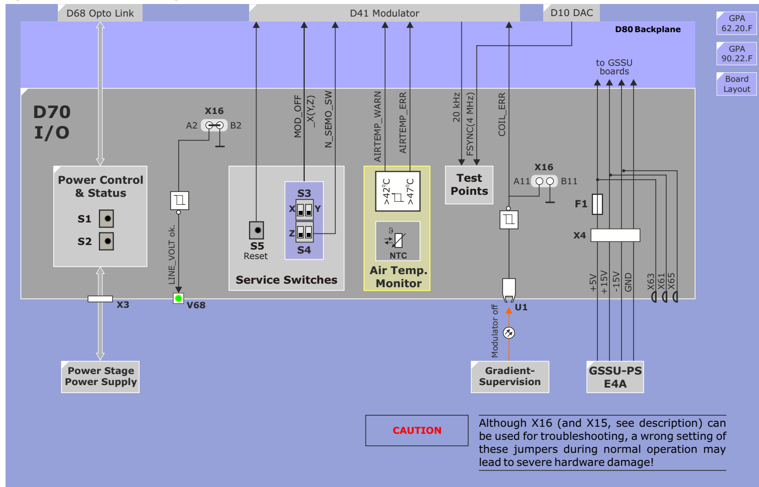
Figure 167 D70 I/O Block Diagram
