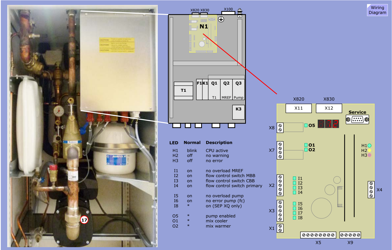
Figure 218 SEP Controller Layout
