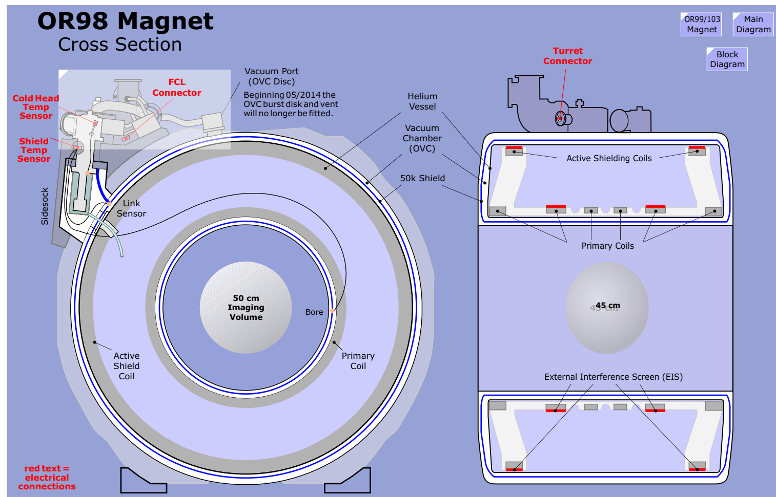
Figure 190 OR98 Magnet - Cross Sectional Diagram
