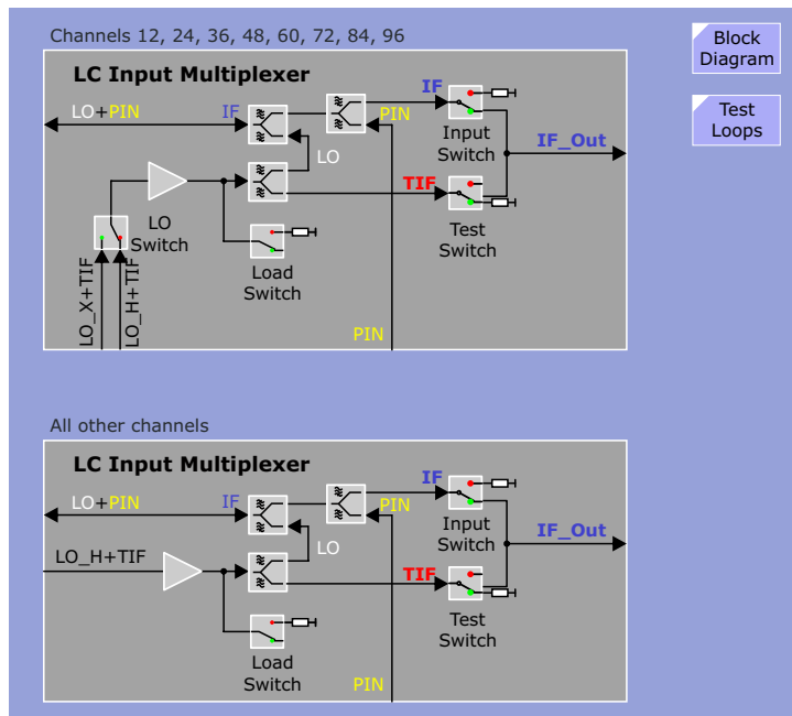
Figure 57 LC Input Multiplexers
