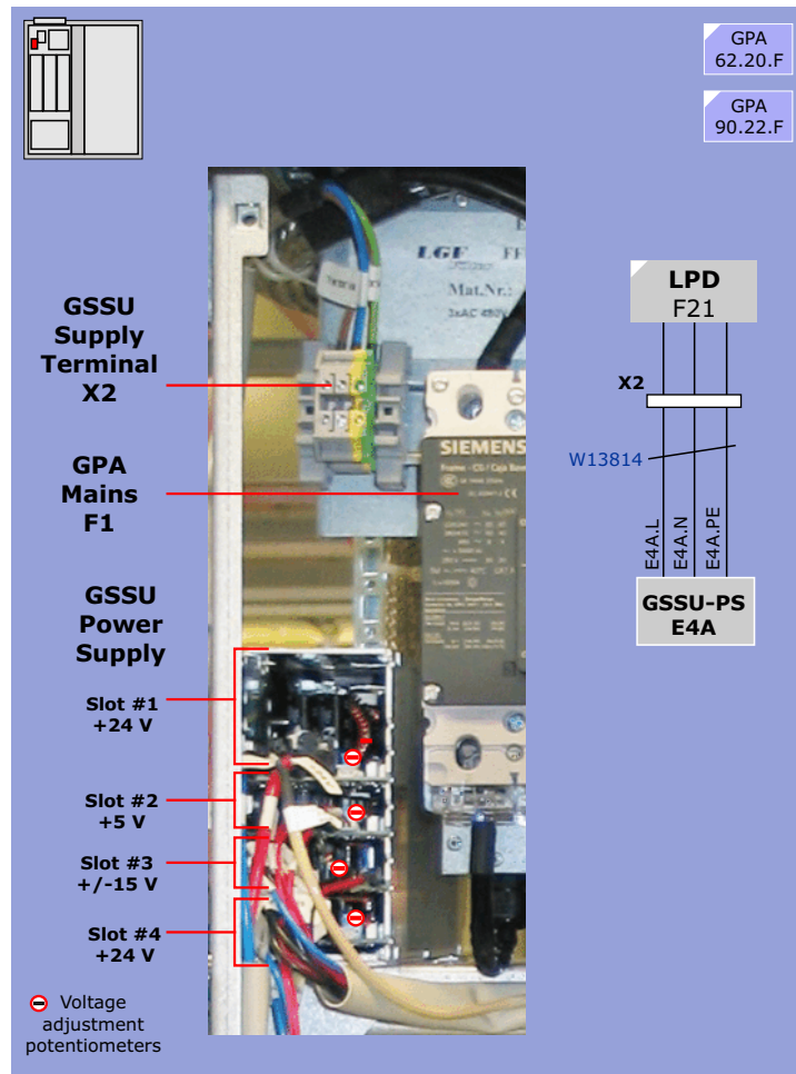
Figure 179 GSSU Power Supply
