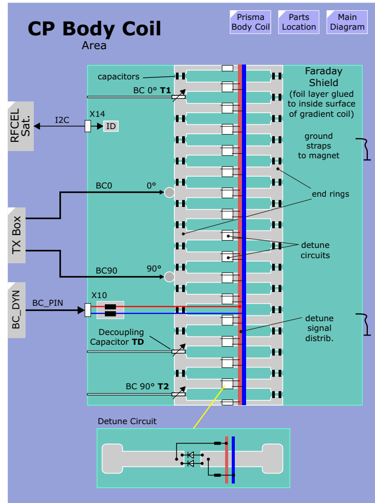
Figure 49 Body Coil Block Diagram
