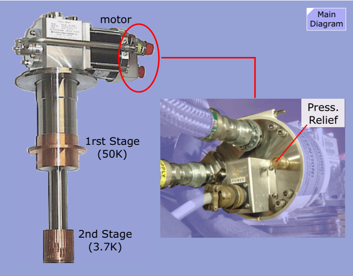
Figure 210 Cold Head
