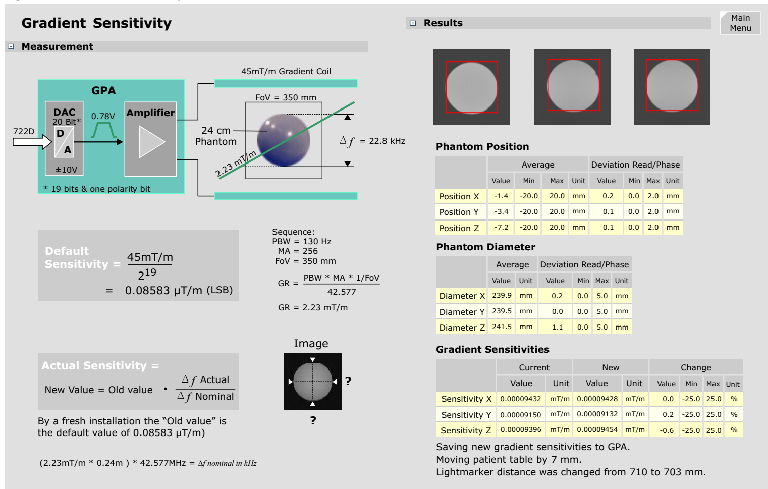
Figure 240 Gradient Sensitivity Measurement and Results
