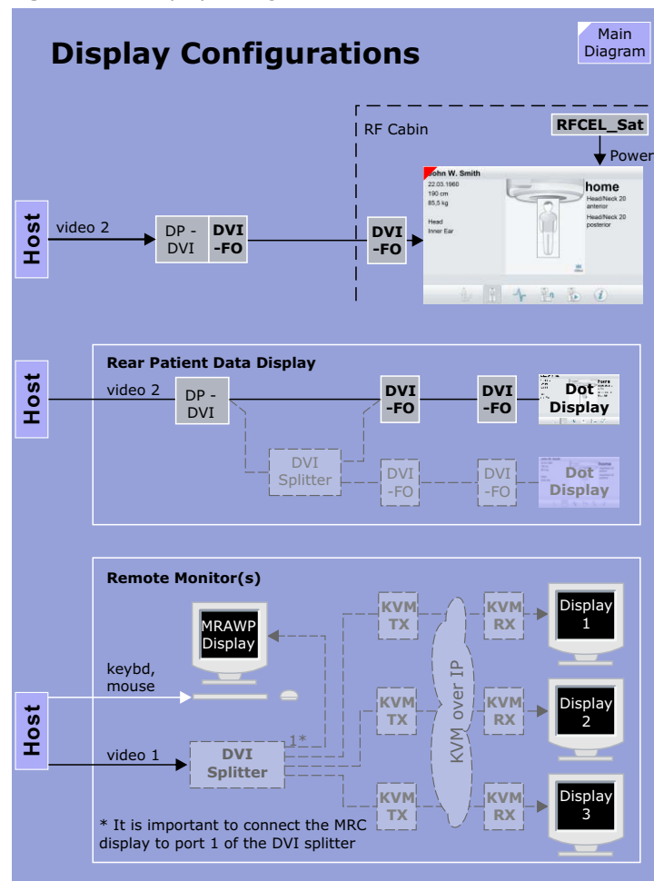
Figure 24 Display Configurations
