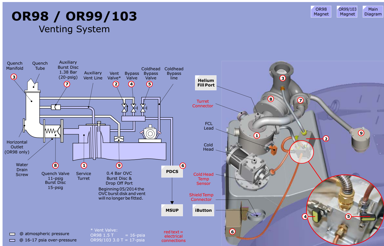
Figure 192 Venting System OR98 / OR99/103
