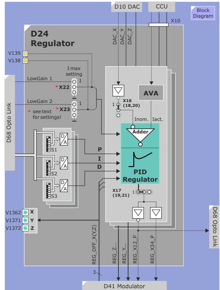
Figure 153 D24 PID Regulator
