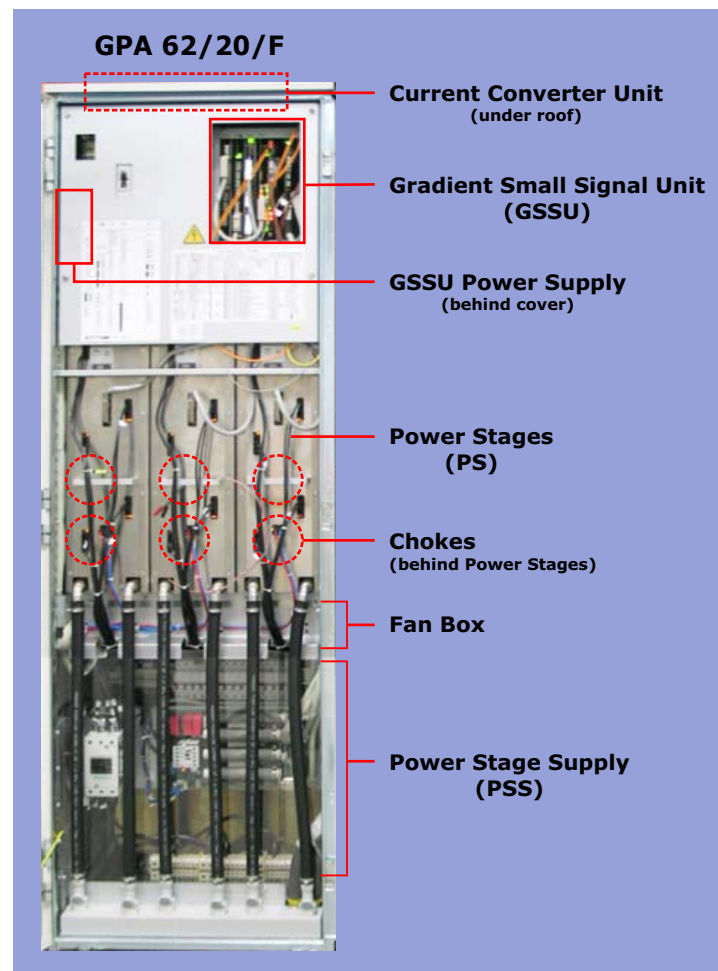
Figure 143 GPA 62/20/F Layout
