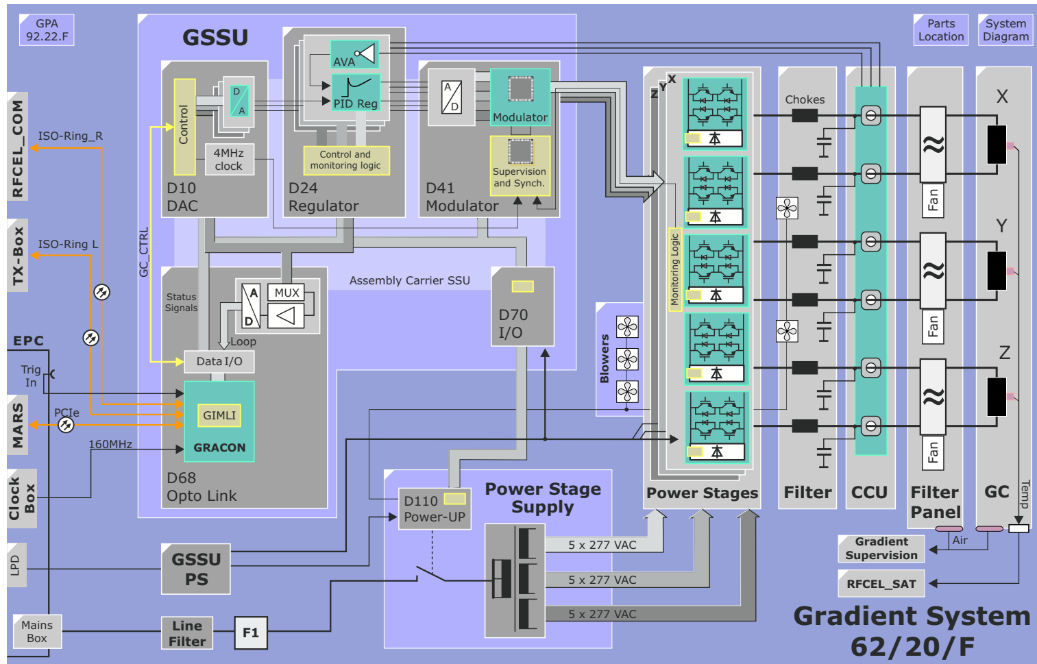
Figure 144 GPA 62/20/F Block Diagram
