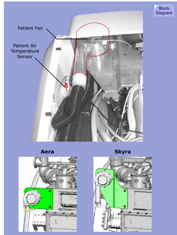
Figure 133 Patient Fan, Air Temp Sensor
