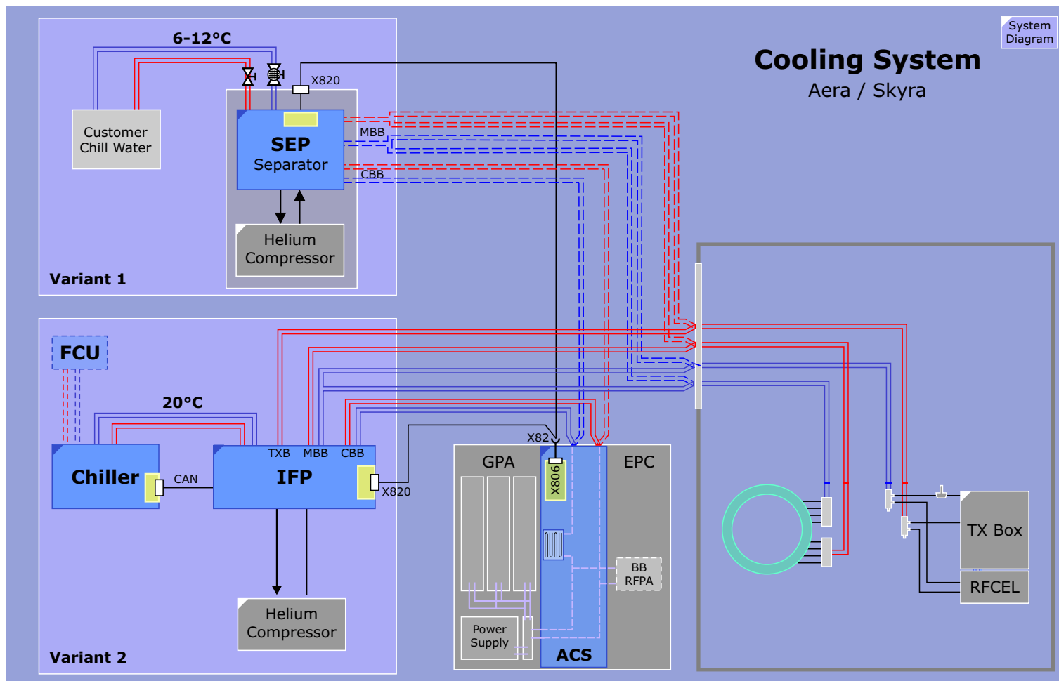
Figure 212 Cooling System Block Diagram
