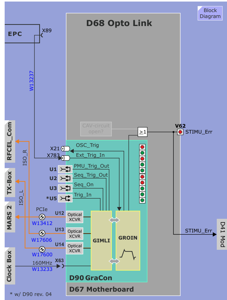
Figure 164 D68 Opto Link - System Interface
