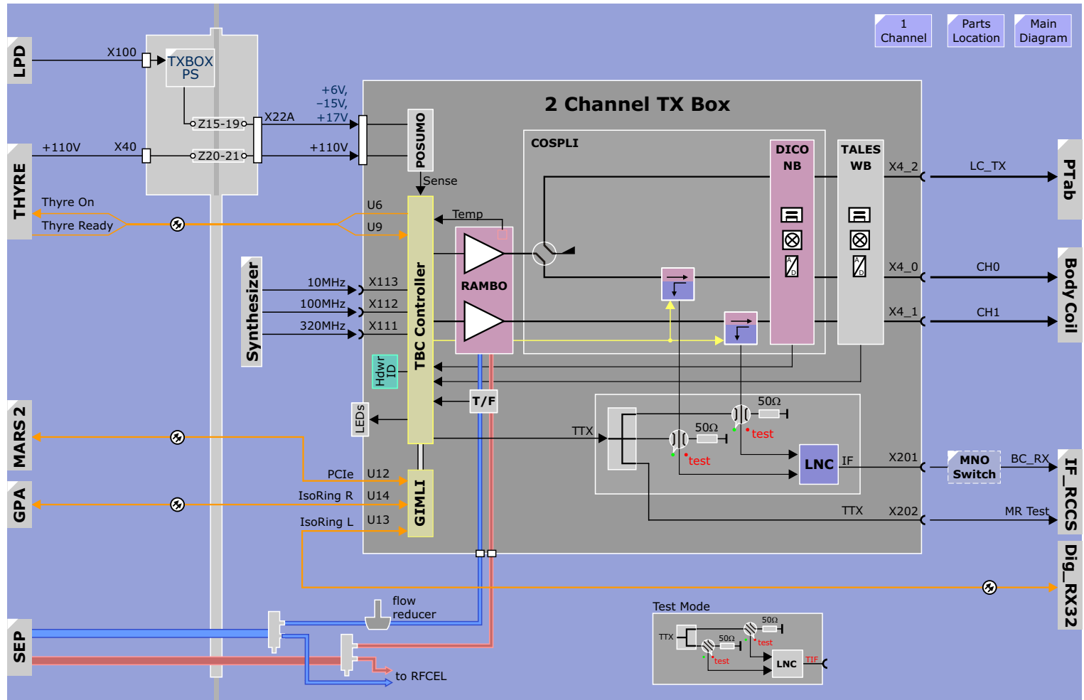
Figure 47 2 Channel TX Box Block Diagram
