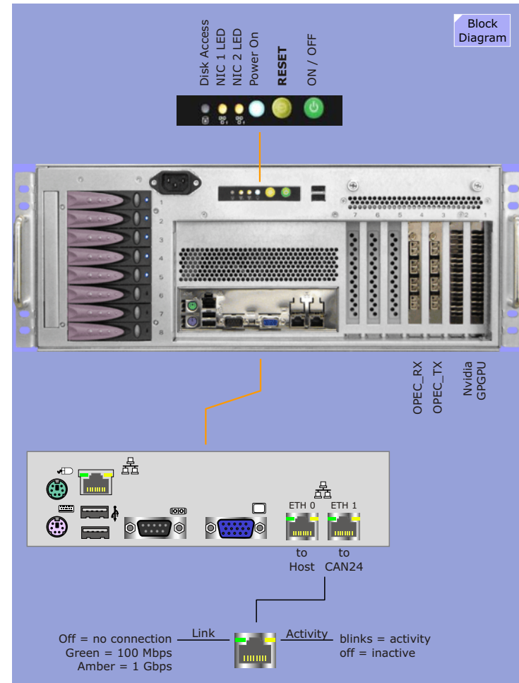
Figure 28 MARS 2 Layout
