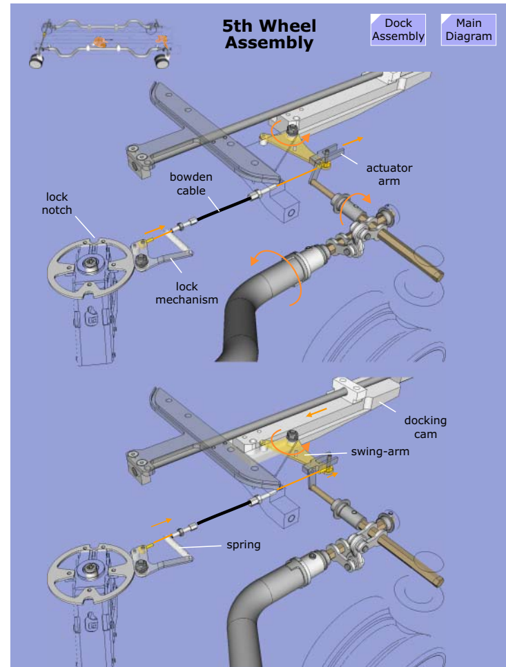
Figure 110 5th Wheel Assembly
