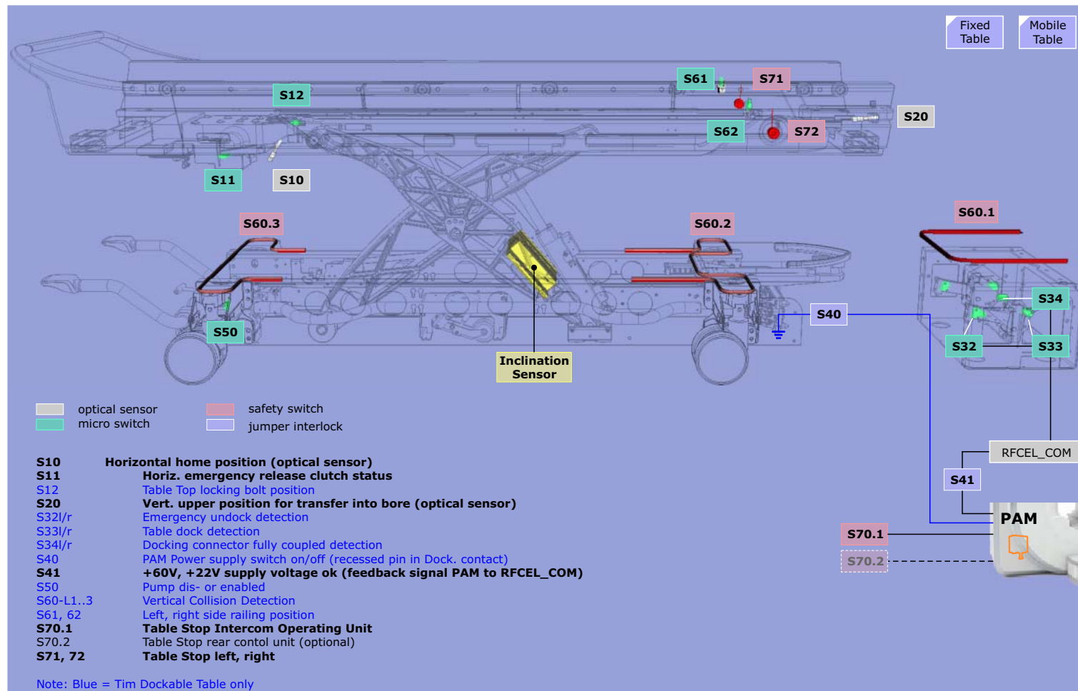
Figure 125 Patient Table Switches and Sensors Location
