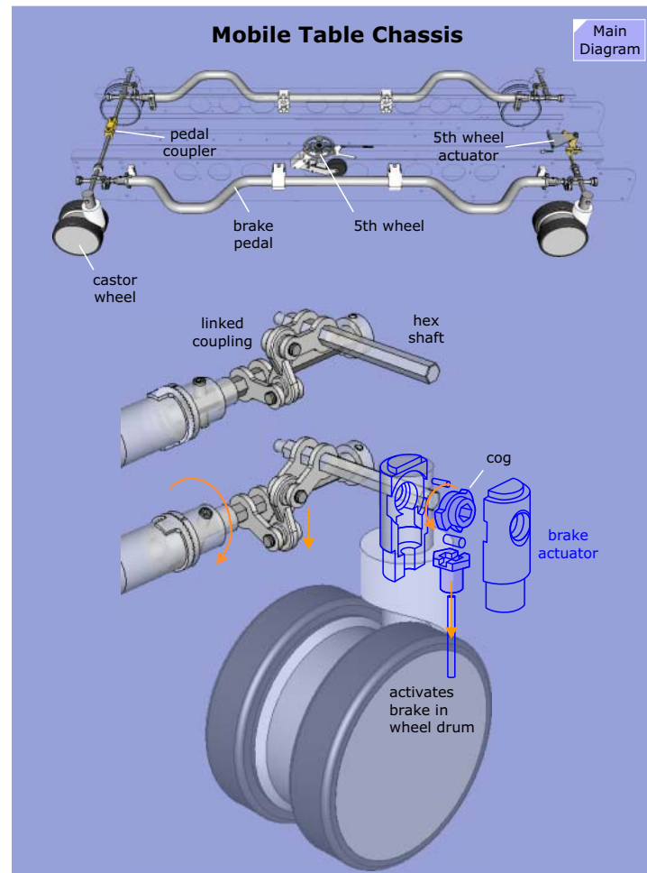
Figure 109 Wheel and Brake Assembly
