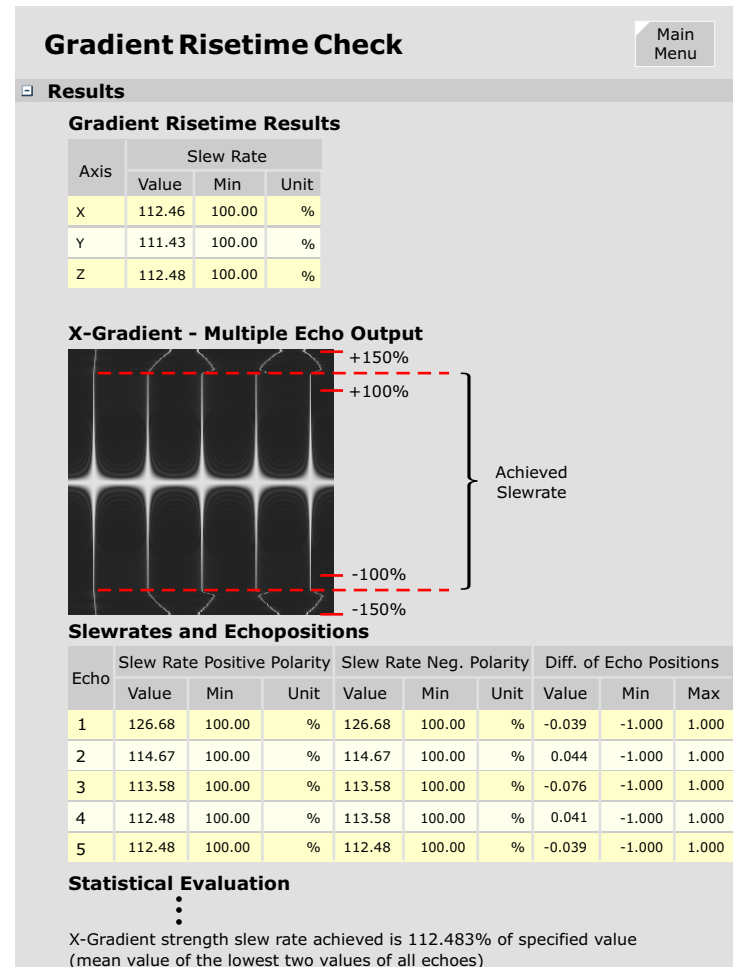
Figure 253 Gradient Rise Time Check
