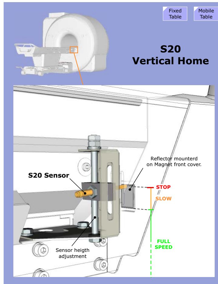
Figure 99 S20 - Vertical HOME Sensor
