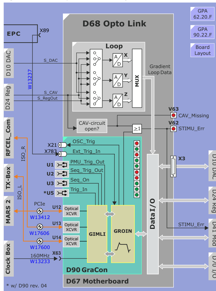
Figure 163 D68 Opto Link Block Diagram
