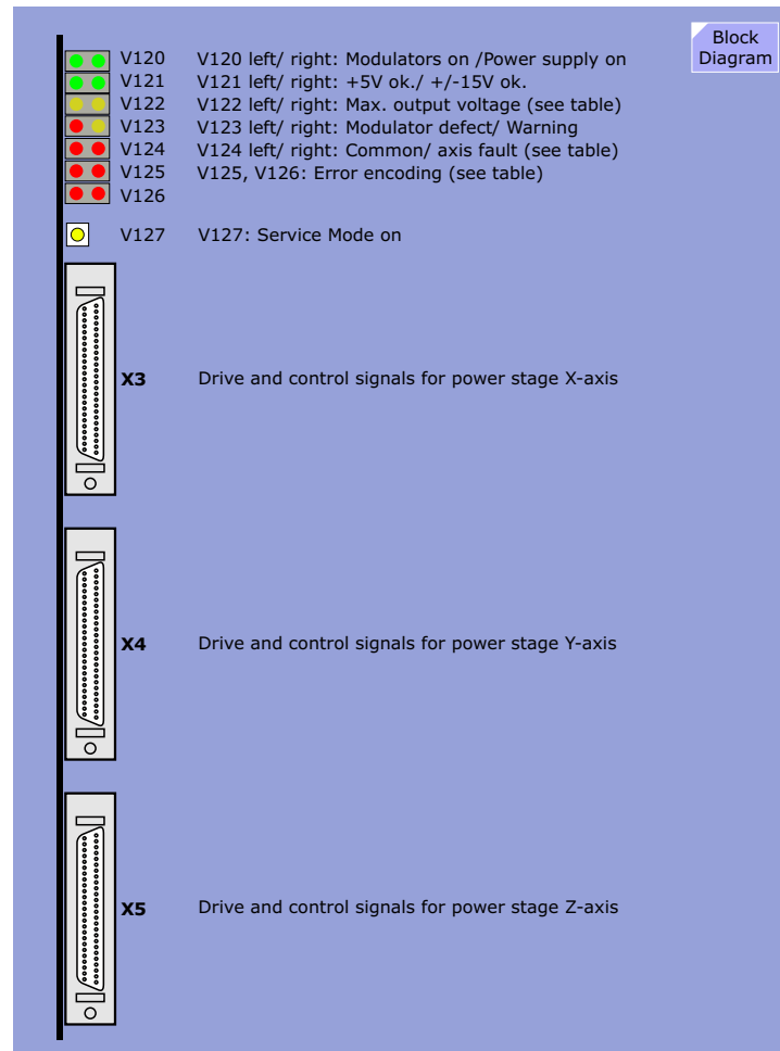
Figure 161 D41 Board Layout
