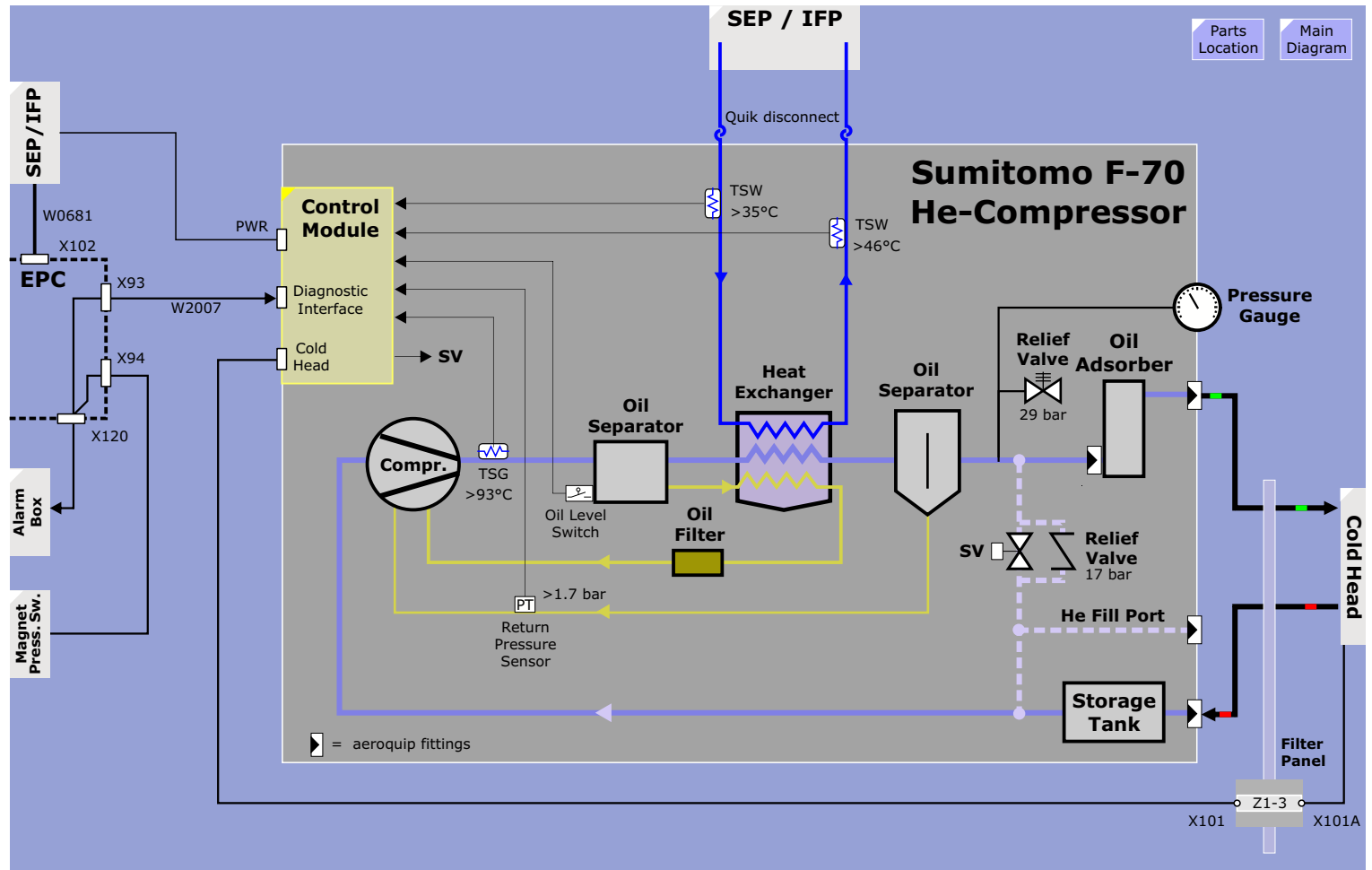
Figure 207 F70 Compressor Block Diagram
