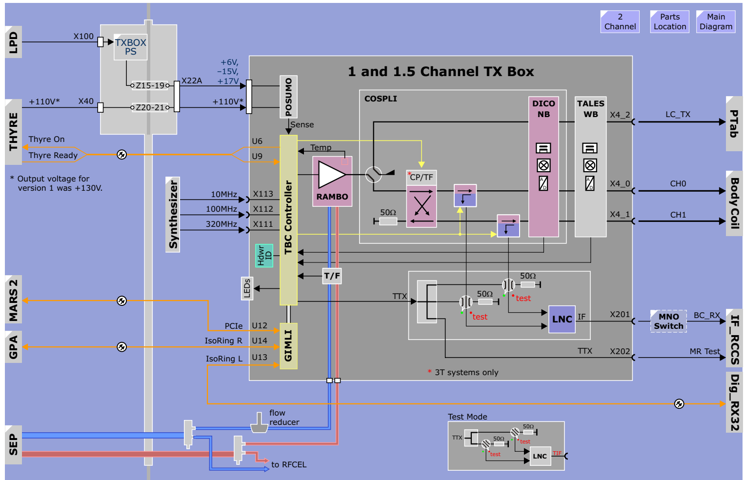
Figure 46 1 and 1.5 Channel TX Box Block Diagram
