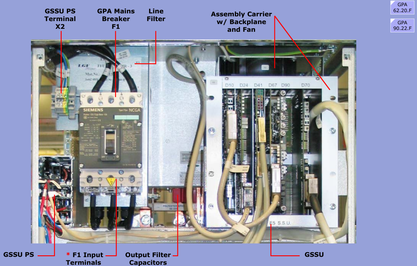
Figure 147 GSSU Layout
