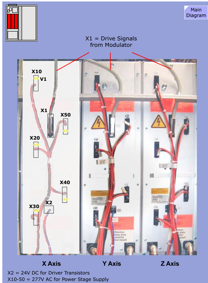
Figure 169 62/20/F Power Stage Layout
