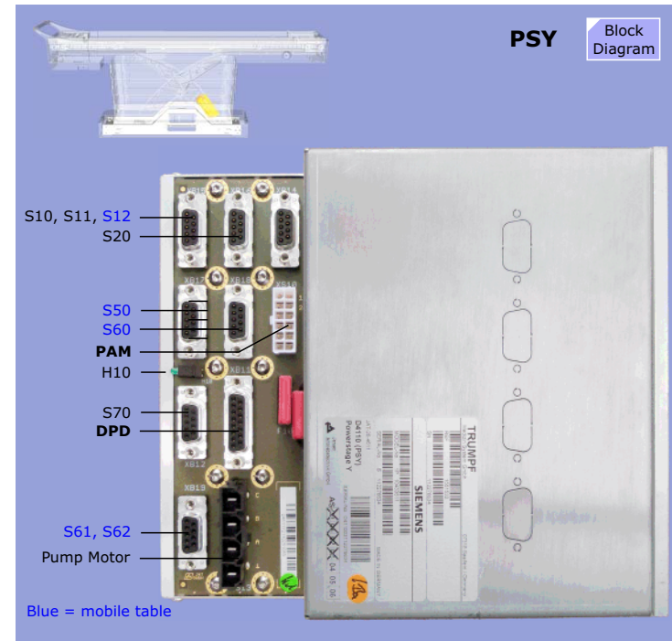
Figure 100 PSY - Power Stage Y
