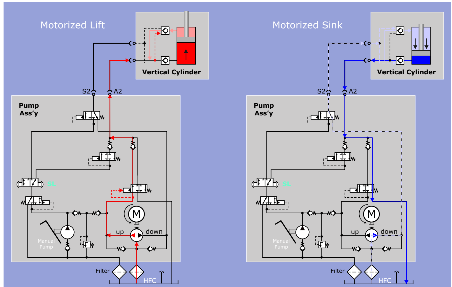
Figure 97 Hydraulic Overview Tim Table
