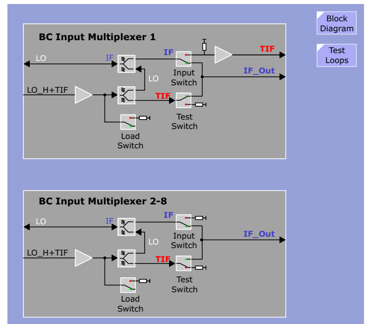
Figure 58 BC Input Multiplexers
