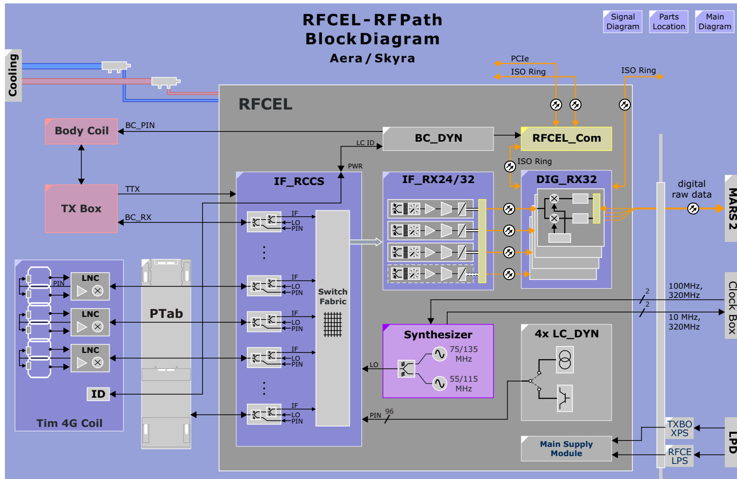
Figure 53 RFCEL - RF Path Block Diagram
