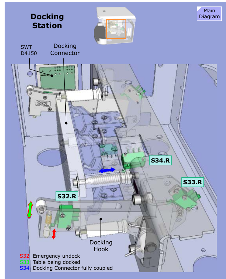
Figure 123 Dock Assembly
