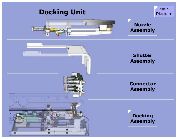
Figure 118 Docking Unit
