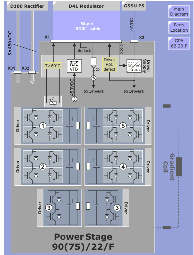
Figure 173 90/22/F Power Stage Block Diagram
