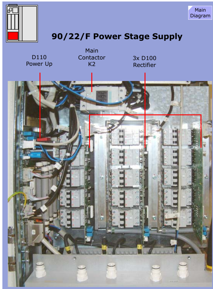
Figure 177 90/22/F Power Stage Supply Layout
