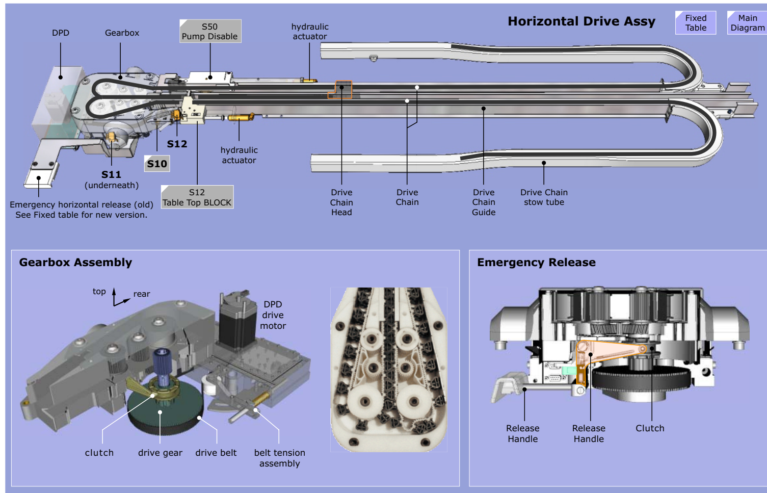
Figure 104 Horizontal Drive System - Mobile Table
