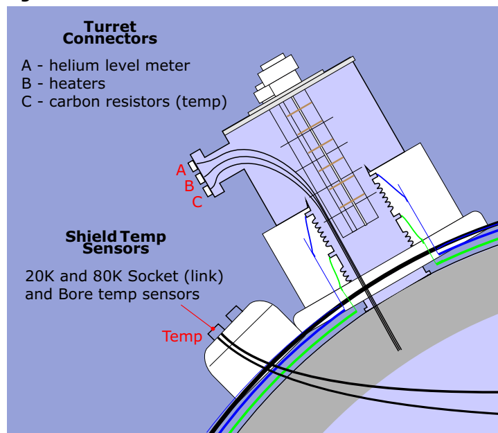
Figure 264 Electrical Connections
