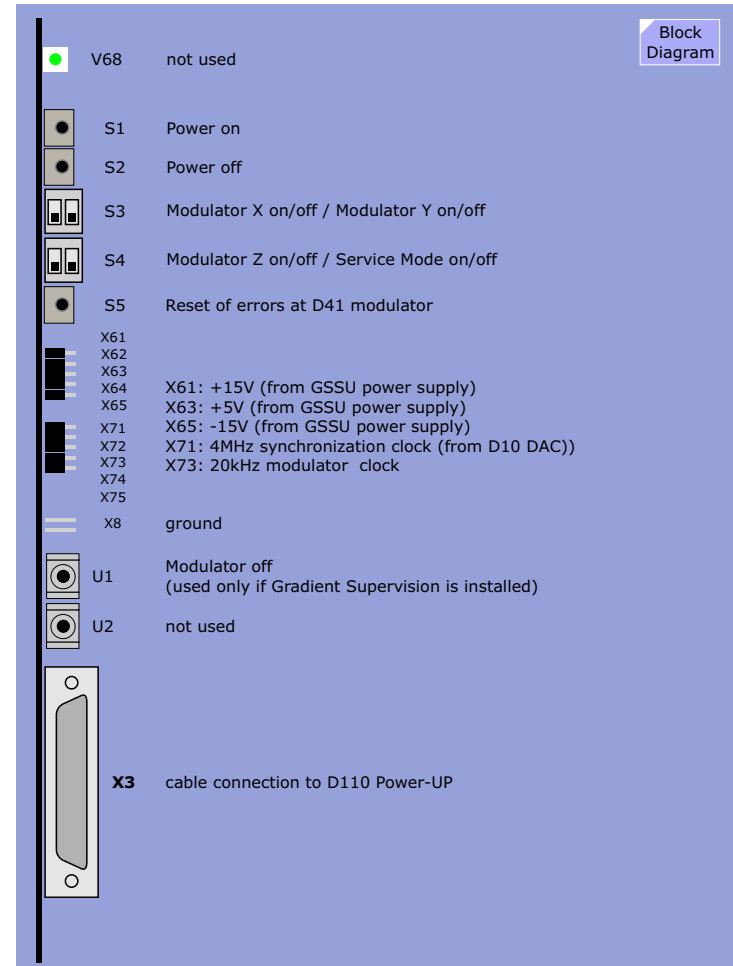
Figure 168 D70 I/O Board Layout
