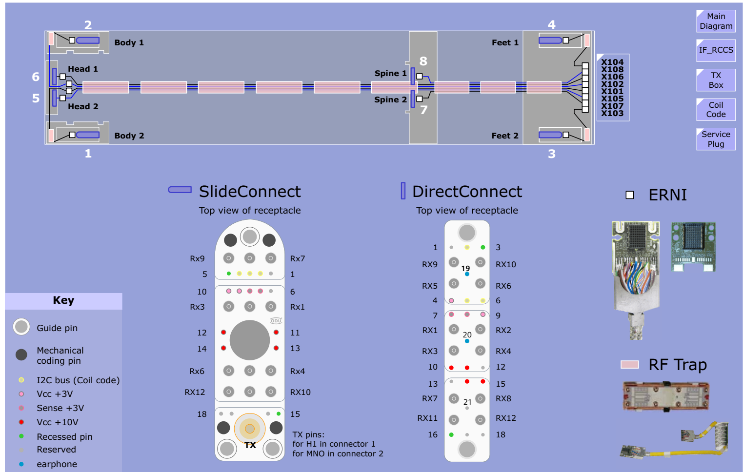
Figure 84 Coil Connectors and PTab Cable Inter-connections
