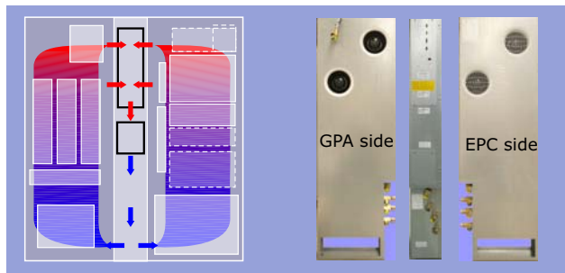
Figure 213 Cabinet Cooling Circulation
