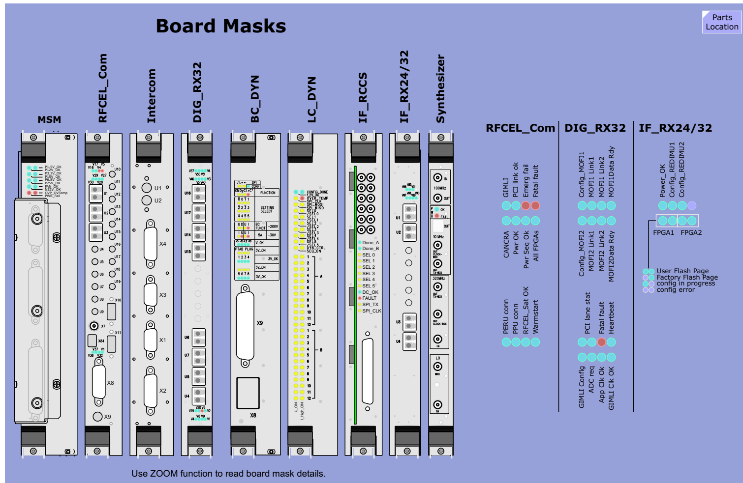
Figure 52 RFCEL Board Masks and LEDs
