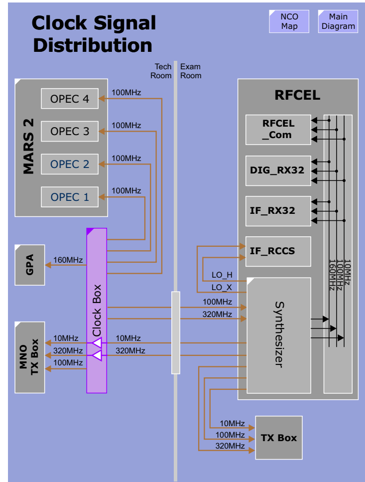
Figure 40 Clock Signal Distribution
