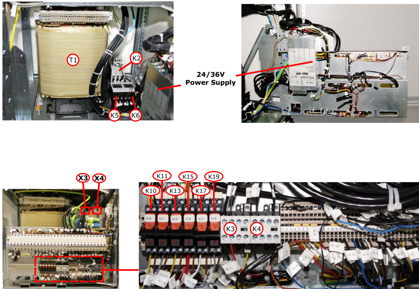
Figure 226 Line Power Distributor Parts Location
