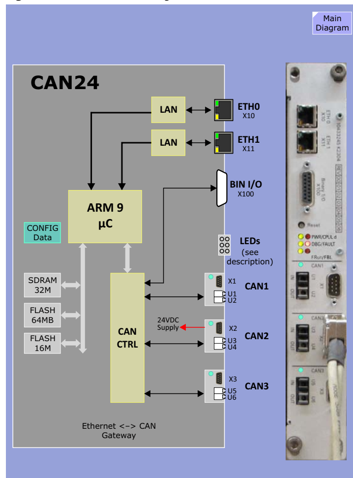
Figure 38 CAN24 Block Diagram
