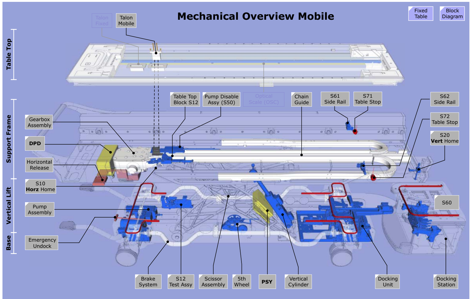
Figure 108 Tim Dockable Table Parts Location
