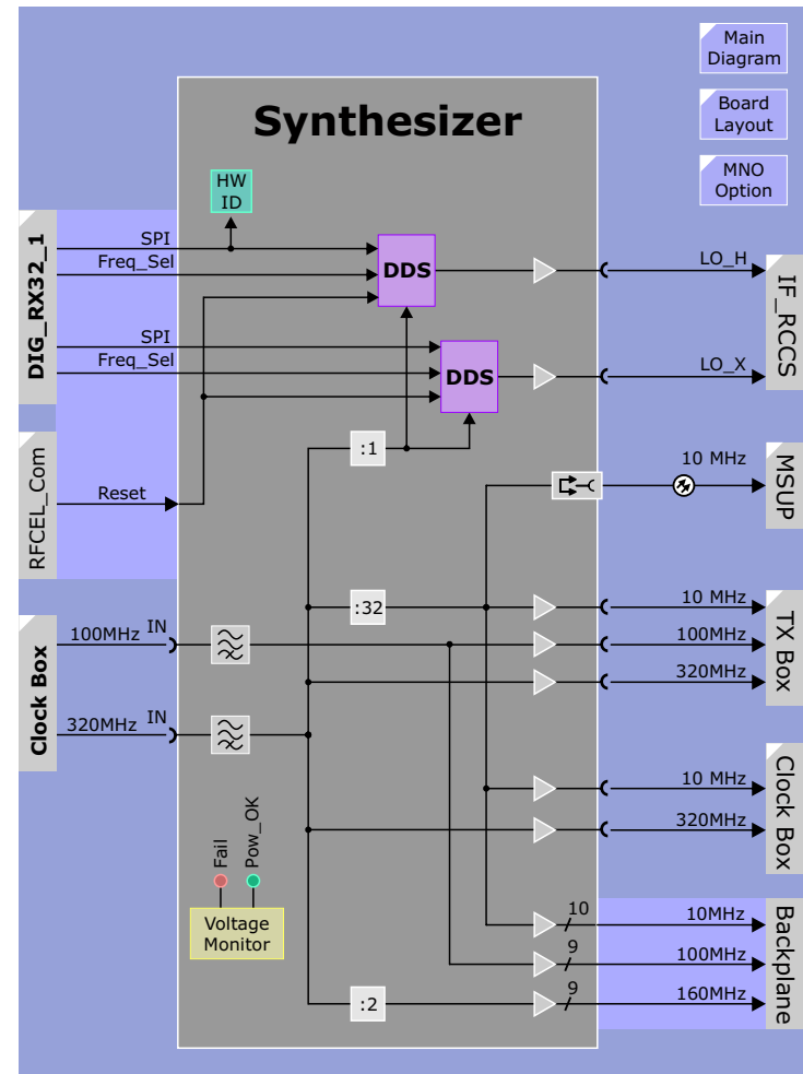
Figure 73 Synthesizer Block Diagram
