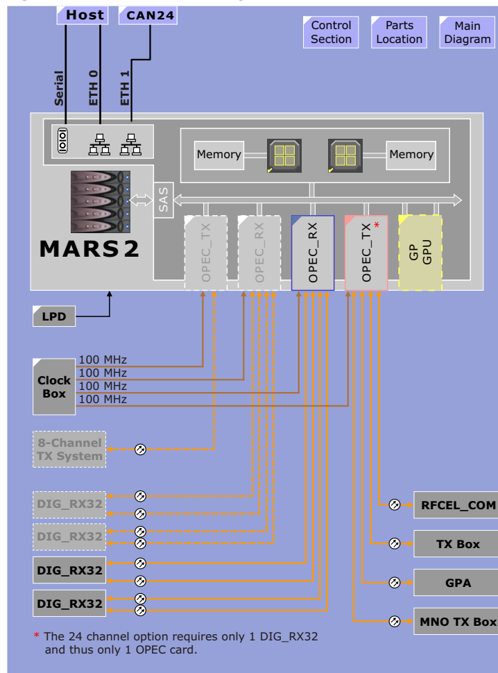
Figure 29 MARS 2 Block Diagram
