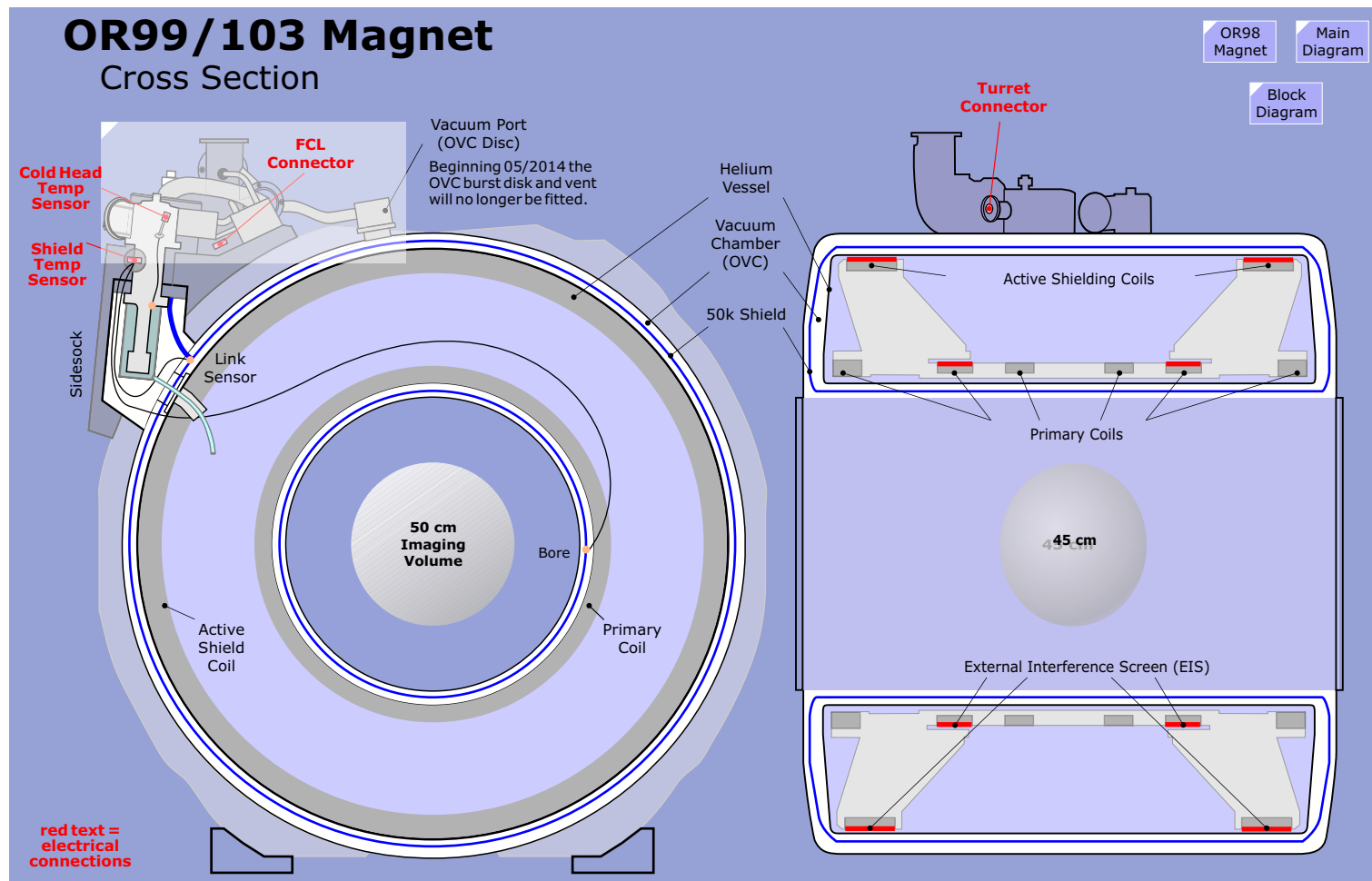
Figure 191 OR99/103 Magnet - Cross Sectional Diagram
