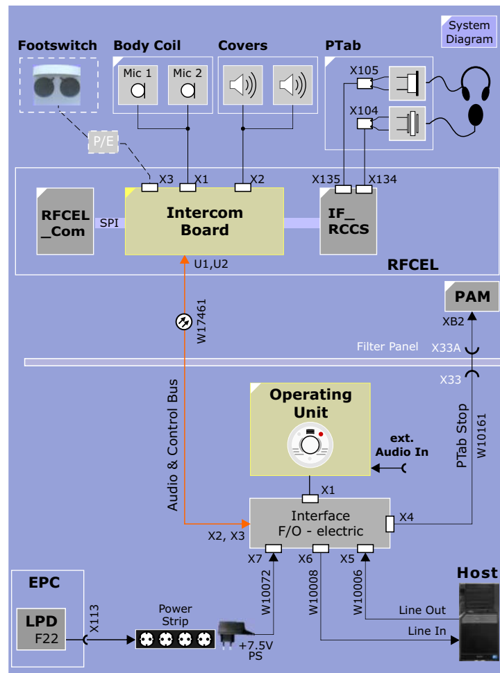
Figure 135 Intercom Block Diagram
