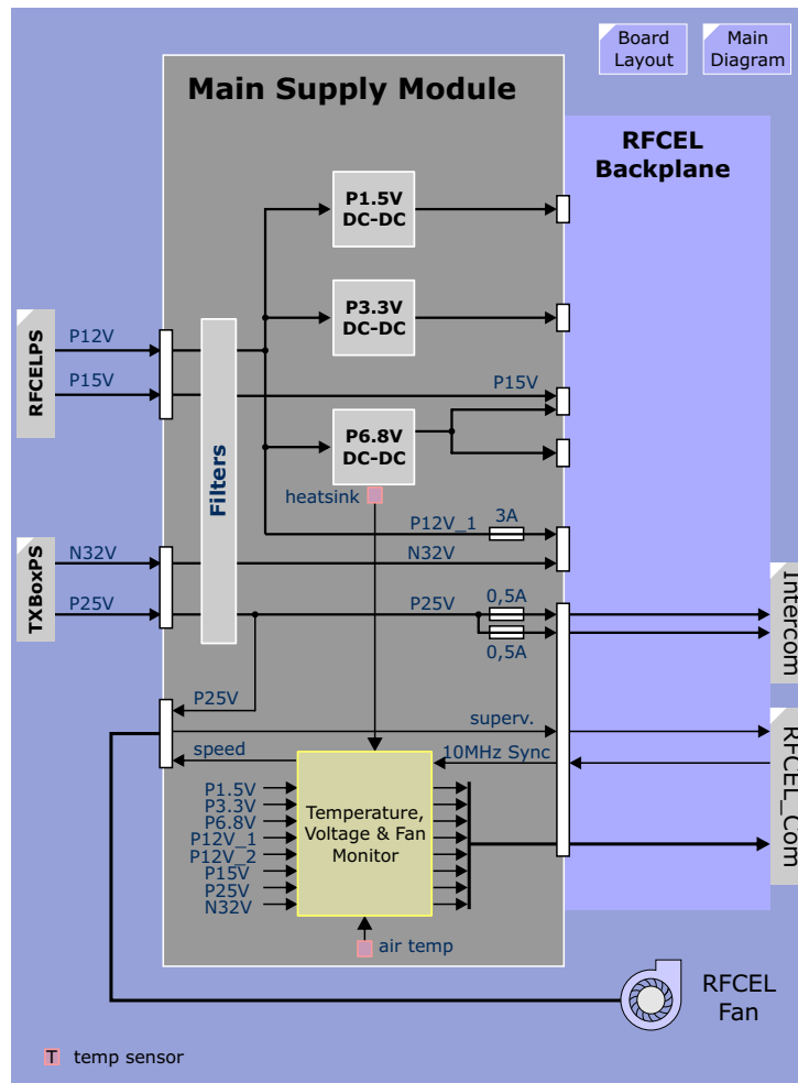
Figure 72 Main Supply Module Block Diagram
