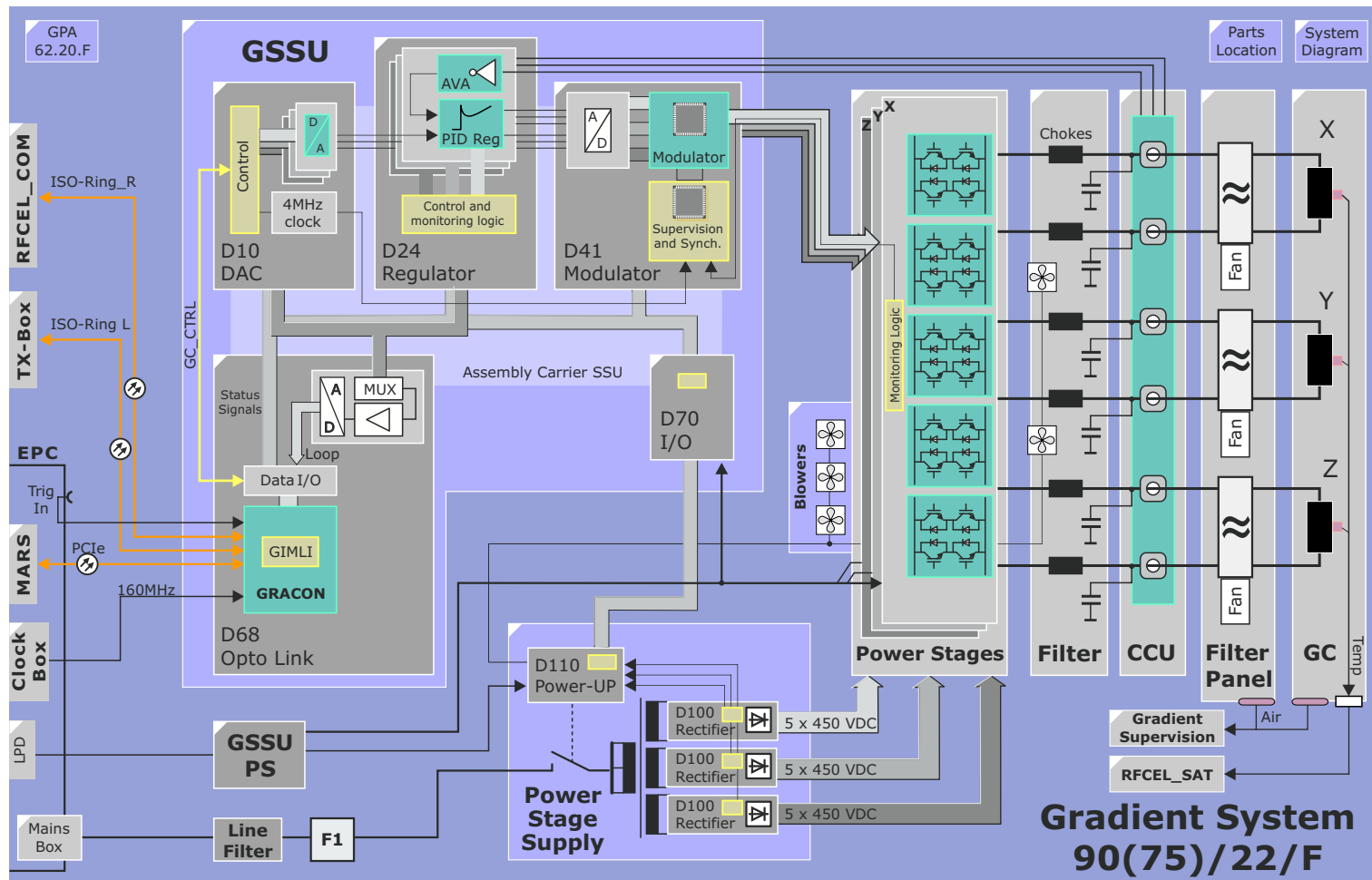
Figure 146 GPA 90(75)/22/F Block Diagram
