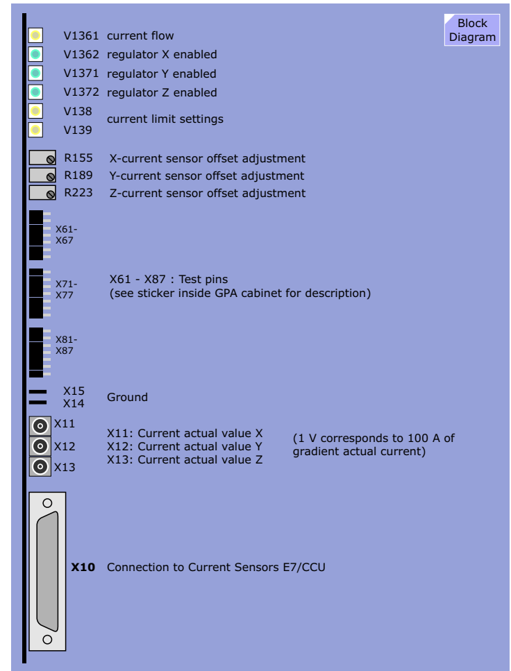
Figure 155 D24 Board Layout
