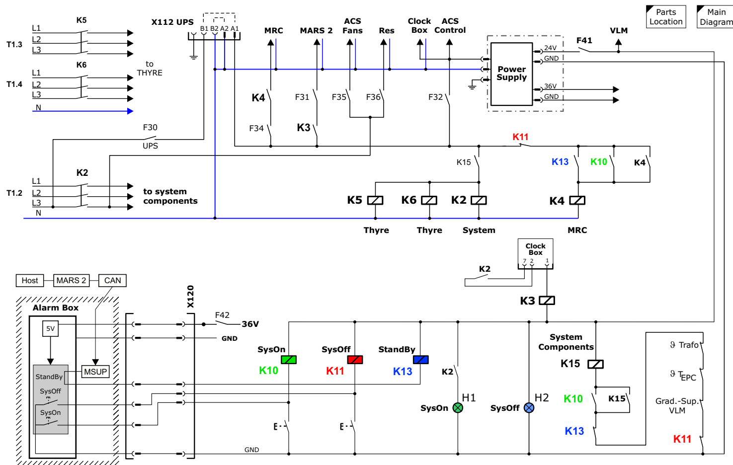
Figure 225 System Power On/Off Switch Logic
