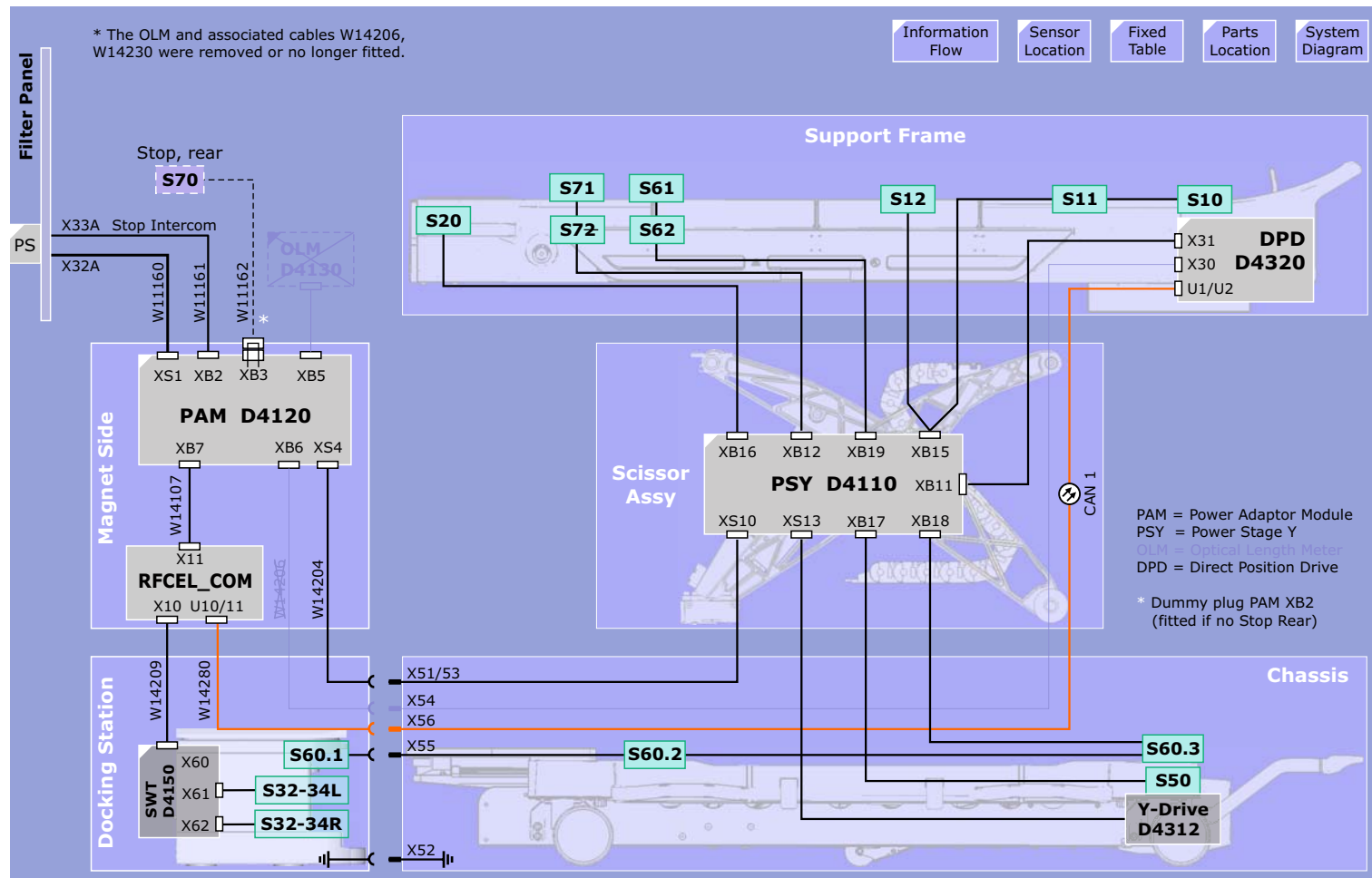
Figure 107 Tim Dockable Table Electrical Diagram
