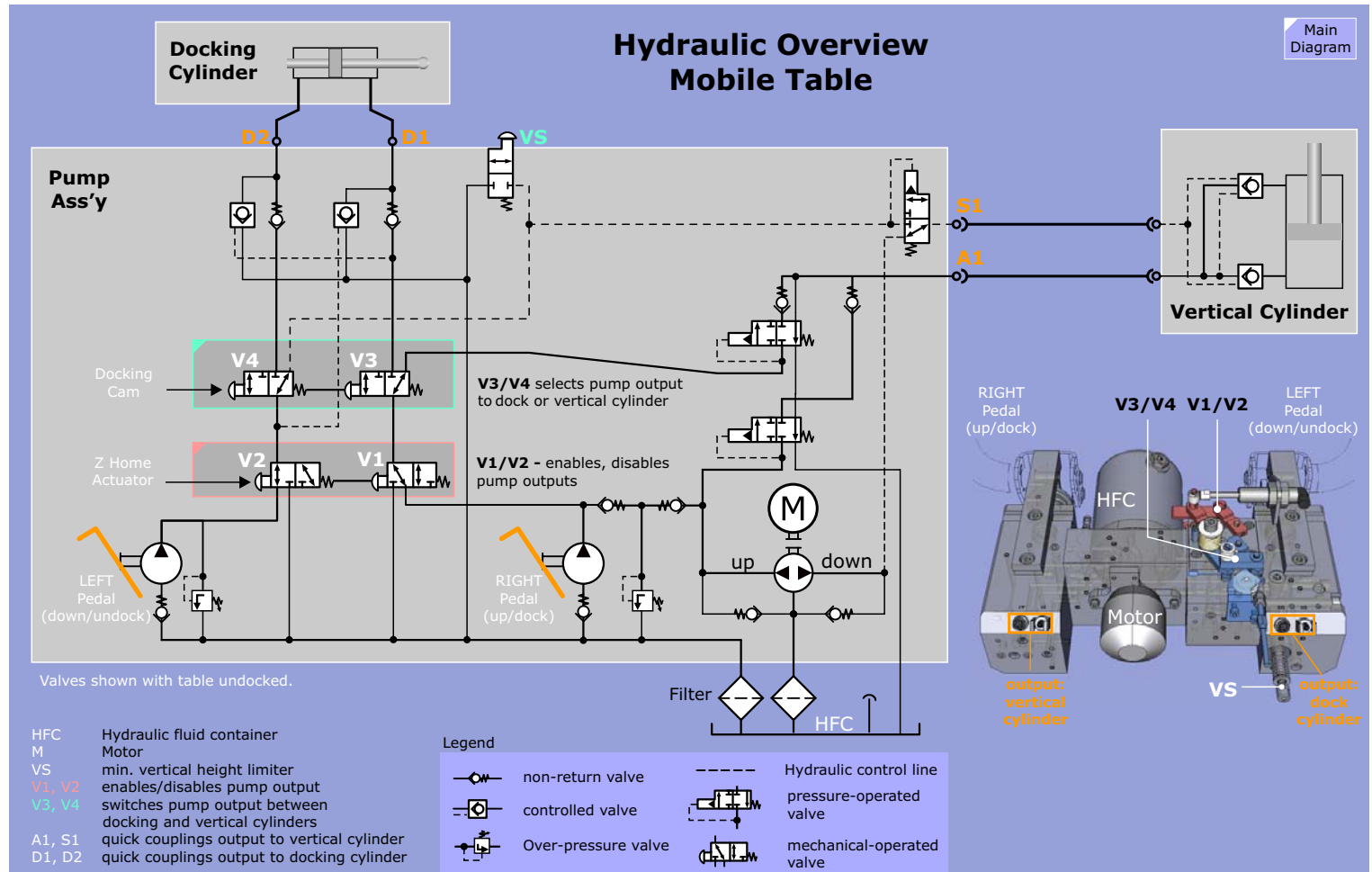
Figure 111 Hydraulic Overview - Mobile Table
