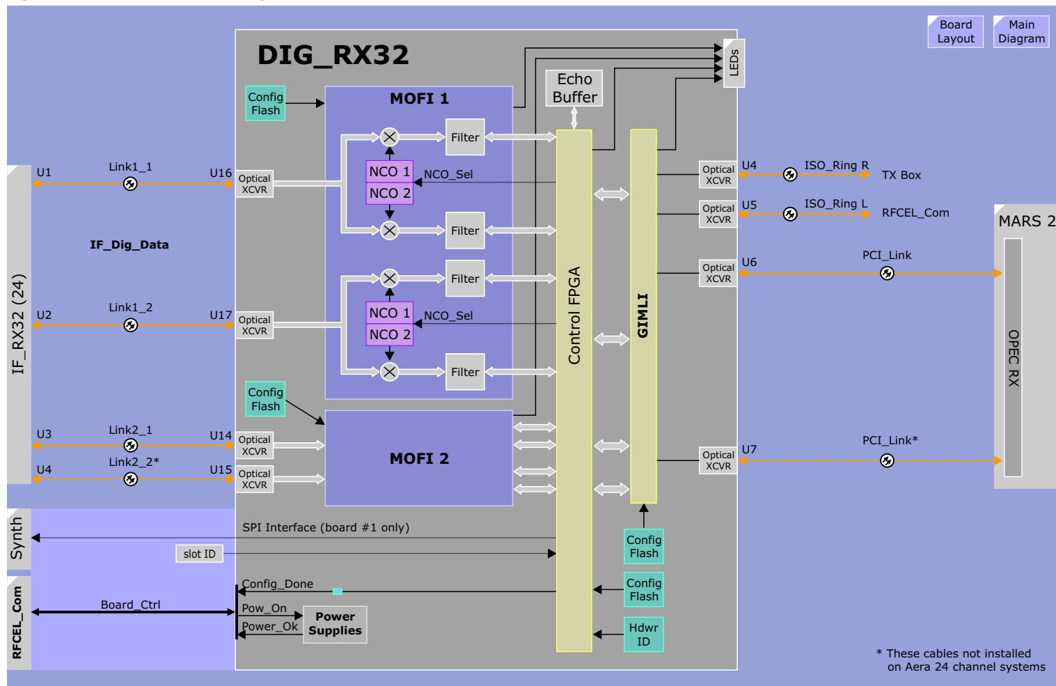
Figure 62 DIG_RX32 Block Diagram
