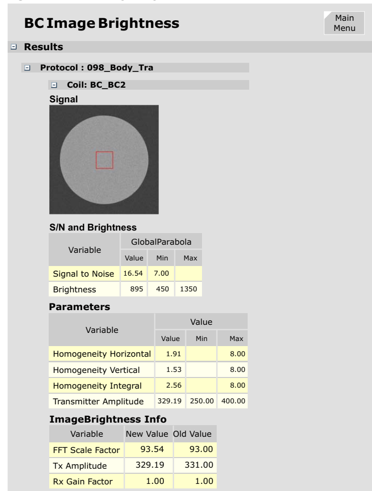
Figure 242 BC Image Brightness
