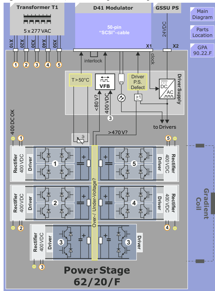
Figure 170 62/20/F Power Stage Block Diagram
