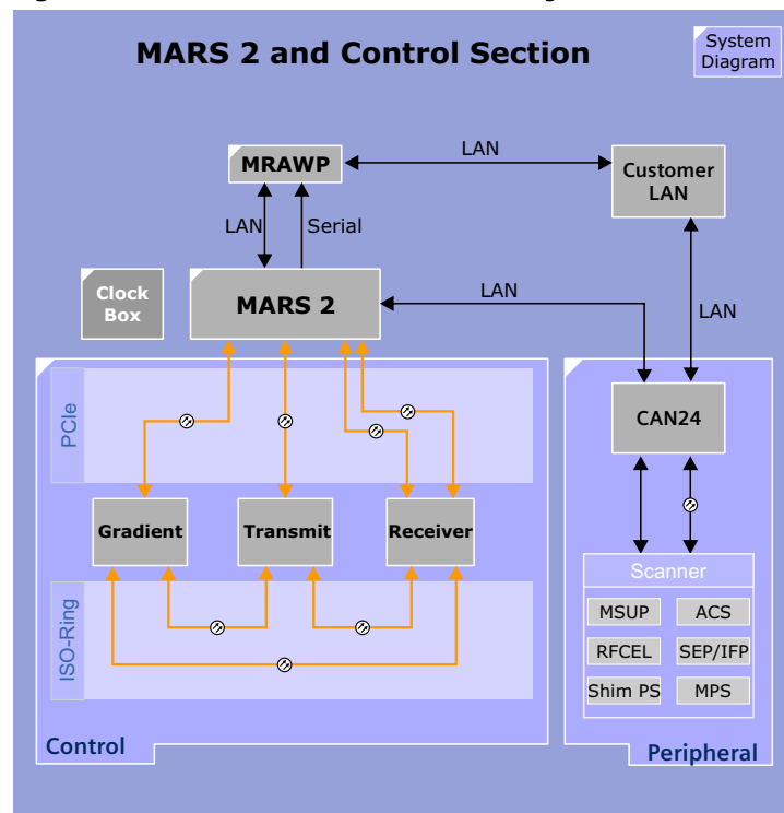
Figure 26 MARS and Control Overview Diagram
