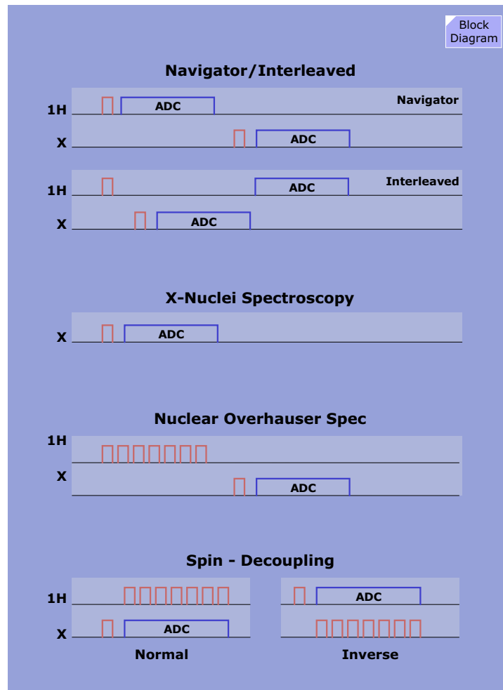
Figure 85 Supported Spectroscopy Measurements
