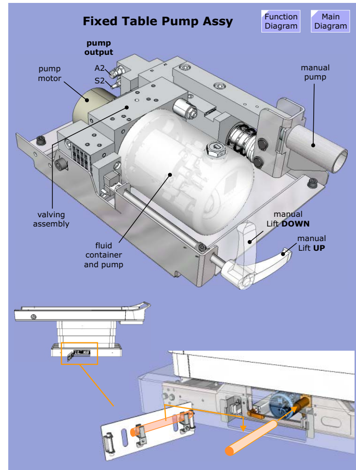
Figure 96 Hydraulic Pump Assembly
