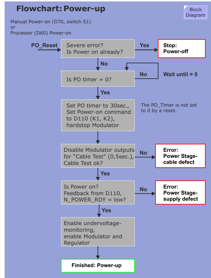
Figure 160 GPA Power Up Chart
