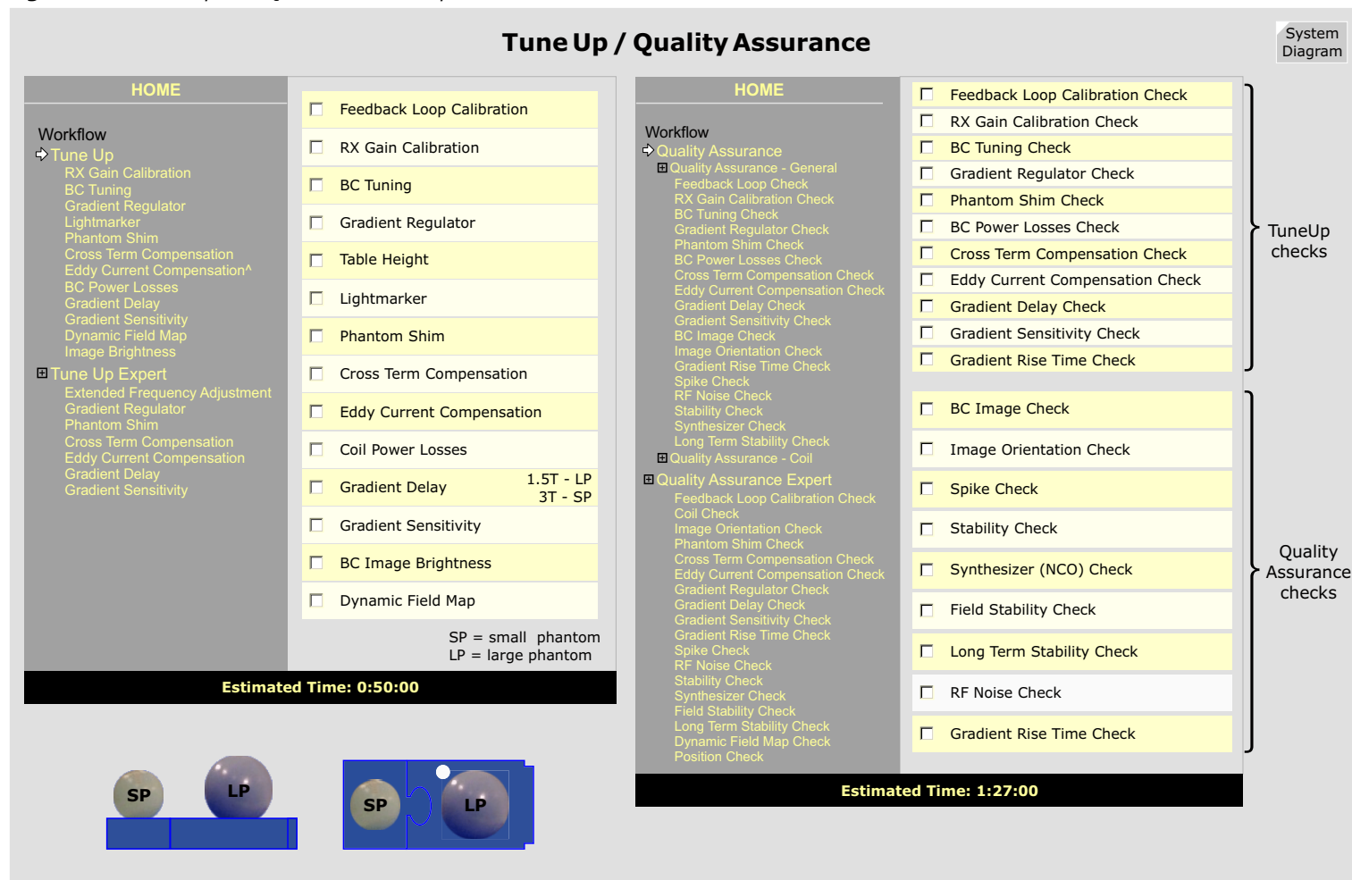
Figure 229 Tune Up and QA Procedural Steps
