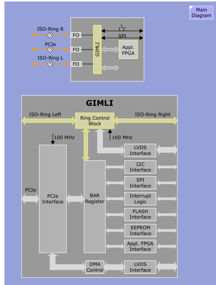
Figure 34 GIMLI Overview
