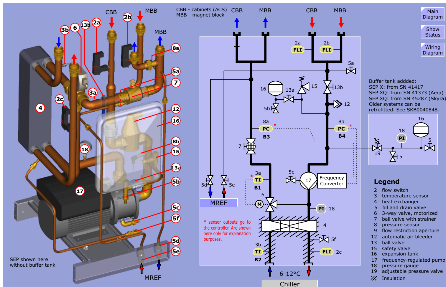
Figure 216 SEP Plumbing
