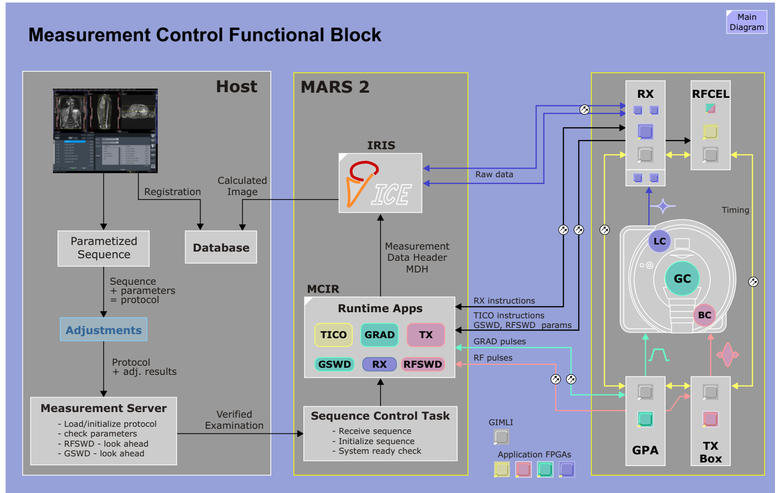
Figure 27 MARS 2 and Control Functional Overview
