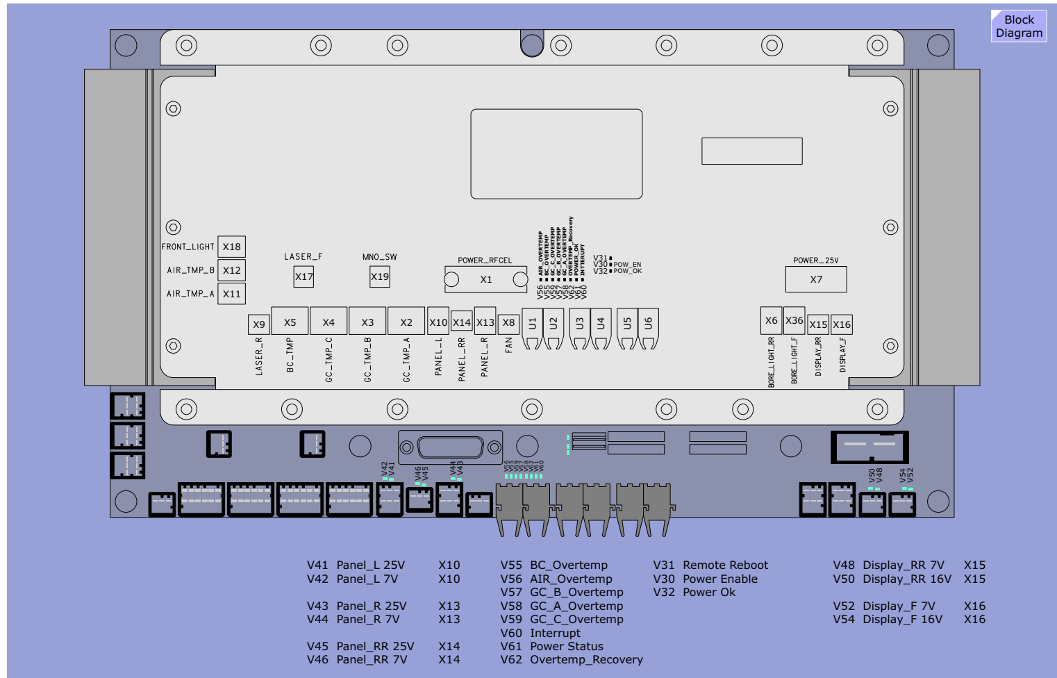
Figure 129 RFCEL_Sat Layout
