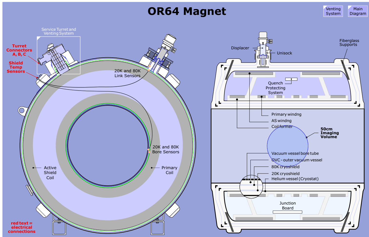
Figure 262 OR64 Magnet
