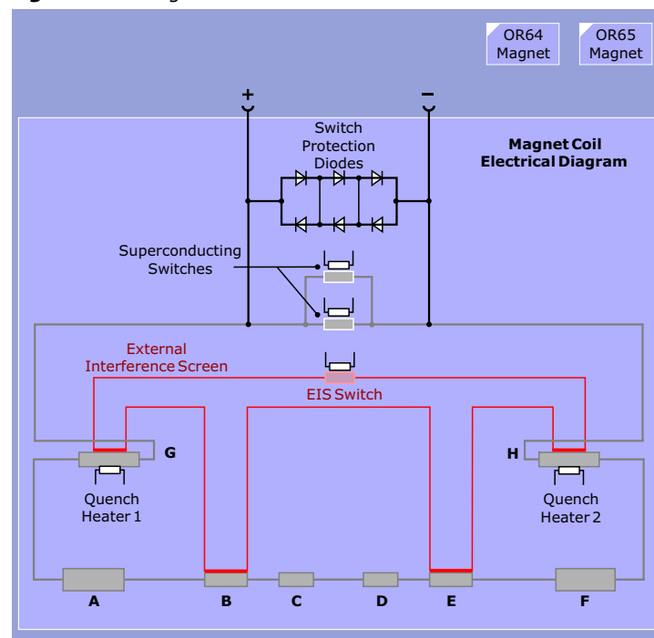
Figure 261 Magnet Schematic
