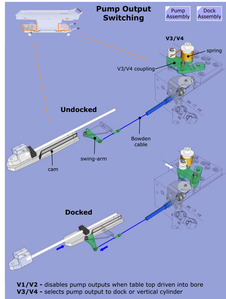
Figure 113 Switching Pump Output with V3/V4
