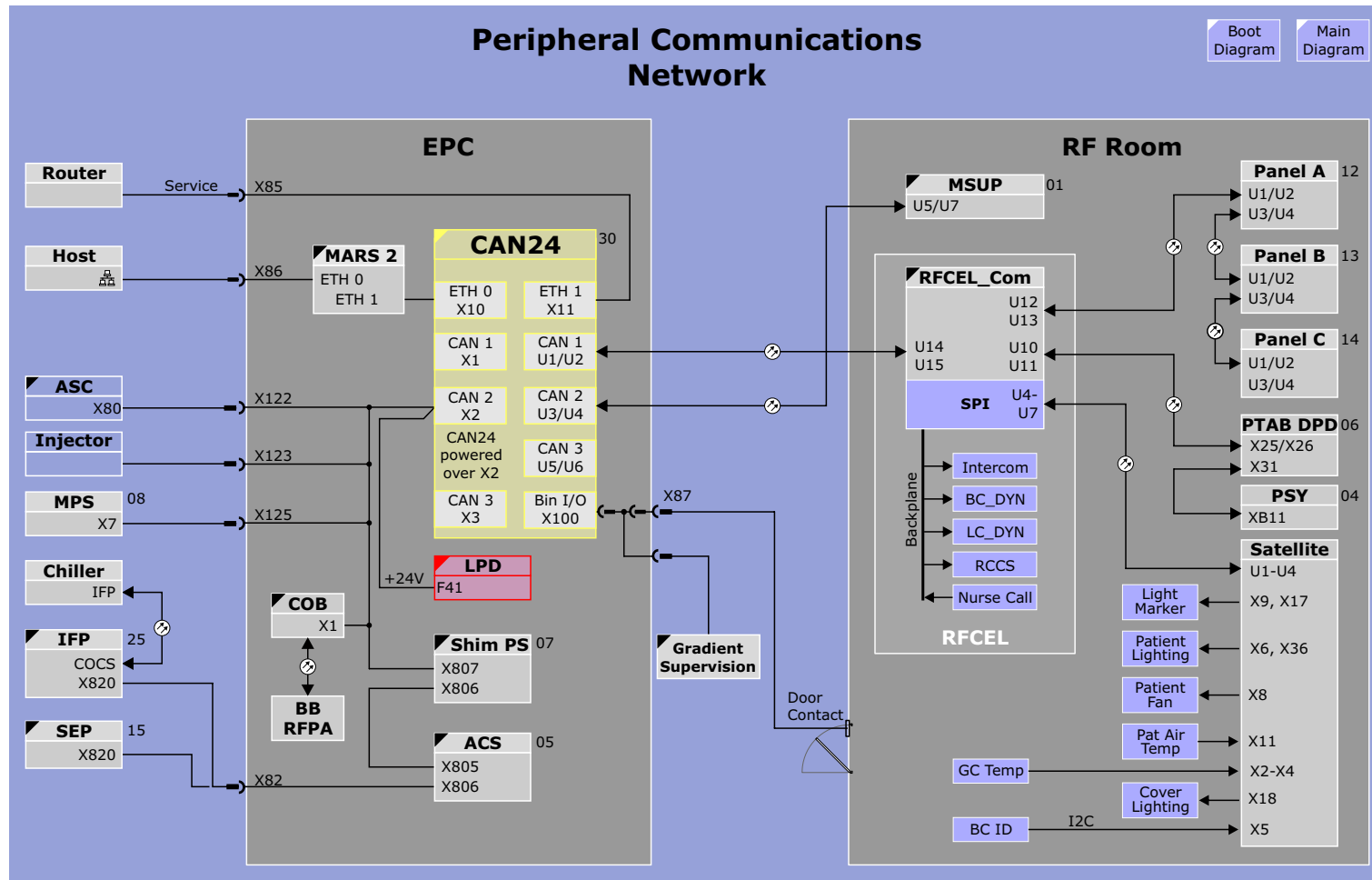
Figure 37 Peripheral Communications Network
