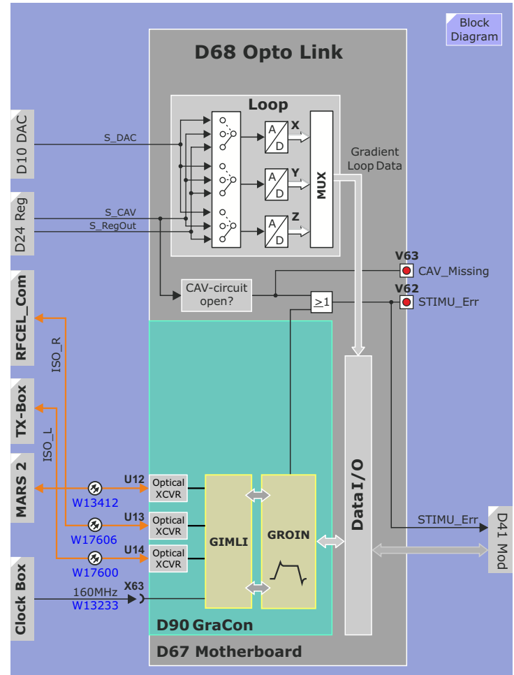
Figure 165 D68 Opto Link - Loop Back
