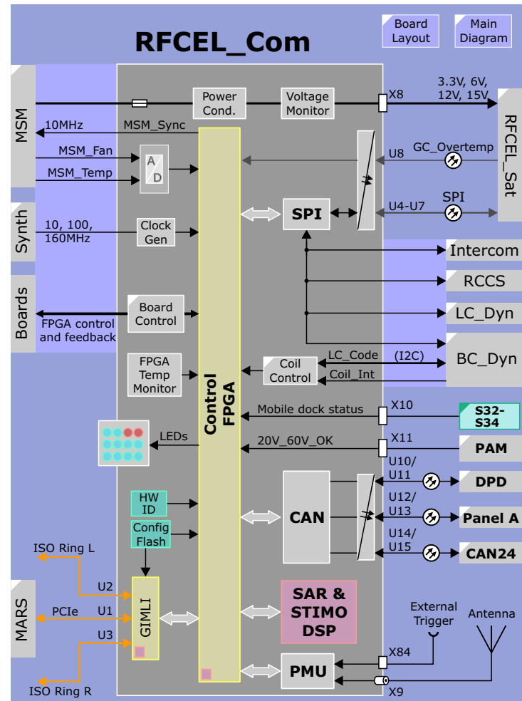
Figure 68 RFCEL_Com Block Diagram
