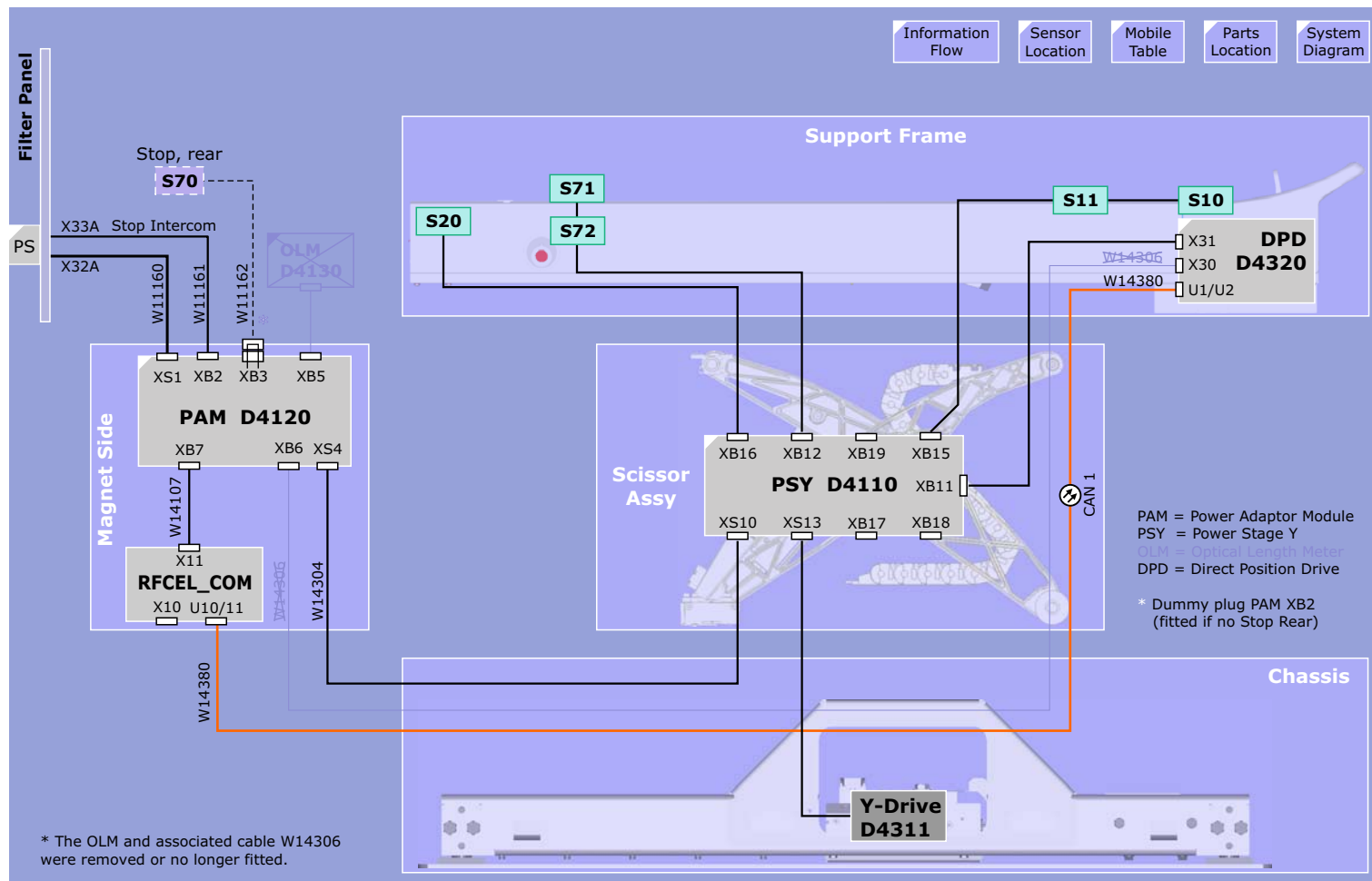
Figure 93 Tim Table Block Diagram
