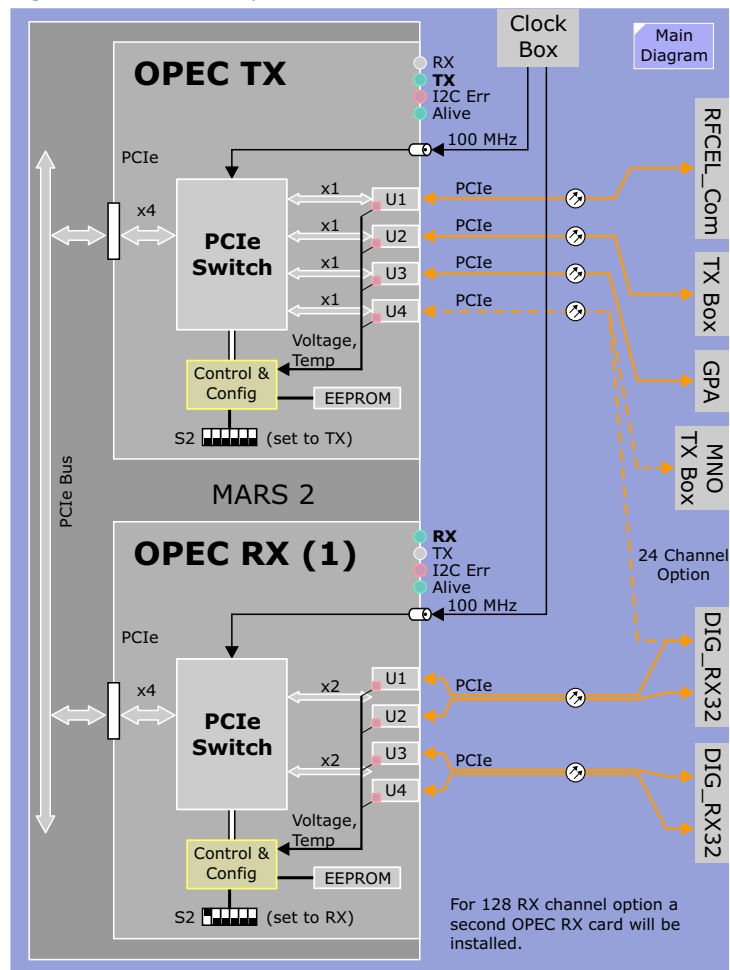
Figure 30 OPEC - Optical PCIe Card
